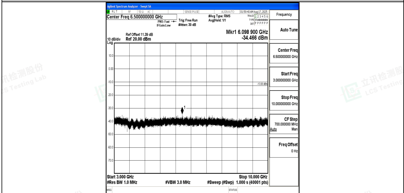
Band12_5MHz_16QAM_23095_1RB#0_3000~10000_3000~10000
