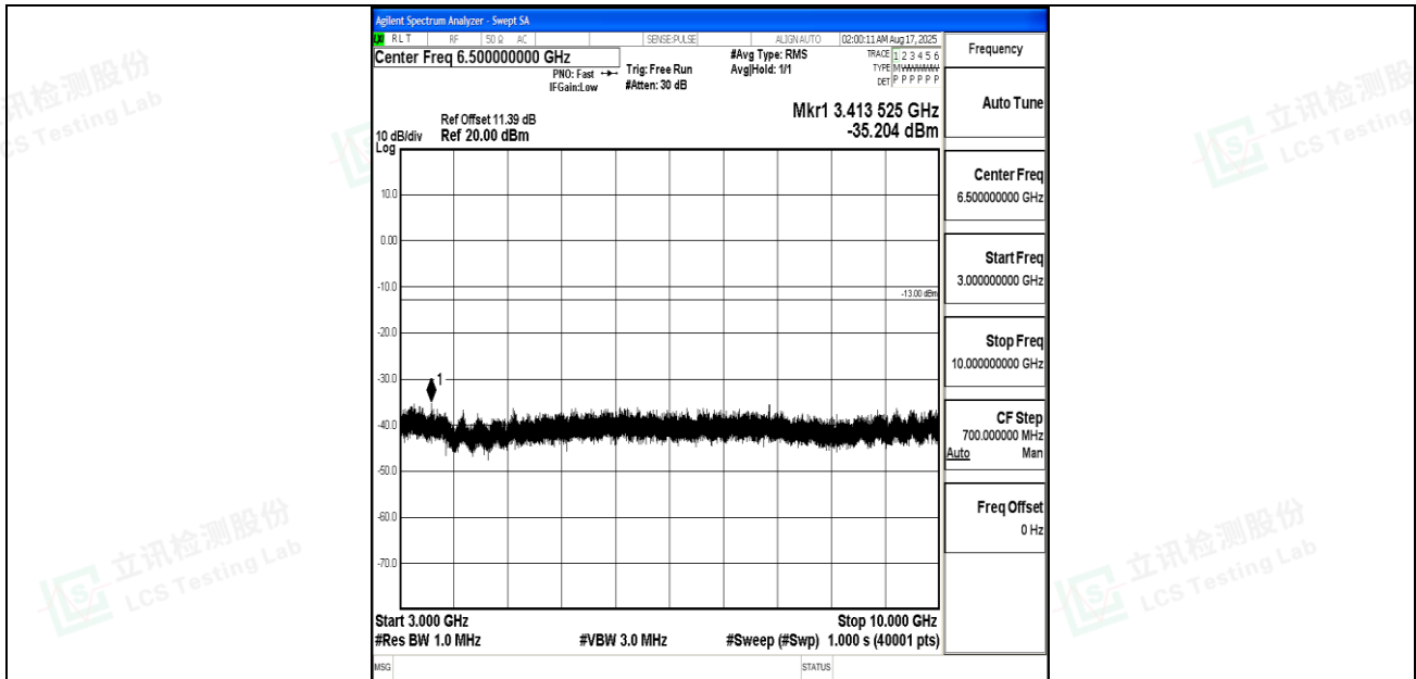
Band12_5MHz_QPSK_23155_1RB#0_3000~10000_3000~10000
