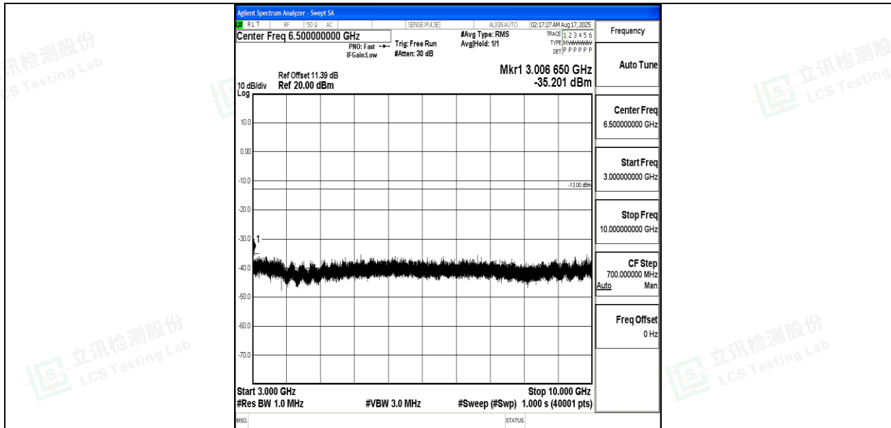
Band12_10MHz_QPSK_23095_1RB#0_3000~10000_3000~10000
