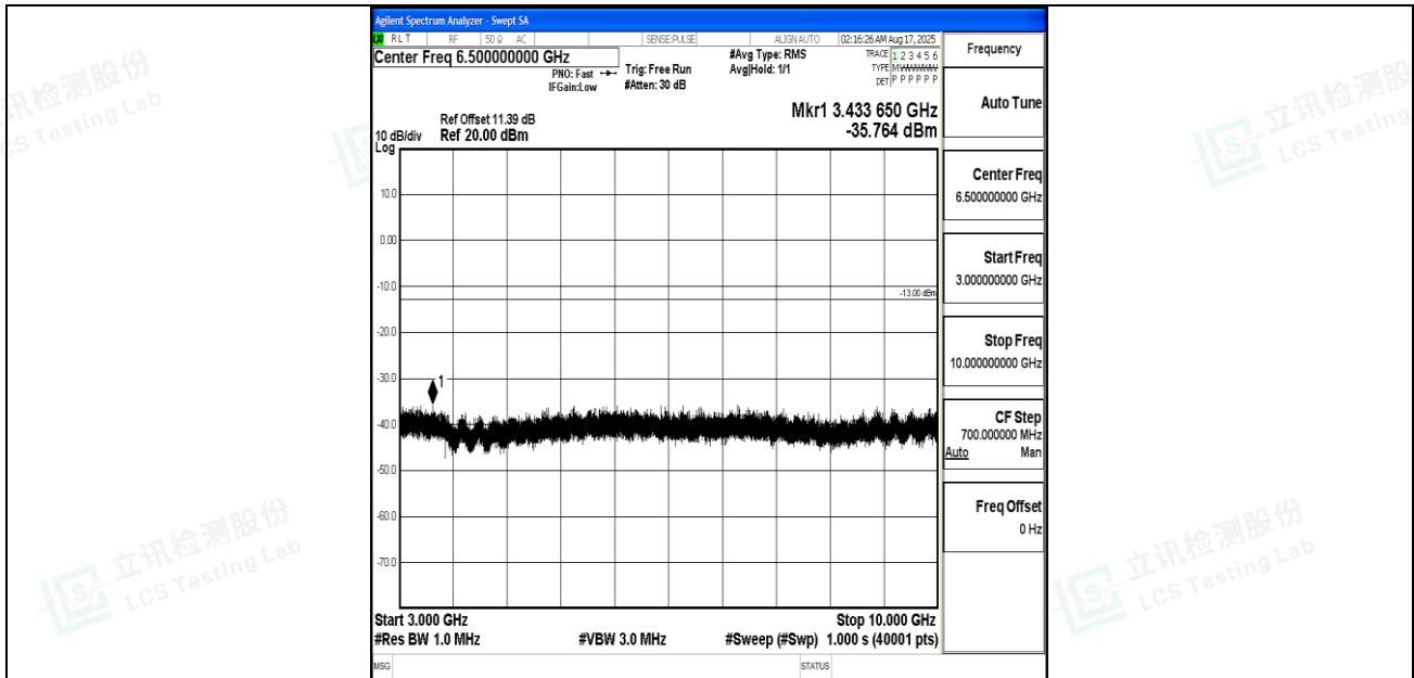
Band12_10MHz_QPSK_23060_1RB#0_3000~10000_3000~10000
