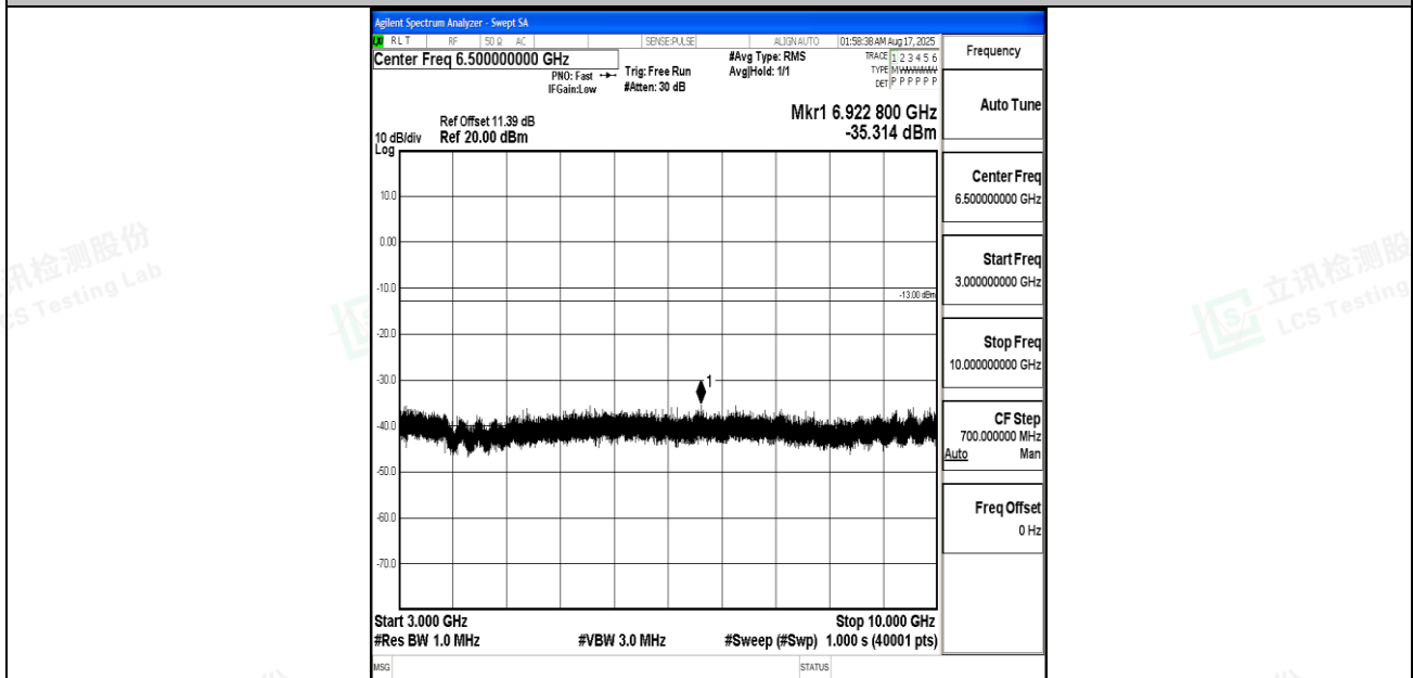
Band12_5MHz_16QAM_23035_1RB#0_3000~10000_3000~10000
