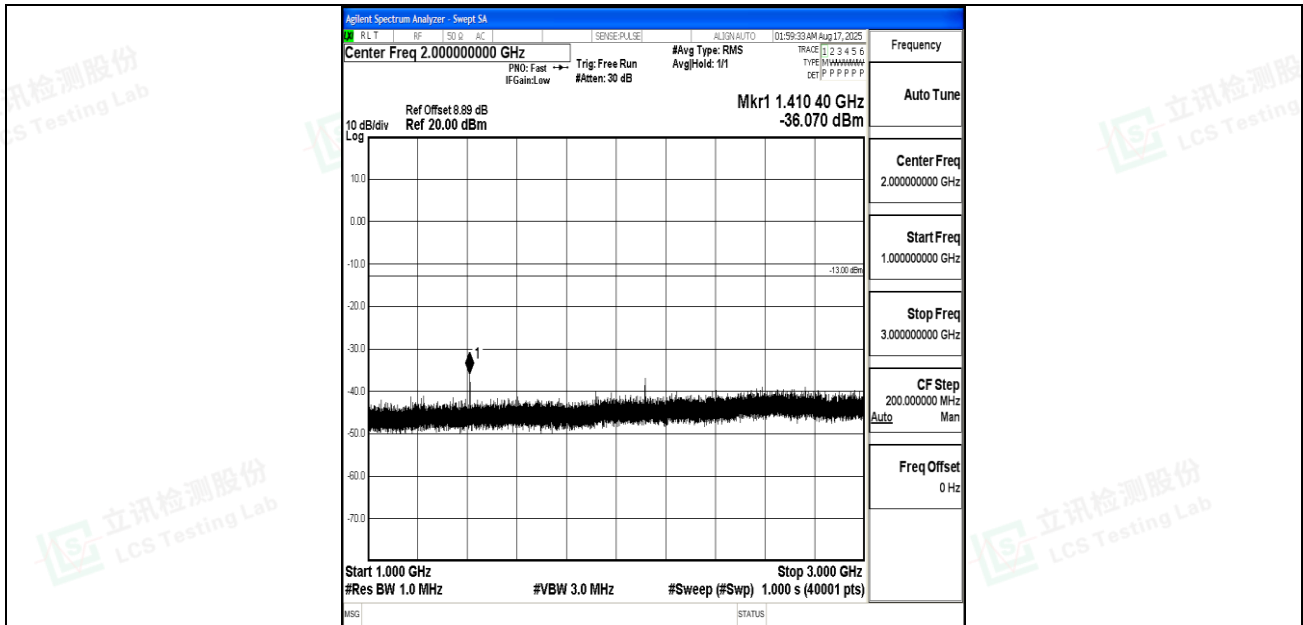
Band12_5MHz_16QAM_23095_1RB#0_1000~3000_1000~3000
