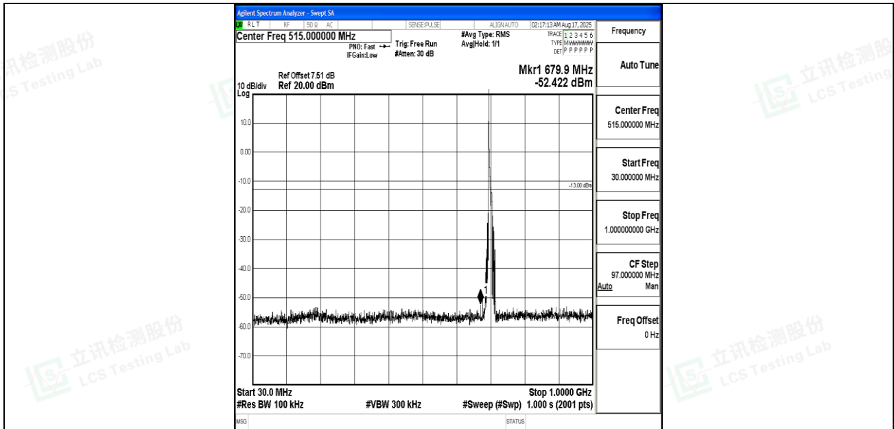
Band12_10MHz_QPSK_23095_1RB#0_30~1000_30~1000
