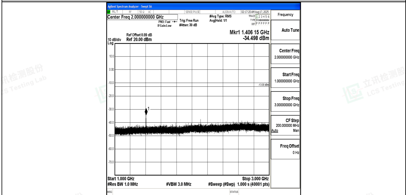
Band12_10MHz_QPSK_23095_1RB#0_1000~3000_1000~3000
