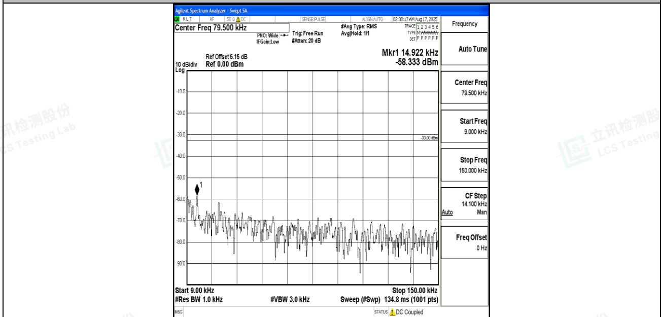
Band12_5MHz_16QAM_23155_1RB#0_0.009~0.15_0.009~0.15
