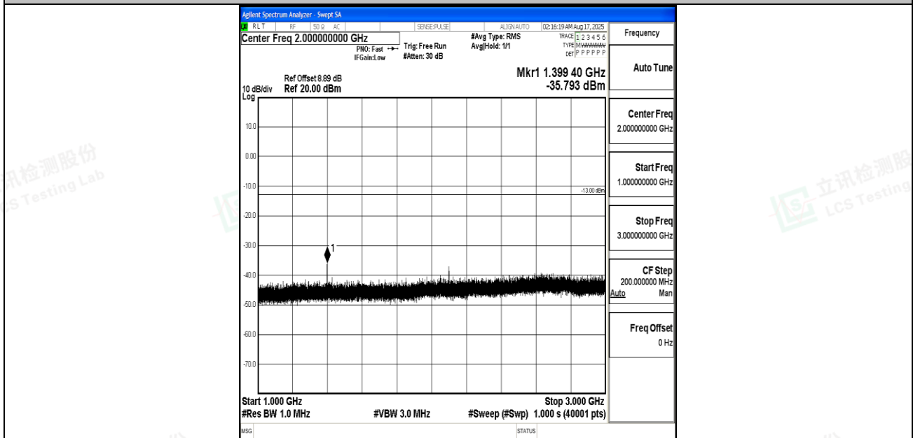
Band12_10MHz_QPSK_23060_1RB#0_1000~3000_1000~3000
