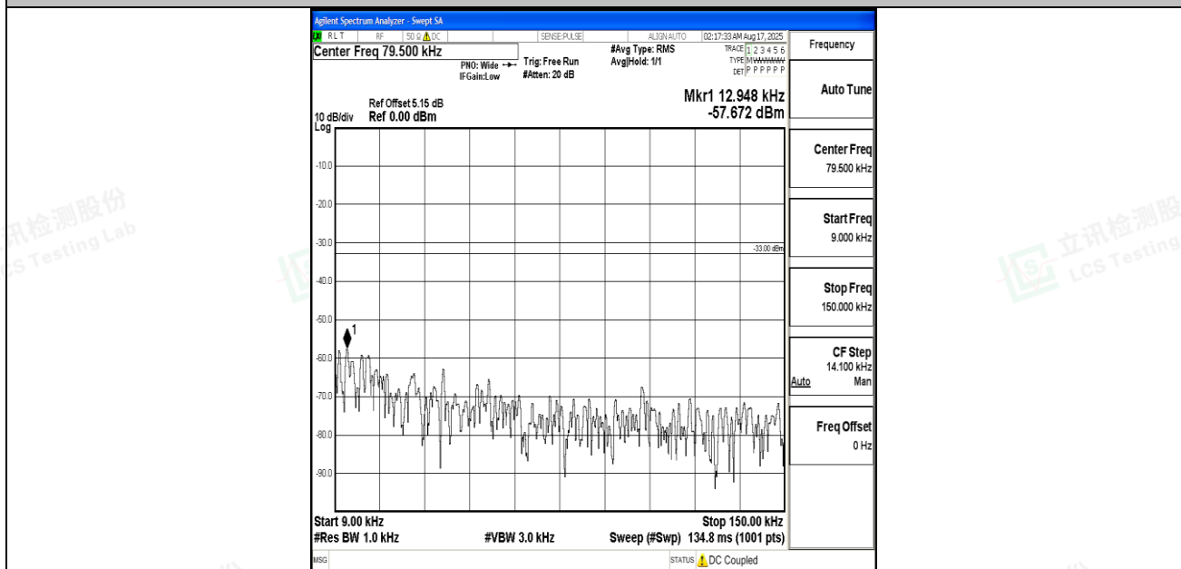
Band12_10MHz_16QAM_23095_1RB#0_0.009~0.15_0.009~0.15
