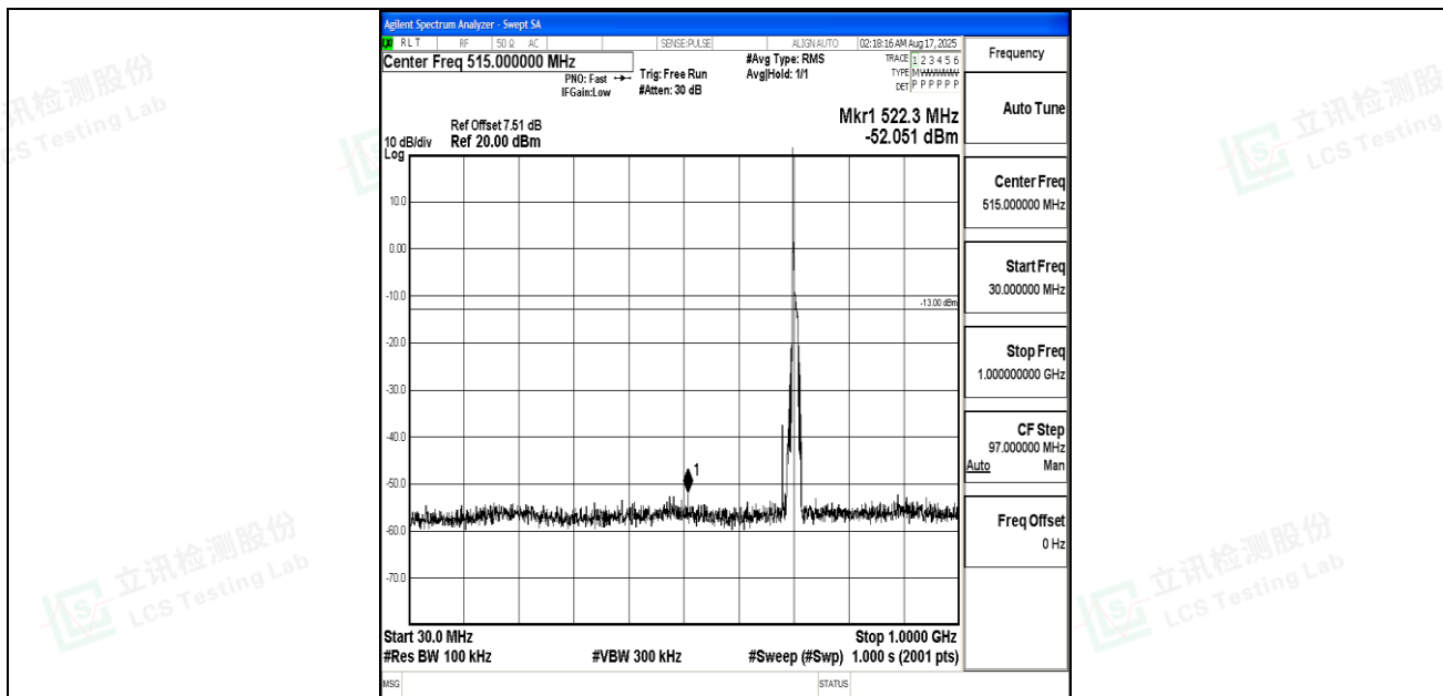
Band12_10MHz_QPSK_23130_1RB#0_30~1000_30~1000
