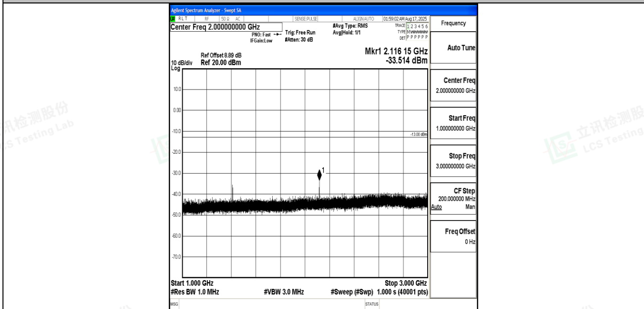
Band12_5MHz_QPSK_23095_1RB#0_1000~3000_1000~3000
