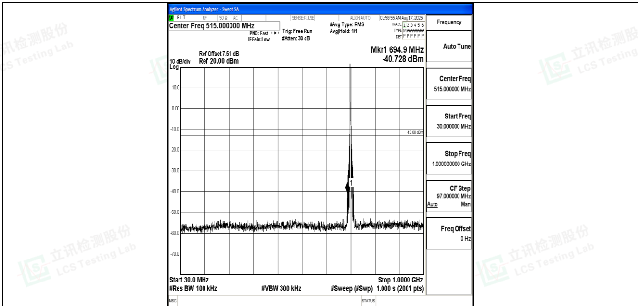
Band12_5MHz_QPSK_23095_1RB#0_30~1000_30~1000
