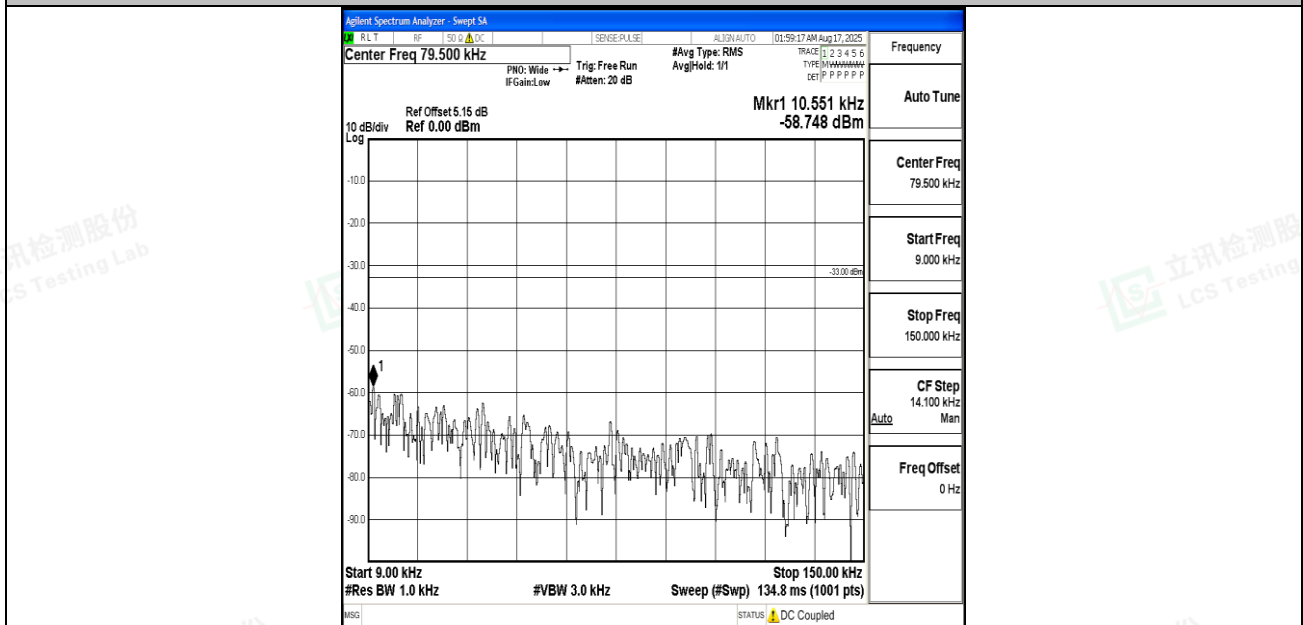
Band12_5MHz_16QAM_23095_1RB#0_0.009~0.15_0.009~0.15
