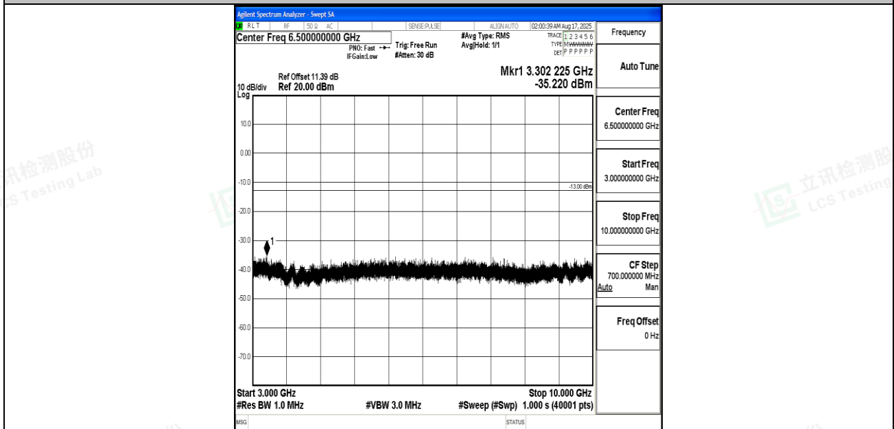
Band12_5MHz_16QAM_23155_1RB#0_3000~10000_3000~10000
