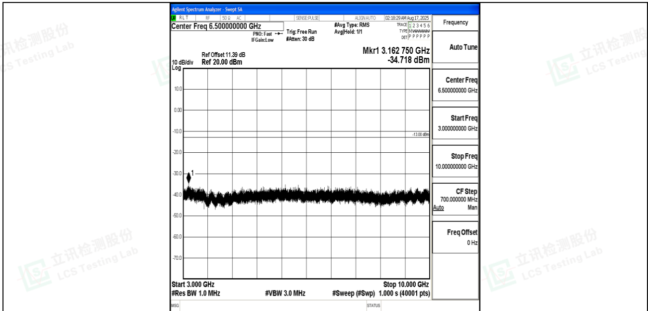
Band12_10MHz_QPSK_23130_1RB#0_3000~10000_3000~10000
