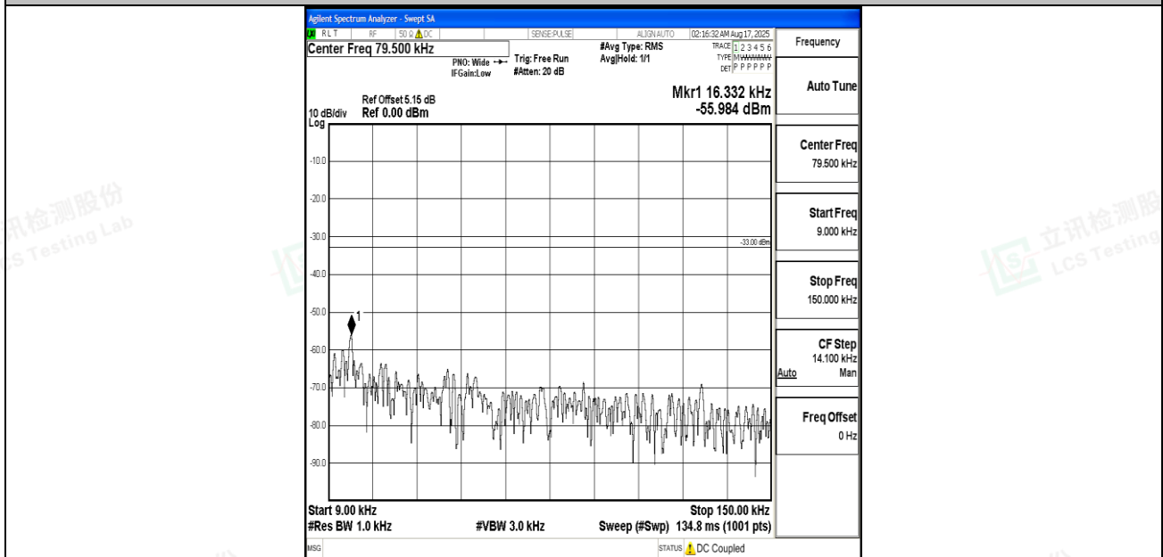
Band12_10MHz_16QAM_23060_1RB#0_0.009~0.15_0.009~0.15
