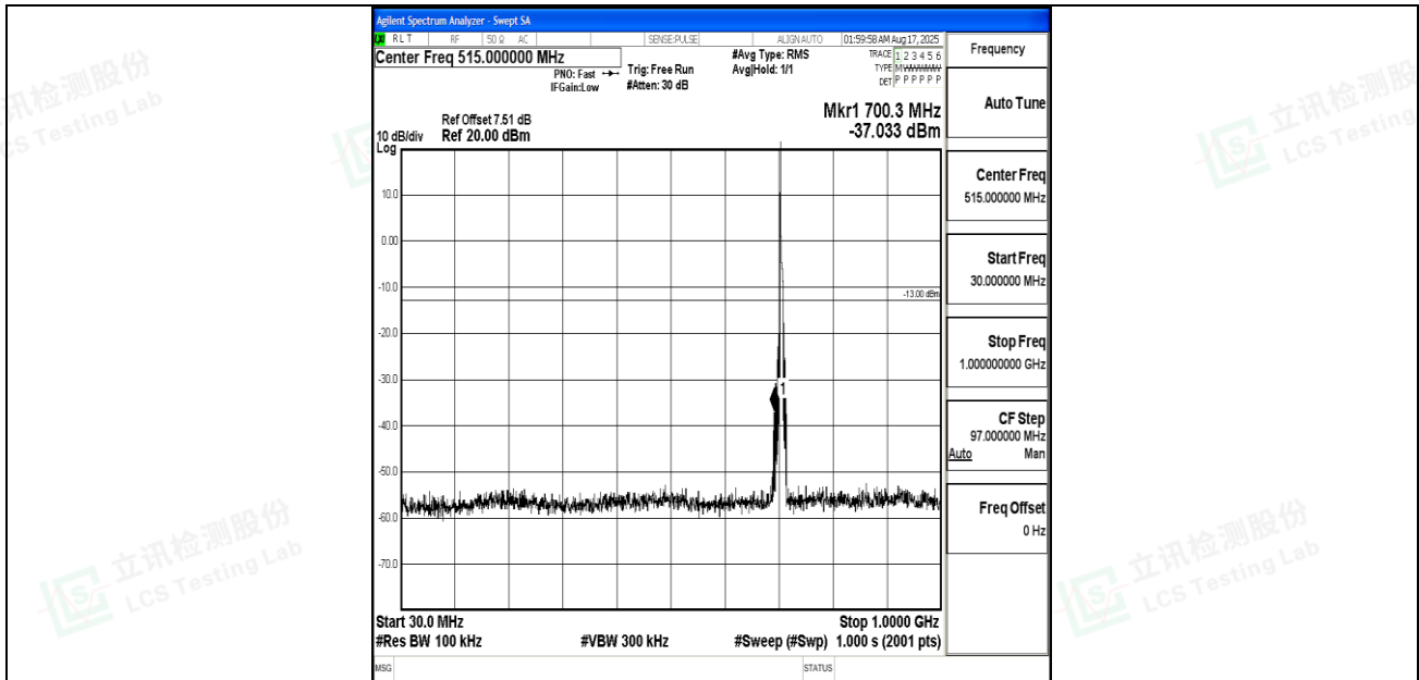
Band12_5MHz_QPSK_23155_1RB#0_30~1000_30~1000
