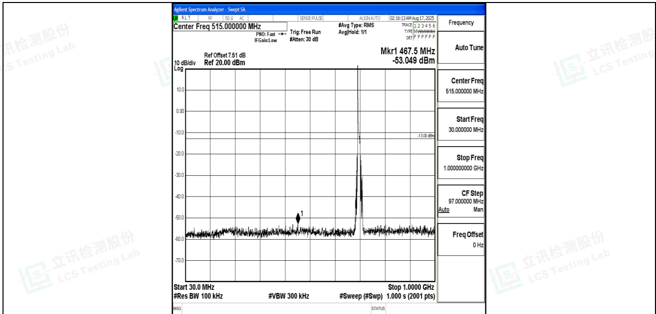
Band12_10MHz_QPSK_23060_1RB#0_30~1000_30~1000
