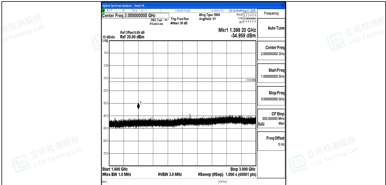
Band12_10MHz_16QAM_23060_1RB#0_1000~3000_1000~3000
