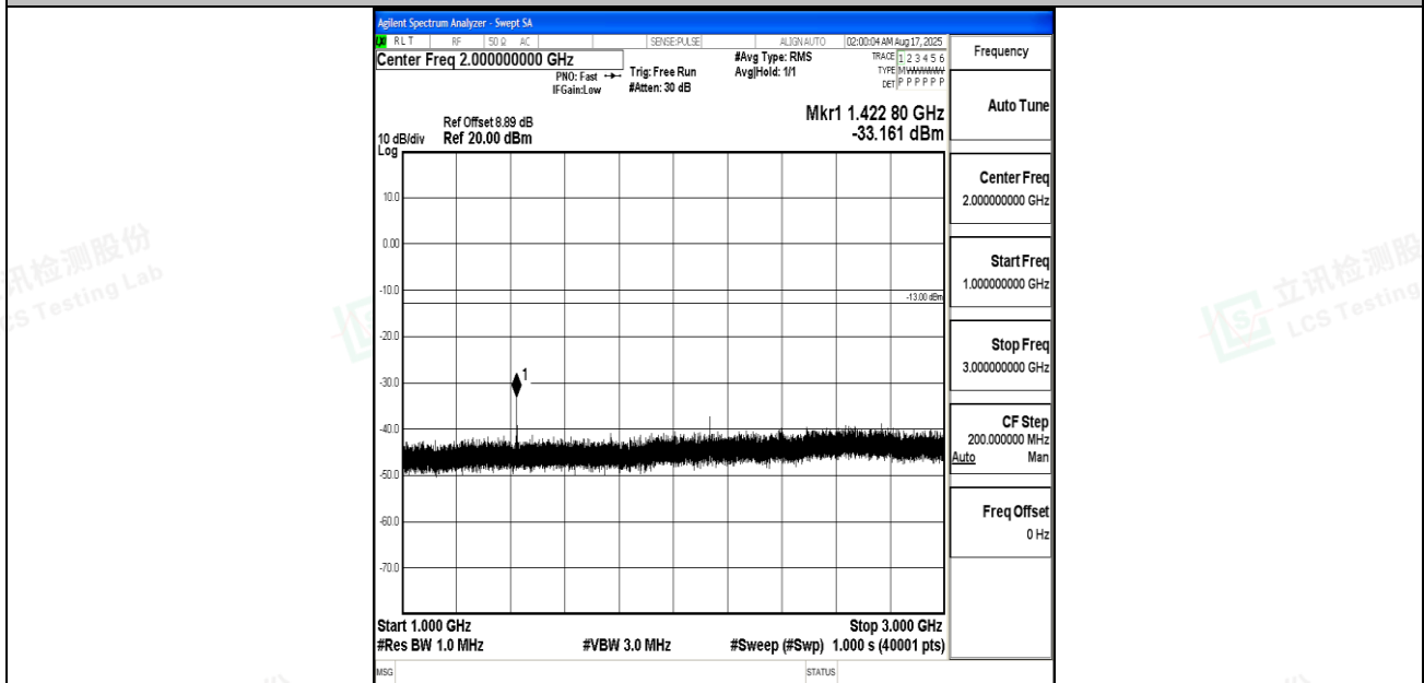
Band12_5MHz_QPSK_23155_1RB#0_1000~3000_1000~3000
