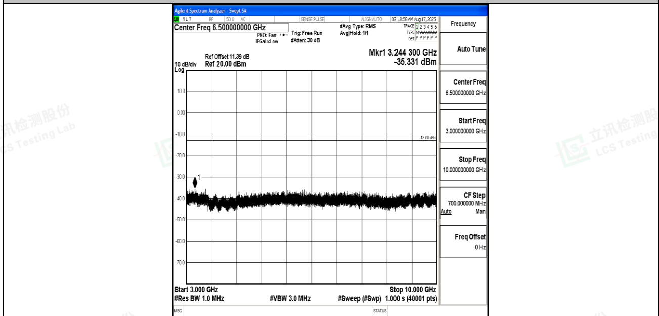
Band12_10MHz_16QAM_23130_1RB#0_3000~10000_3000~10000
