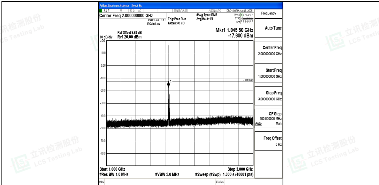
Band25_1.4MHz_QPSK_26047_1RB#0_1000~3000_1000~3000
