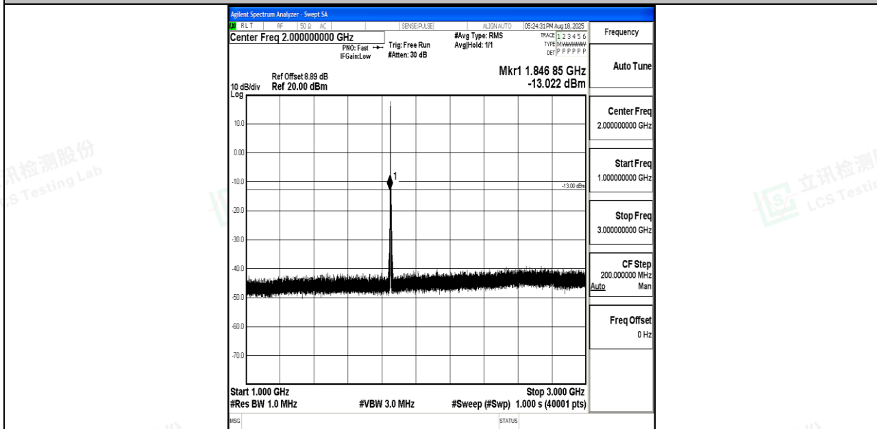
Band25_1.4MHz_16QAM_26047_1RB#0_1000~3000_1000~3000
