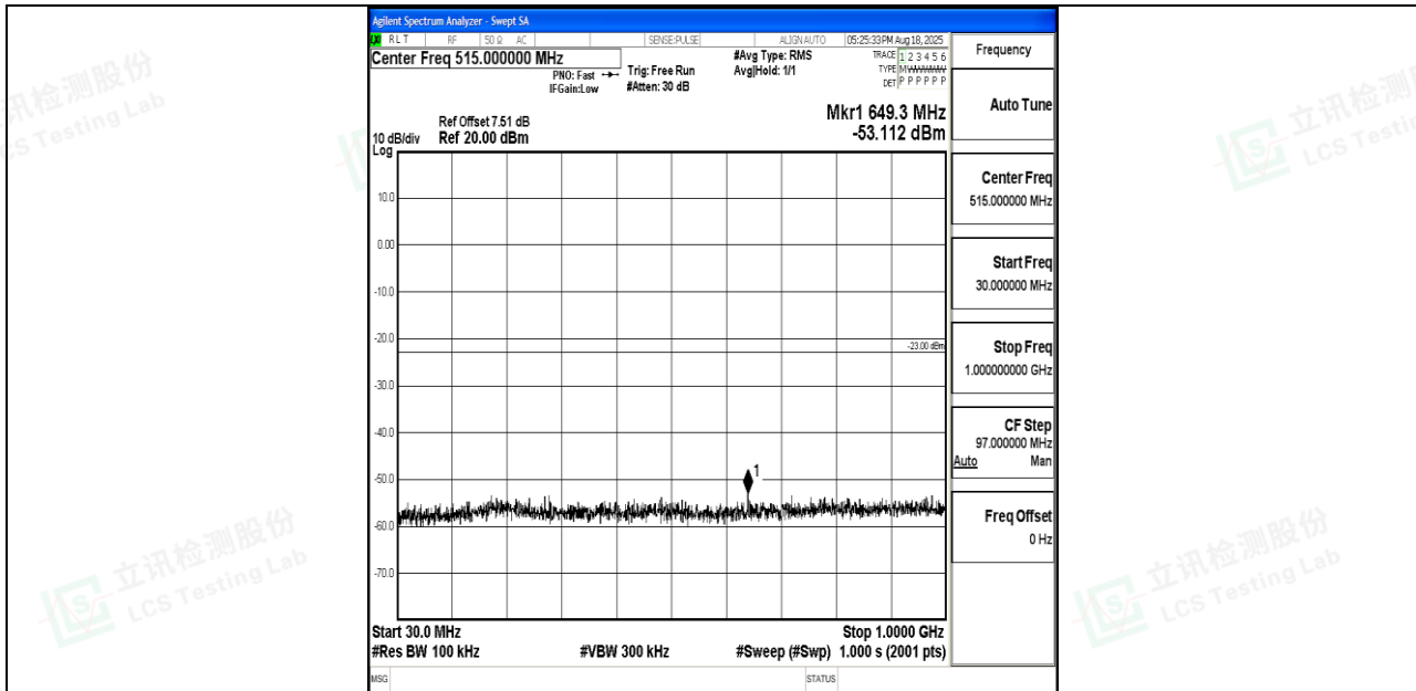
Band25_1.4MHz_16QAM_26365_1RB#0_30~1000_30~1000
