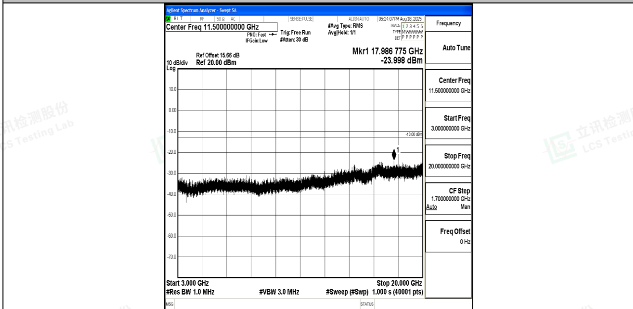
Band25_1.4MHz_QPSK_26047_1RB#0_3000~20000_3000~20000
