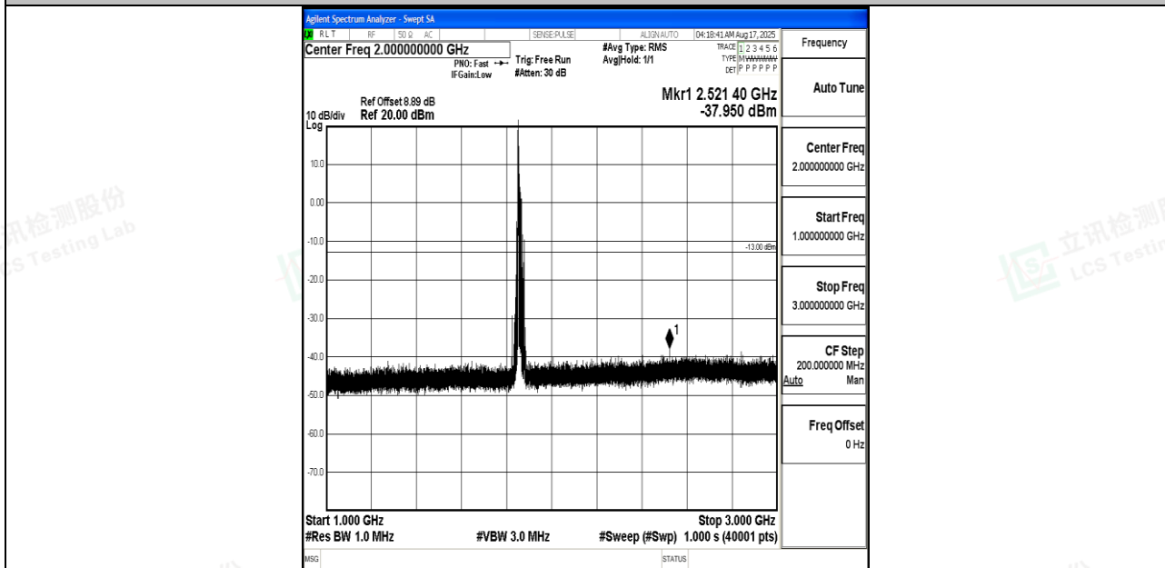
Band25_15MHz_16QAM_26115_1RB#0_1000~3000_1000~3000
