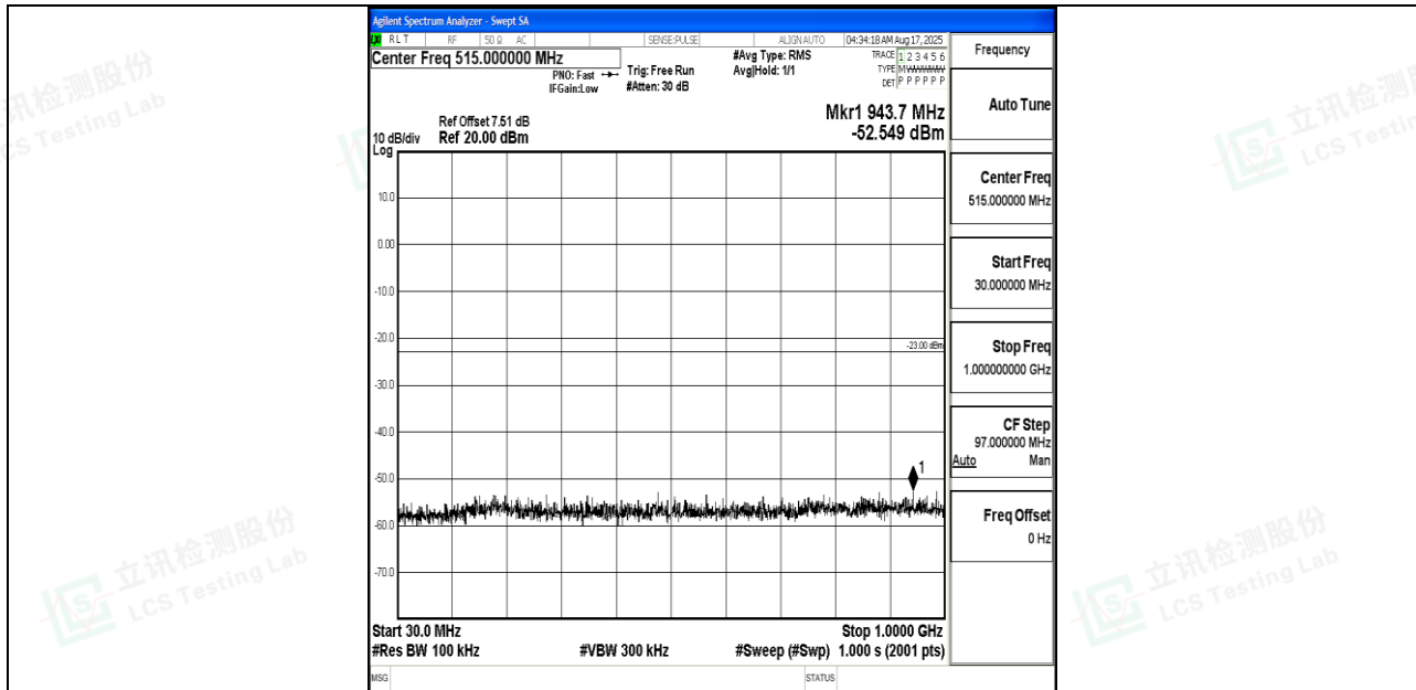
Band25_20MHz_16QAM_26140_1RB#0_30~1000_30~1000
