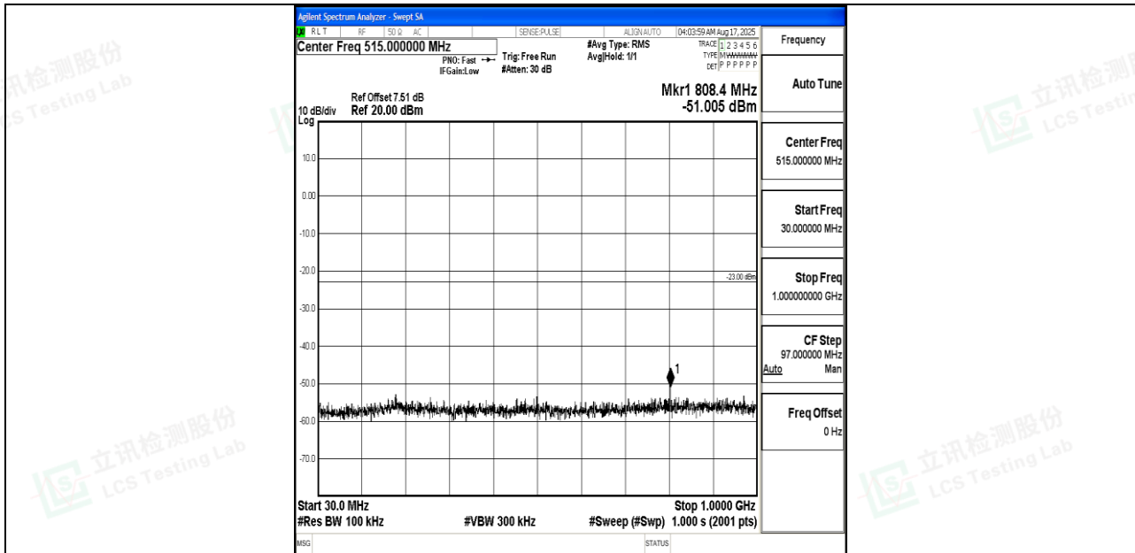
Band25_10MHz_16QAM_26640_1RB#0_30~1000_30~1000
