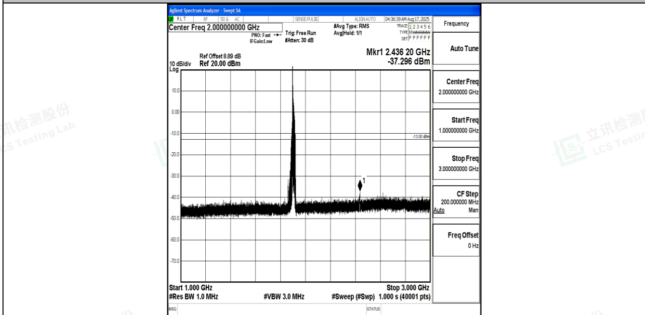
Band25_20MHz_16QAM_26590_1RB#0_1000~3000_1000~3000
