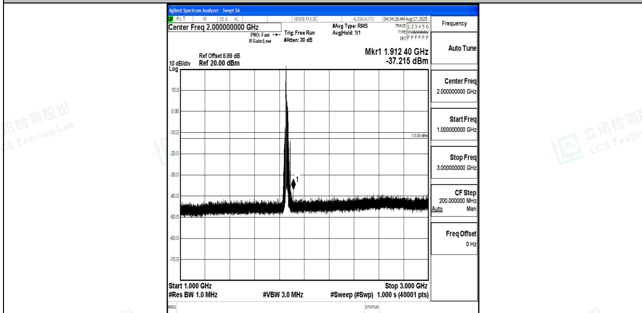
Band25_20MHz_16QAM_26140_1RB#0_1000~3000_1000~3000
