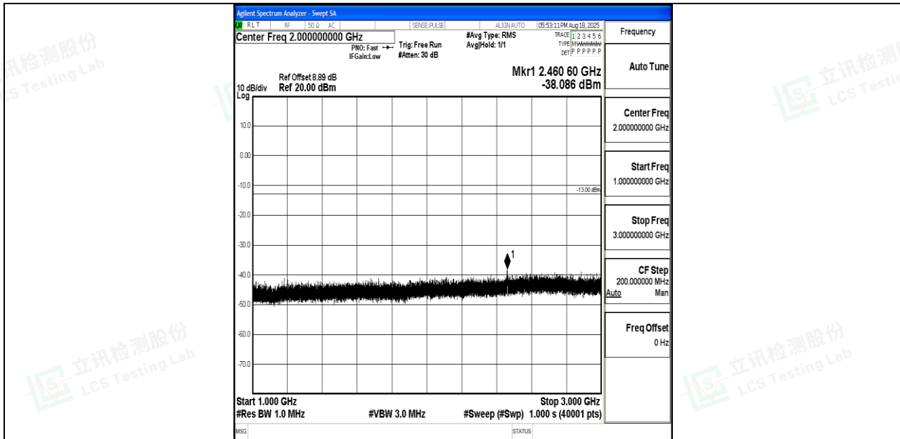
Band26_5MHz_QPSK_26765_1RB#0_1000~3000_1000~3000
