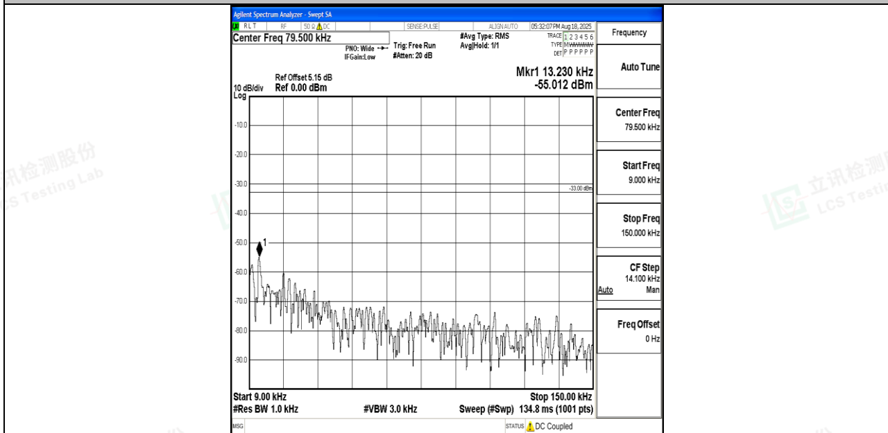
Band26_3MHz_QPSK_26775_1RB#0_0.009~0.15_0.009~0.15
