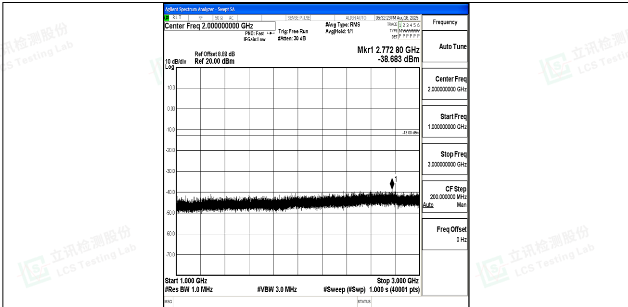
Band26_3MHz_QPSK_26775_1RB#0_1000~3000_1000~3000
