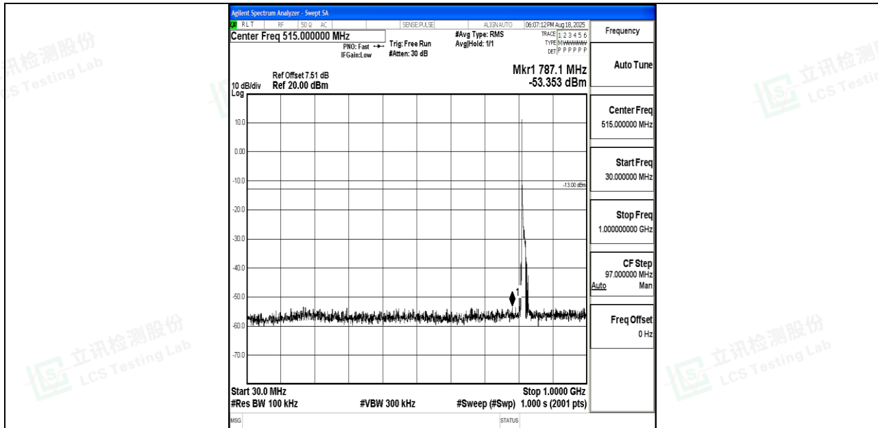
Band26_10MHz_16QAM_26740_1RB#0_30~1000_30~1000
