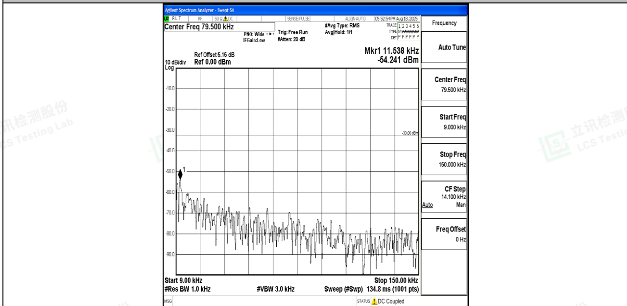
Band26_5MHz_QPSK_26765_1RB#0_0.009~0.15_0.009~0.15
