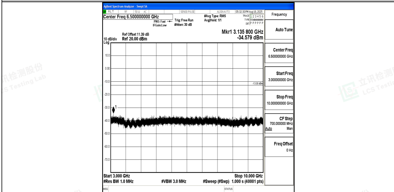
Band26_3MHz_QPSK_26775_1RB#0_3000~10000_3000~10000
