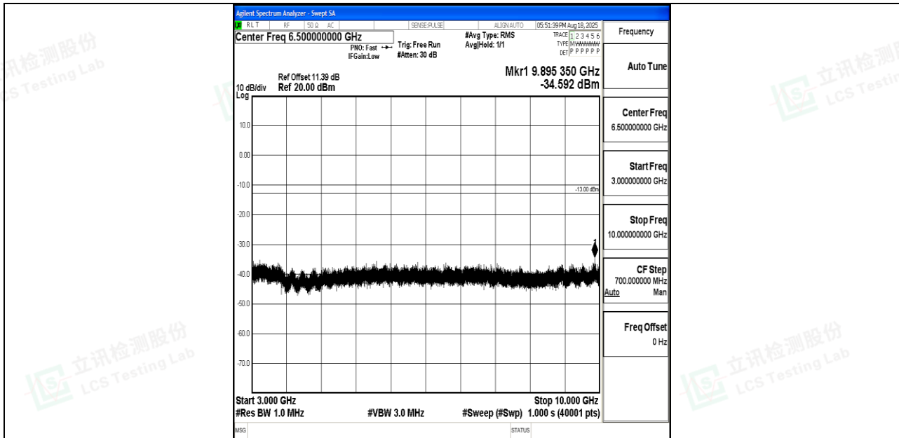
Band26_5MHz_16QAM_26715_1RB#0_3000~10000_3000~10000
