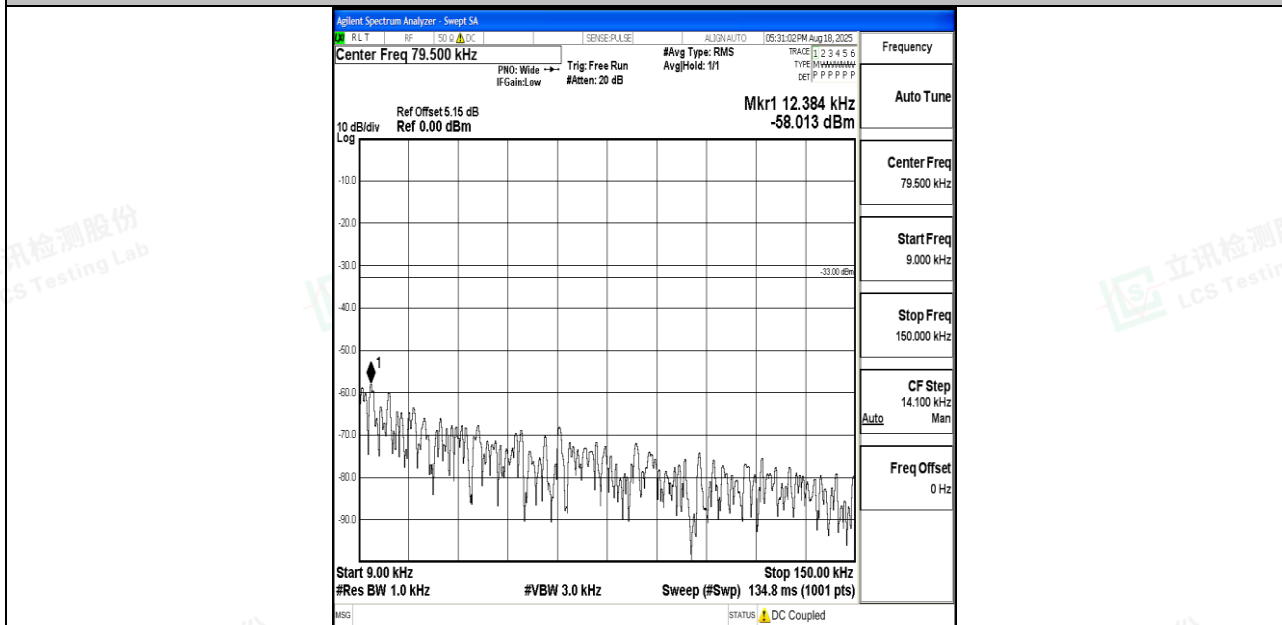
Band26_3MHz_QPSK_26740_1RB#0_0.009~0.15_0.009~0.15
