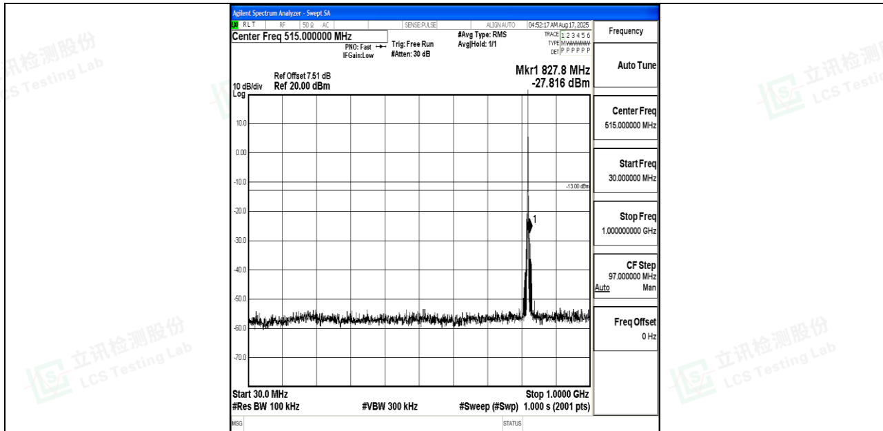
Band26_1.4MHz_16QAM_26783_1RB#0_30~1000_30~1000
