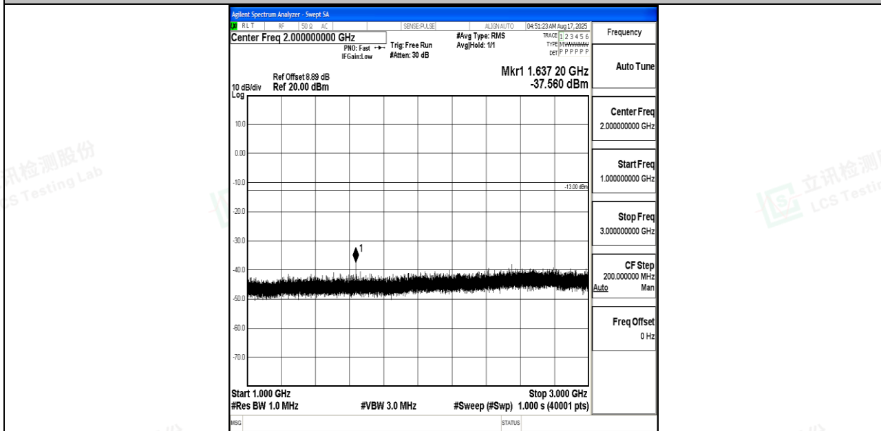
Band26_1.4MHz_16QAM_26740_1RB#0_1000~3000_1000~3000
