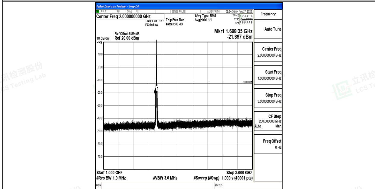
Band66_5MHz_16QAM_131997_1RB#0_1000~3000_1000~3000
