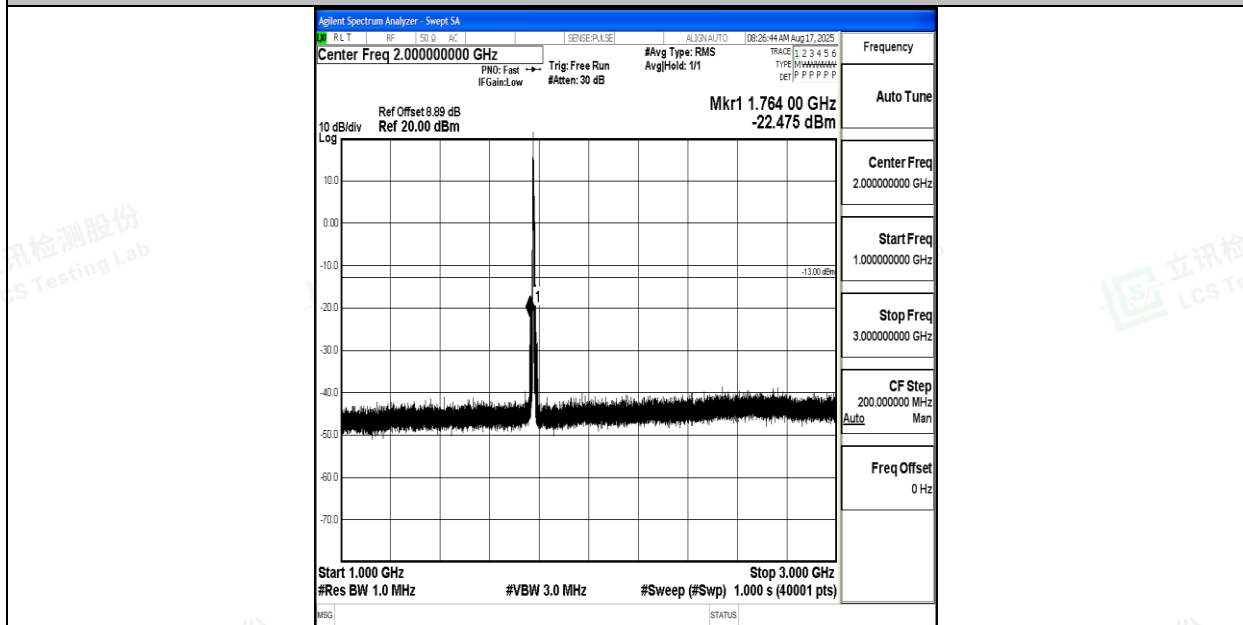
Band66_5MHz_16QAM_132647_1RB#0_1000~3000_1000~3000
