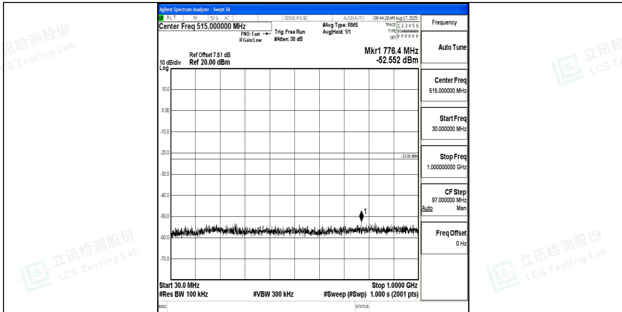
Band66_10MHz_16QAM_132322_1RB#0_30~1000_30~1000
