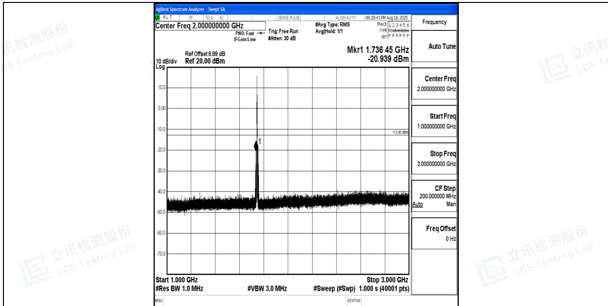
Band66_3MHz_QPSK_132322_1RB#0_1000~3000_1000~3000
