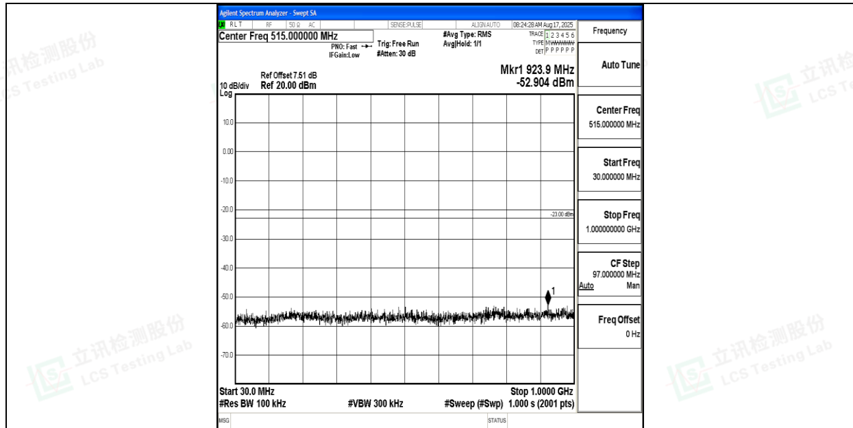
Band66_5MHz_16QAM_131997_1RB#0_30~1000_30~1000
