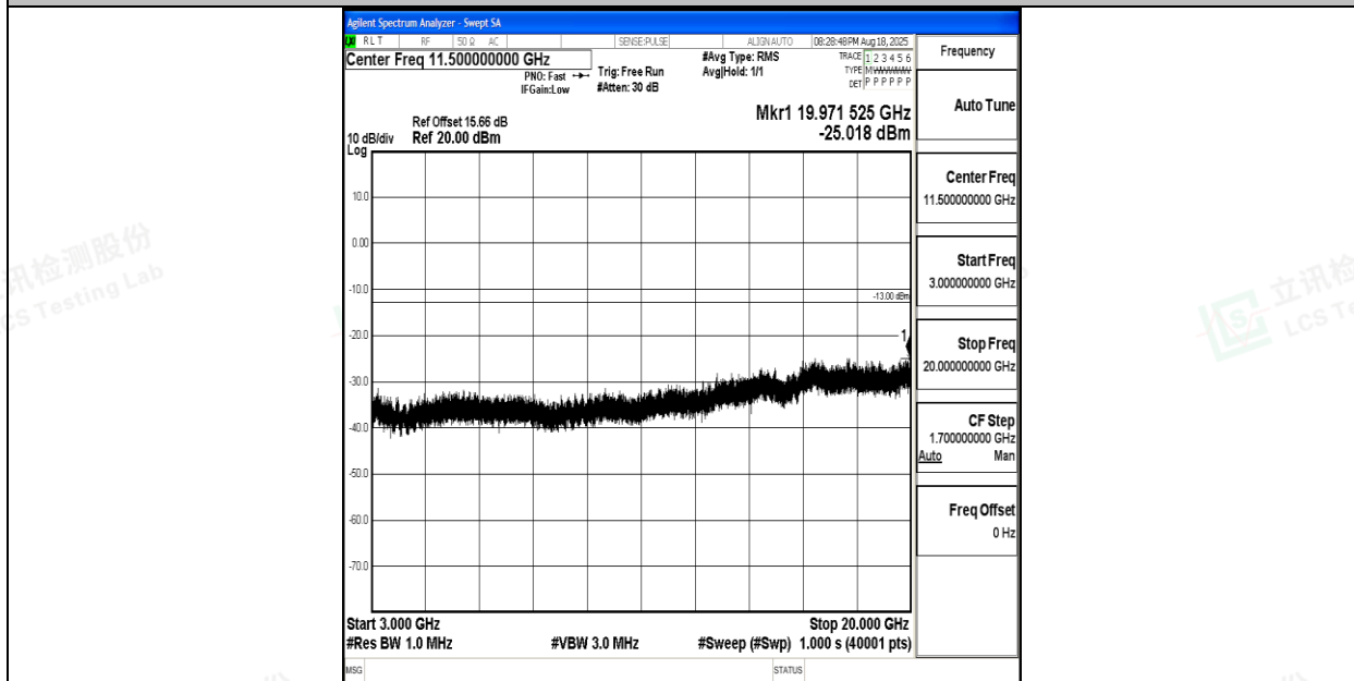
Band66_3MHz_QPSK_132322_1RB#0_3000~20000_3000~20000
