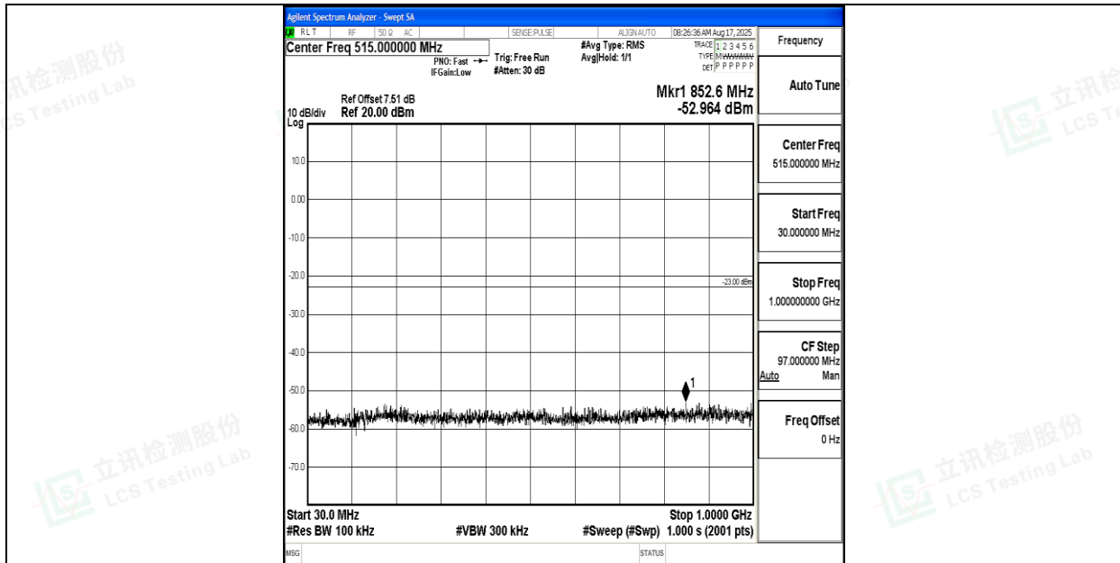
Band66_5MHz_16QAM_132647_1RB#0_30~1000_30~1000
