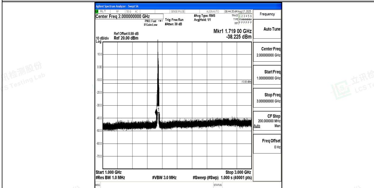
Band66_10MHz_16QAM_132322_1RB#0_1000~3000_1000~3000
