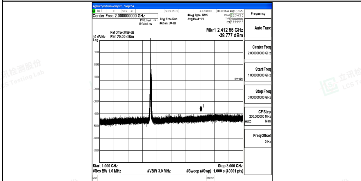
Band66_10MHz_16QAM_132022_1RB#0_1000~3000_1000~3000
