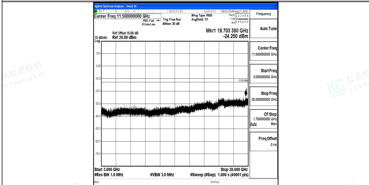
Band66_15MHz_QPSK_132047_1RB#0_3000~20000_3000~20000
