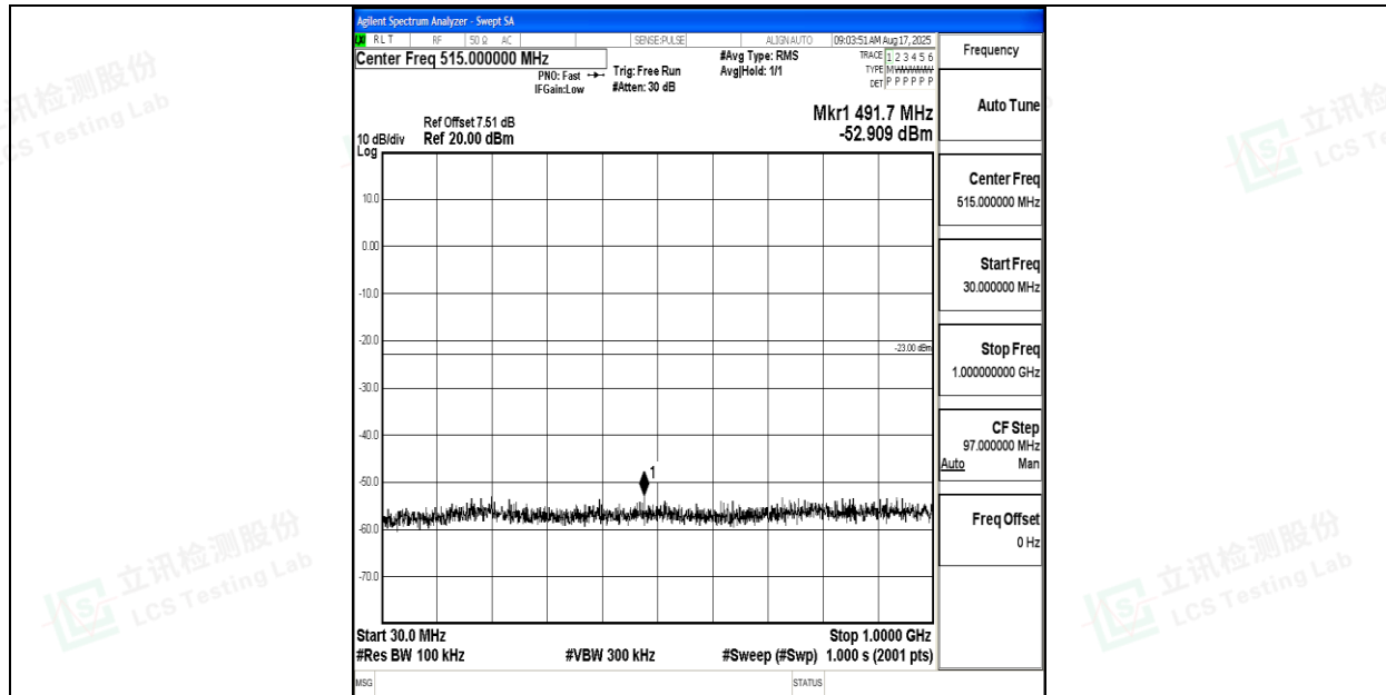
Band66_15MHz_16QAM_132597_1RB#0_30~1000_30~1000
