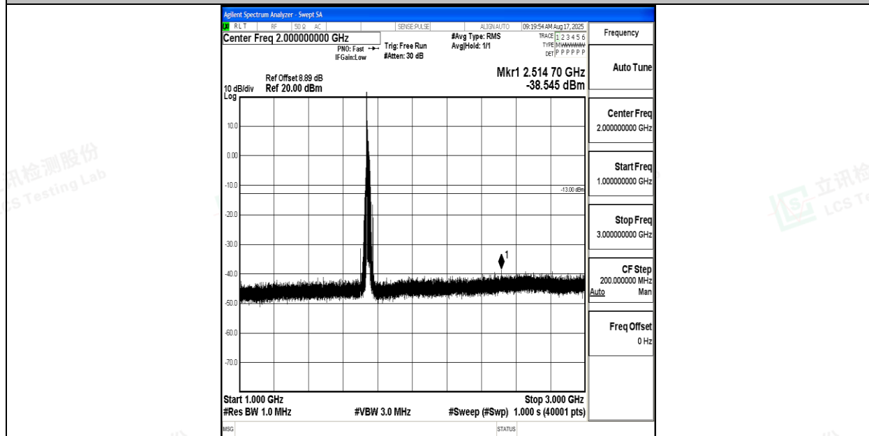
Band66_20MHz_16QAM_132322_1RB#0_1000~3000_1000~3000
