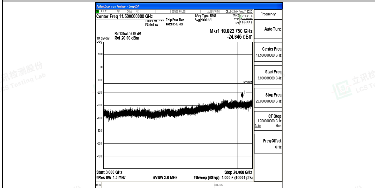
Band66_20MHz_QPSK_132072_1RB#0_3000~20000_3000~20000
