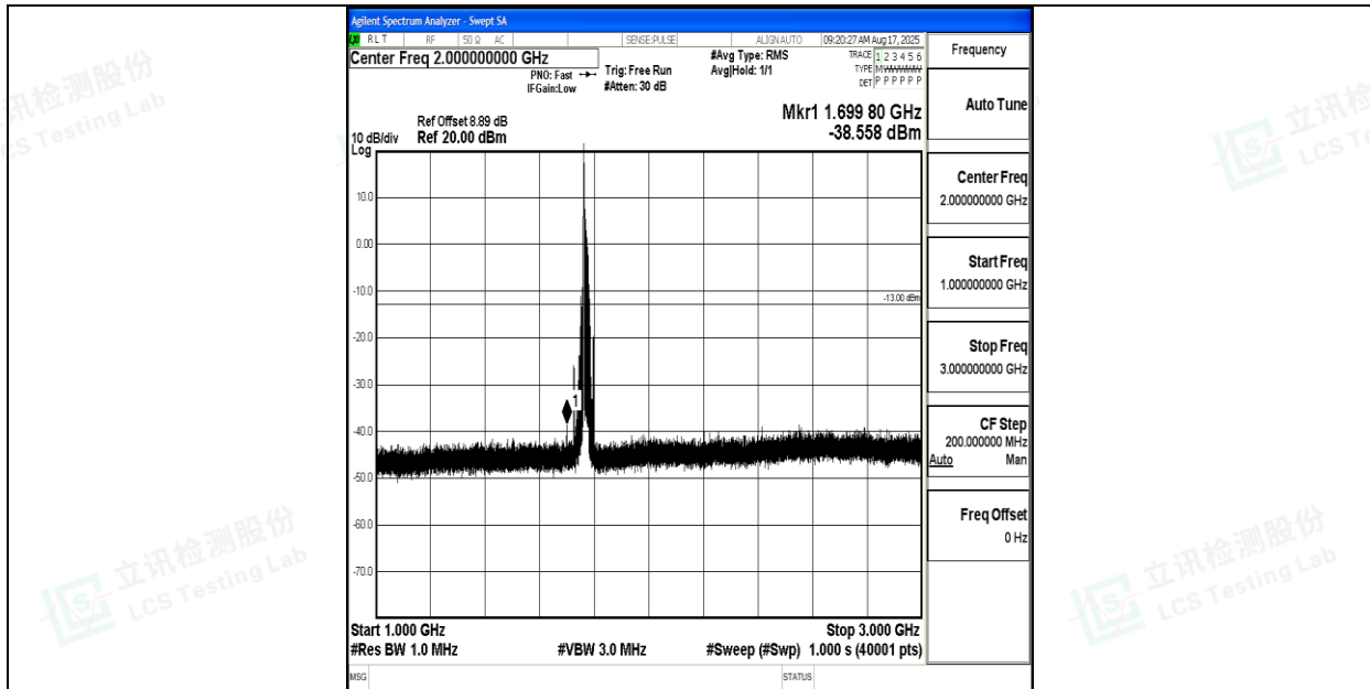
Band66_20MHz_QPSK_132572_1RB#0_1000~3000_1000~3000
