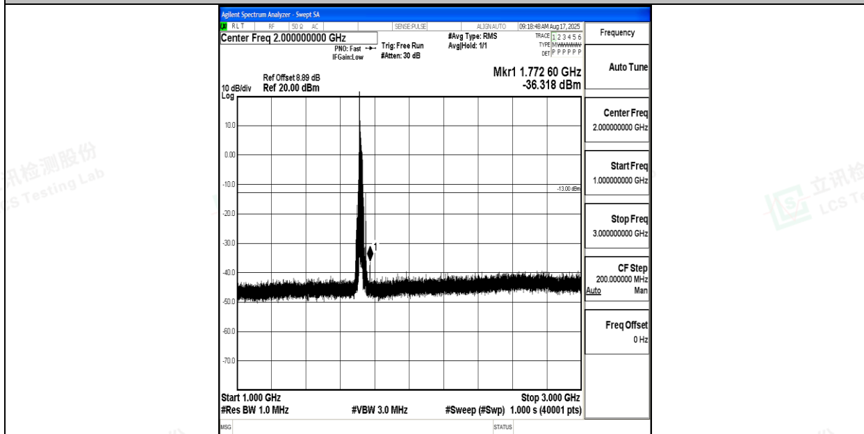
Band66_20MHz_16QAM_132072_1RB#0_1000~3000_1000~3000
