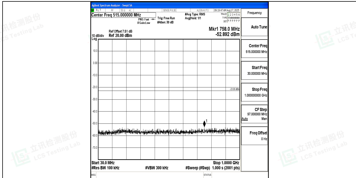
Band66_20MHz_16QAM_132322_1RB#0_30~1000_30~1000
