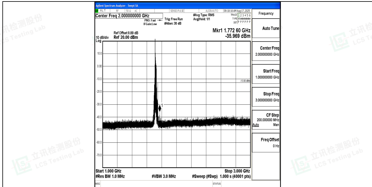
Band66_20MHz_QPSK_132072_1RB#0_1000~3000_1000~3000
