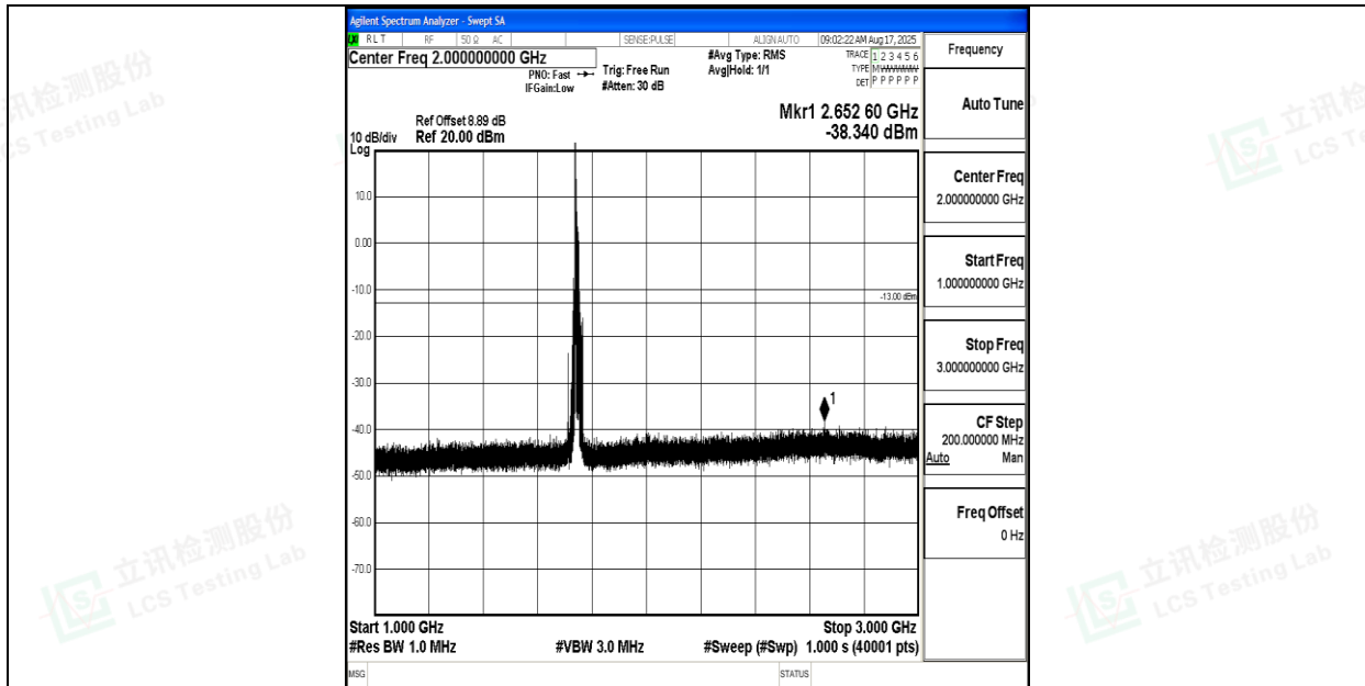
Band66_15MHz_QPSK_132322_1RB#0_1000~3000_1000~3000
