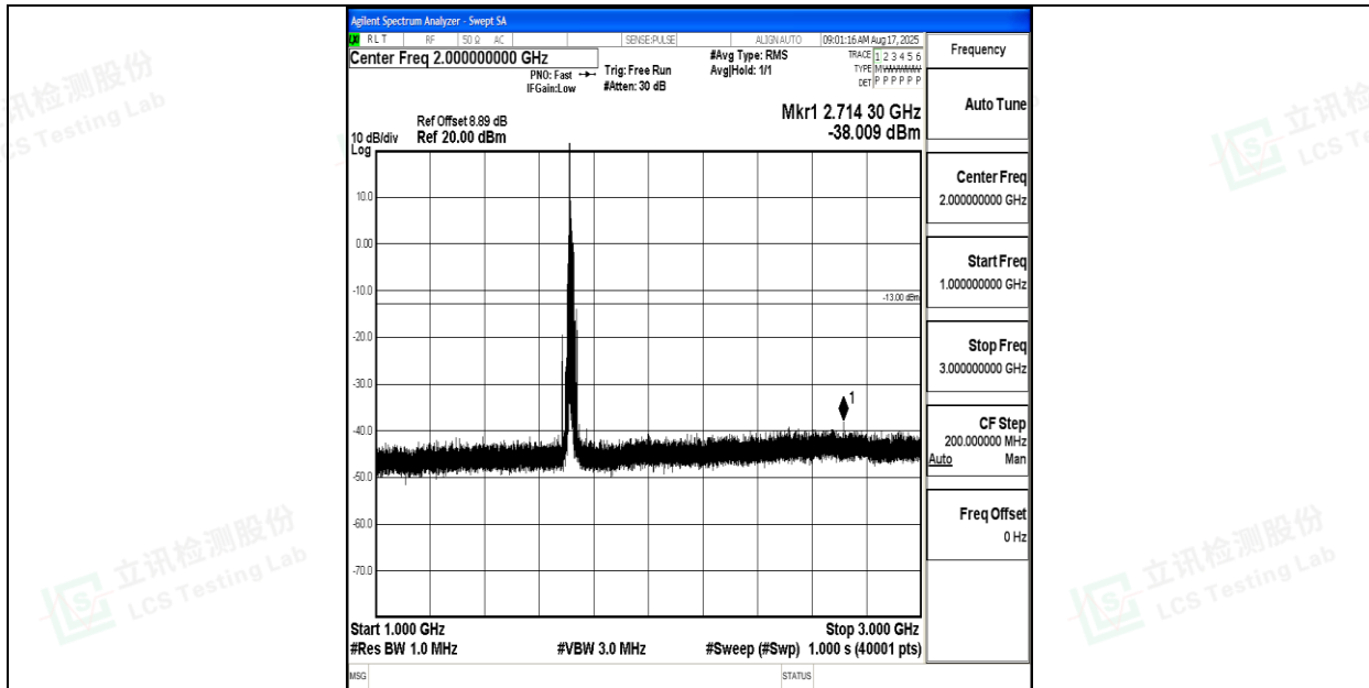
Band66_15MHz_QPSK_132047_1RB#0_1000~3000_1000~3000
