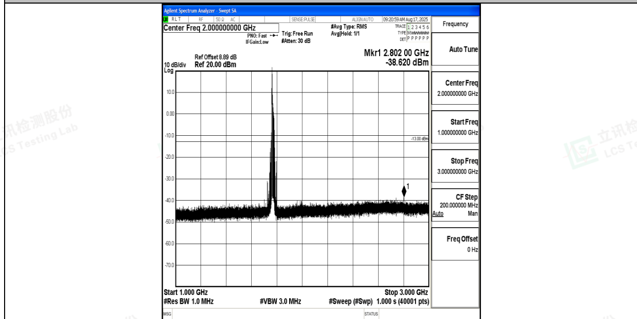
Band66_20MHz_16QAM_132572_1RB#0_1000~3000_1000~3000
