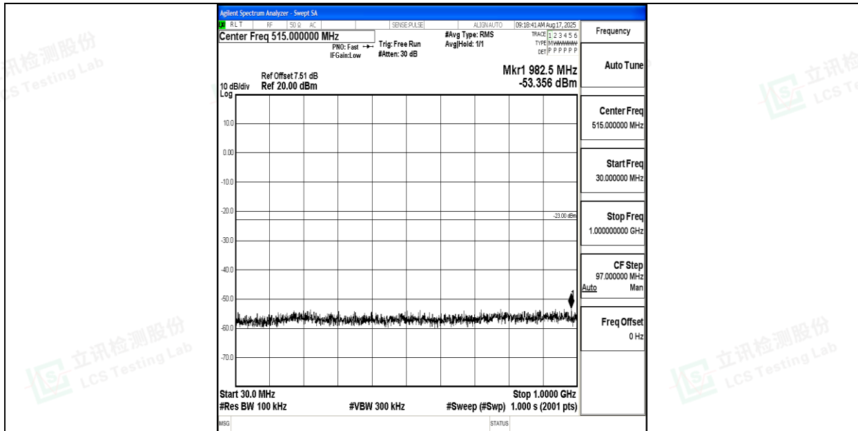
Band66_20MHz_16QAM_132072_1RB#0_30~1000_30~1000
