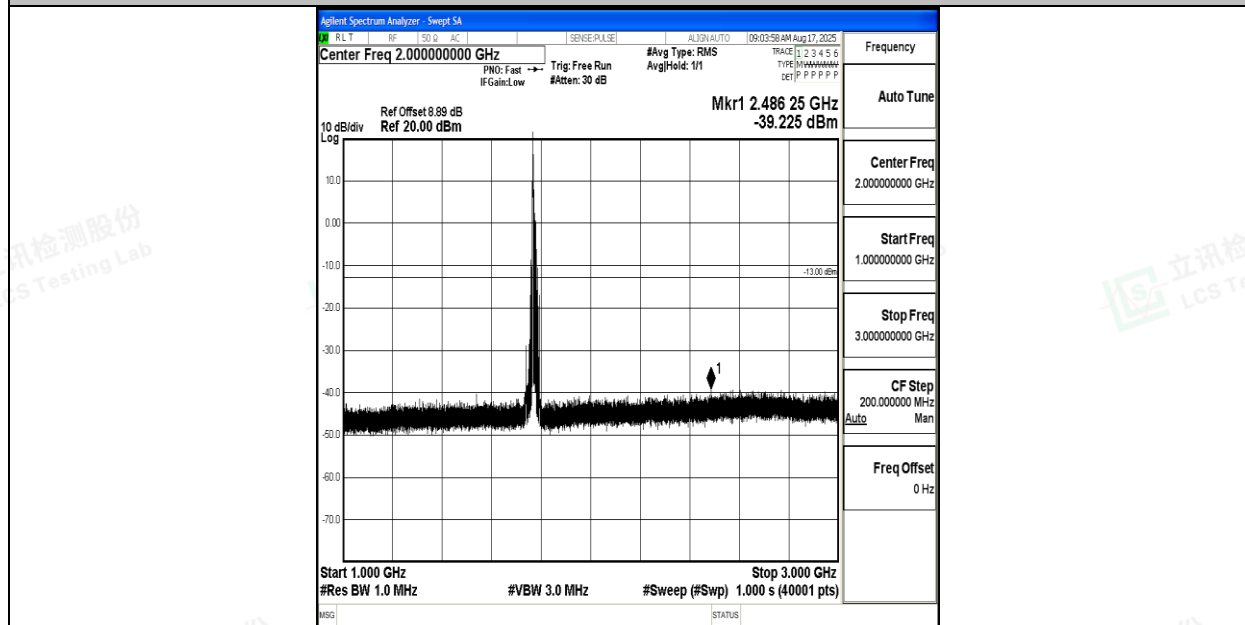
Band66_15MHz_16QAM_132597_1RB#0_1000~3000_1000~3000
