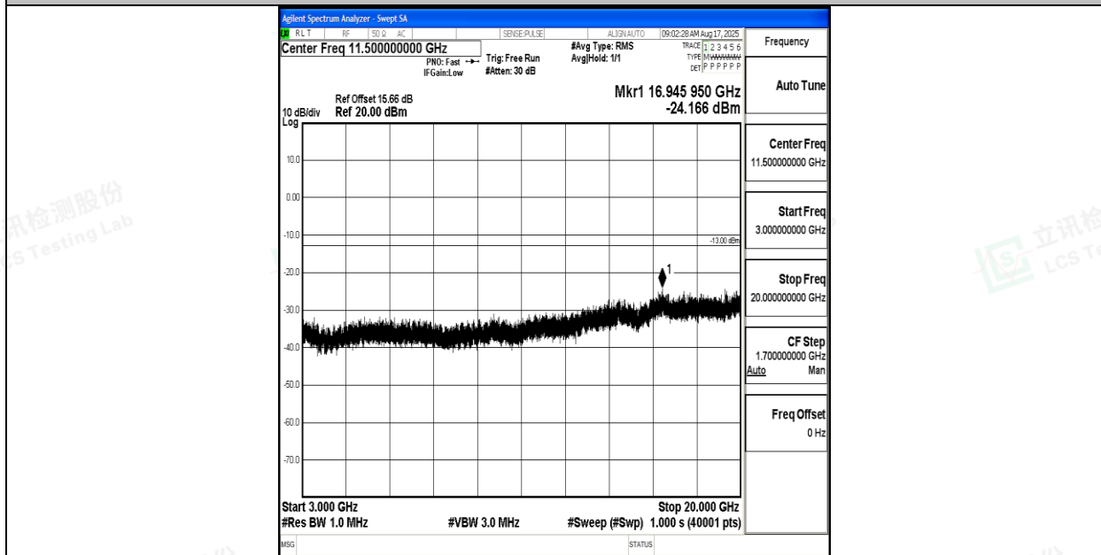
Band66_15MHz_QPSK_132322_1RB#0_3000~20000_3000~20000
