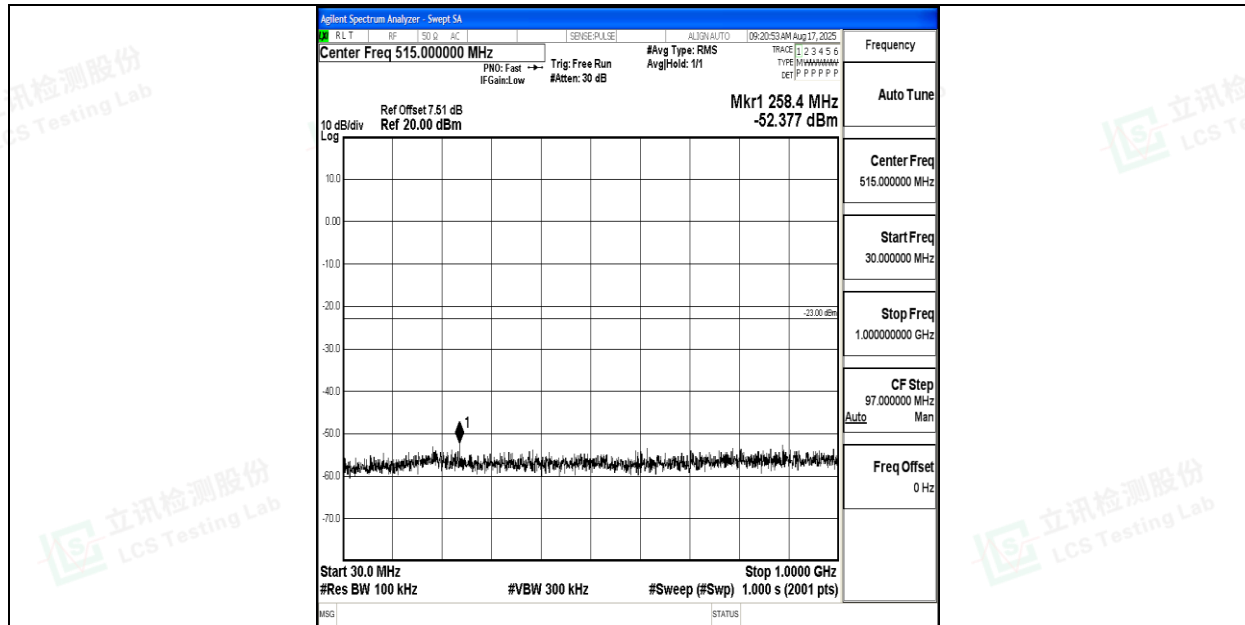
Band66_20MHz_16QAM_132572_1RB#0_30~1000_30~1000
