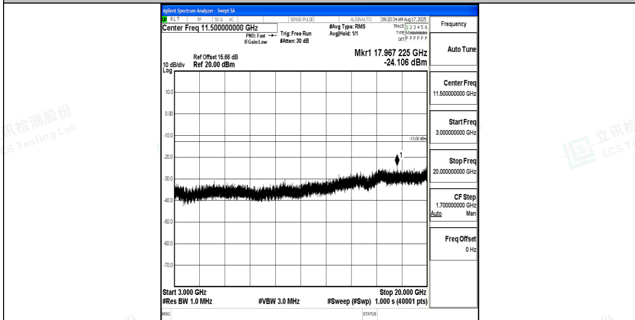
Band66_20MHz_QPSK_132572_1RB#0_3000~20000_3000~20000
