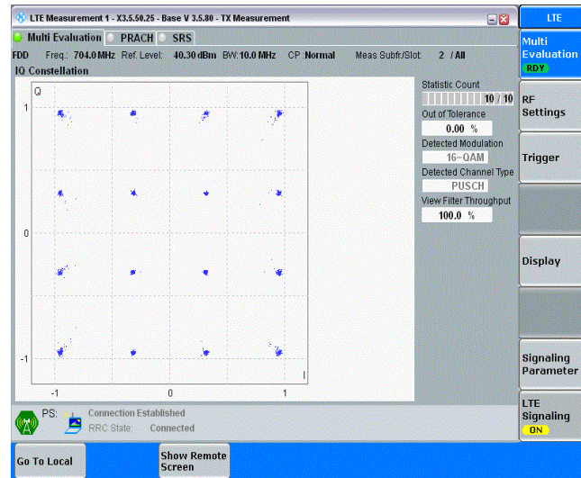
Band12-10MHz-16QAM-23095-25RB#0
