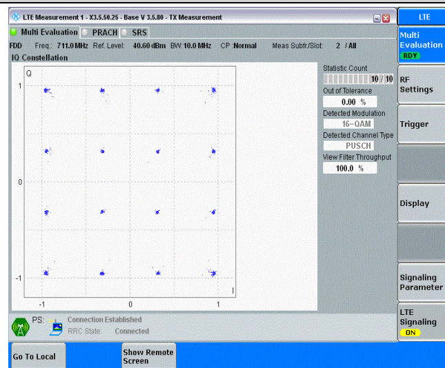
Band12-10MHz-16QAM-23130-25RB#0
