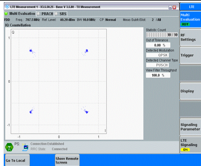
Band12-10MHz-QPSK-23130-25RB#0
