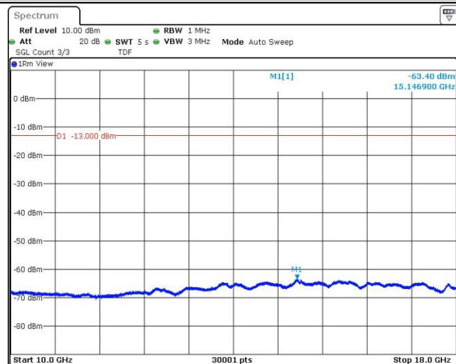
Band5-4182-3-10000~18000MHz
