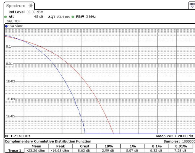
Band4-15MHz-QPSK-20025-75RB#0
