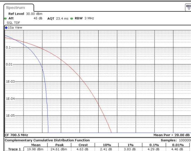
Band12-3MHz-QPSK-23025-15RB#0
