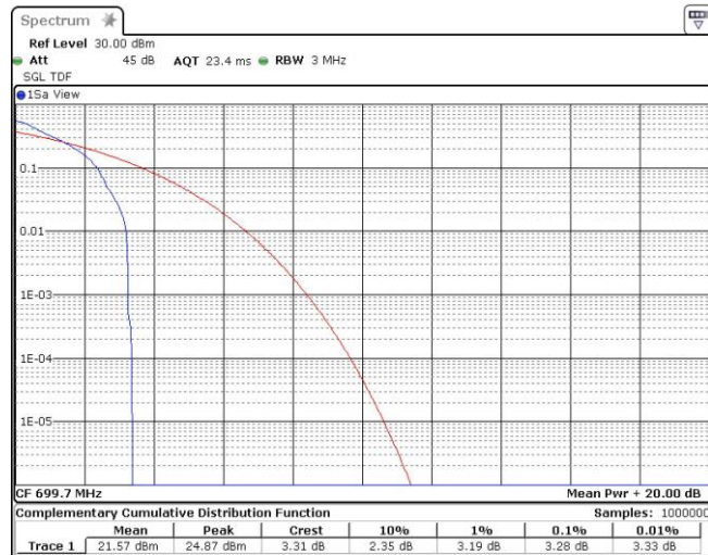
Band12-1.4MHz-QPSK-23017-6RB#0
