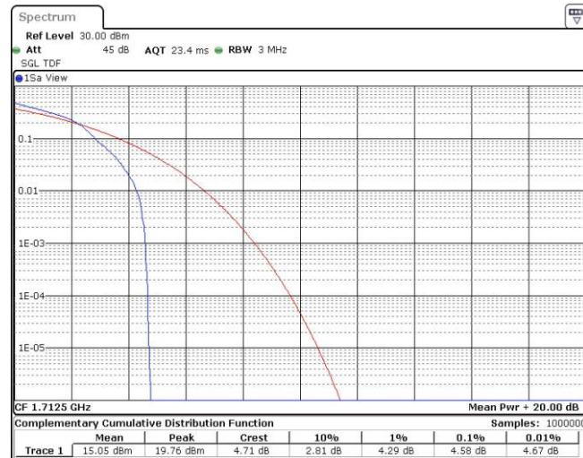
Band4-5MHz-16QAM-19975-25RB#0
