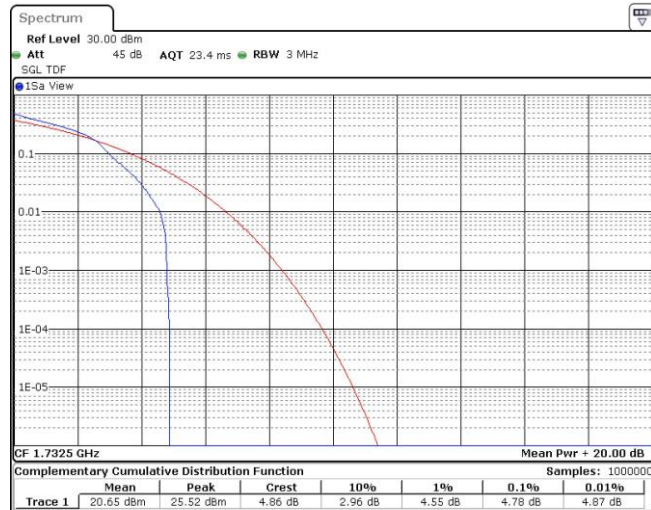
Band4-1.4MHz-16QAM-20175-6RB#0
