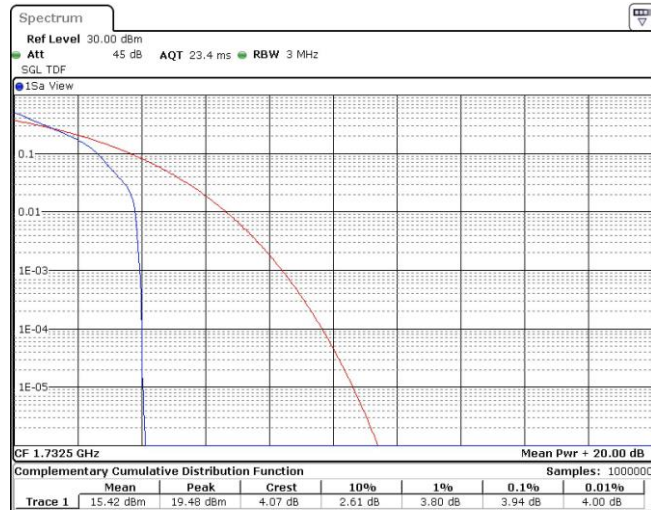
Band4-5MHz-QPSK-20175-25RB#0
