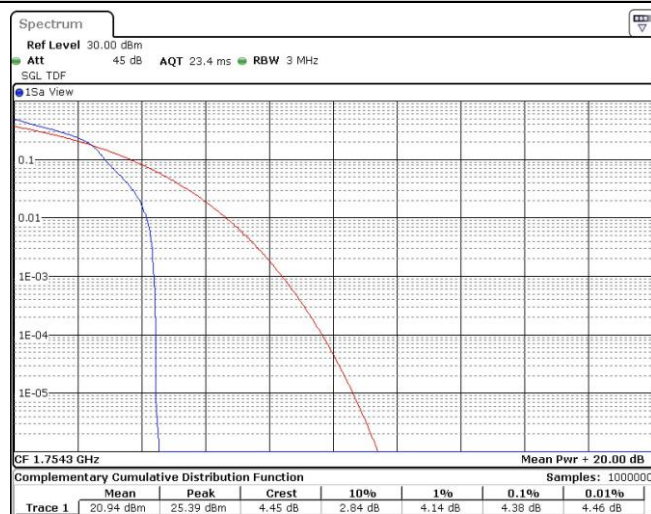
Band4-1.4MHz-16QAM-20393-1RB#0
