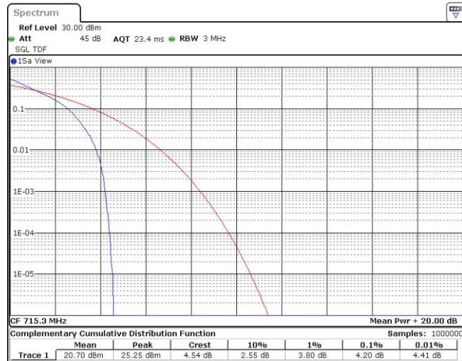
Band12-1.4MHz-16QAM-23017-1RB#0
