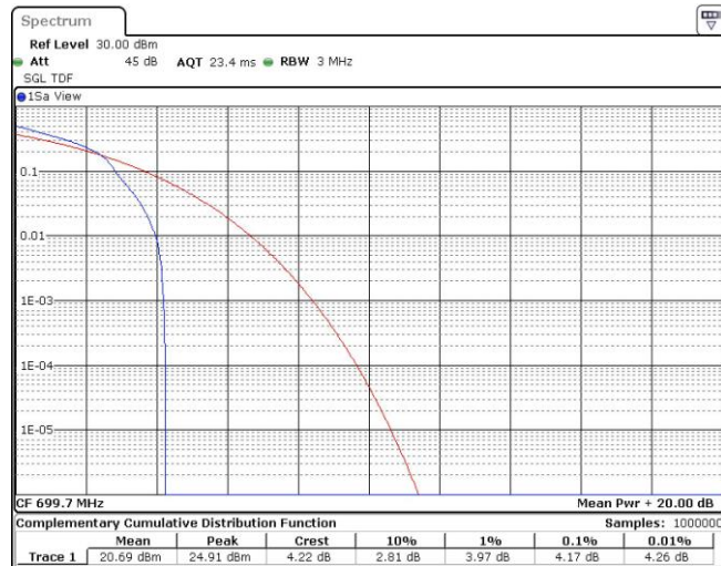
Band12-1.4MHz-16QAM-23017-6RB#0
