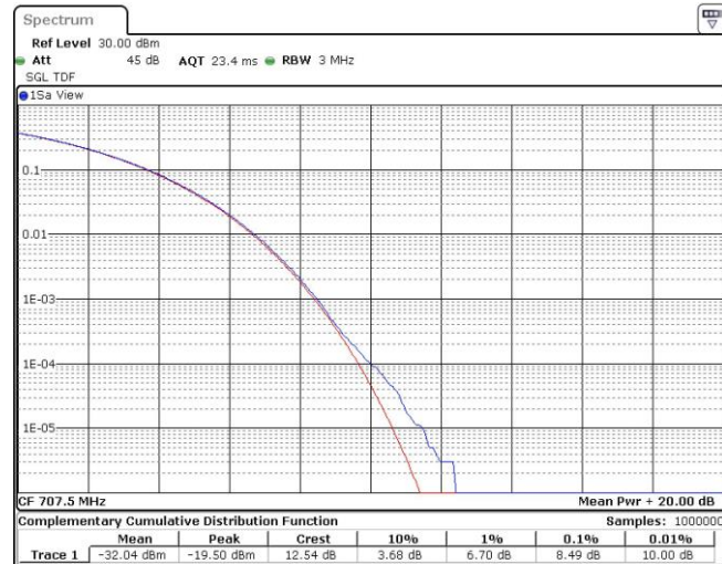
Band12-1.4MHz-16QAM-23095-6RB#0
