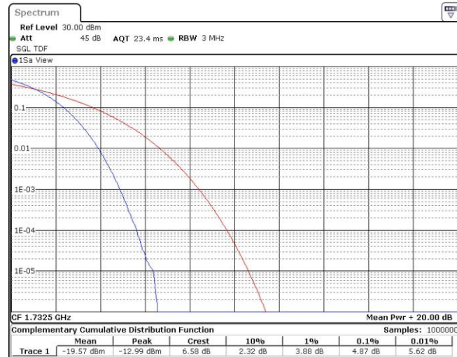
Band4-15MHz-QPSK-20175-75RB#0
