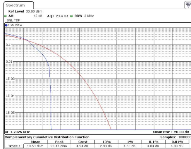
Band4-3MHz-16QAM-20175-15RB#0
