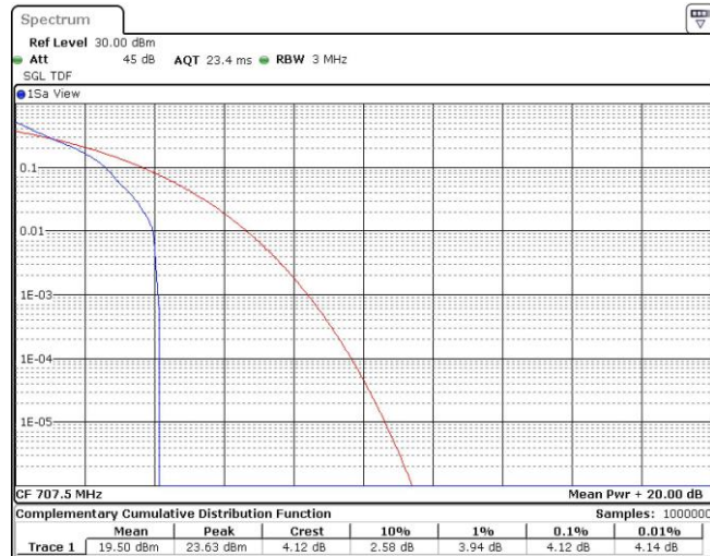
Band12-3MHz-QPSK-23095-15RB#0
