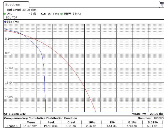
Band4-5MHz-16QAM-20175-25RB#0
