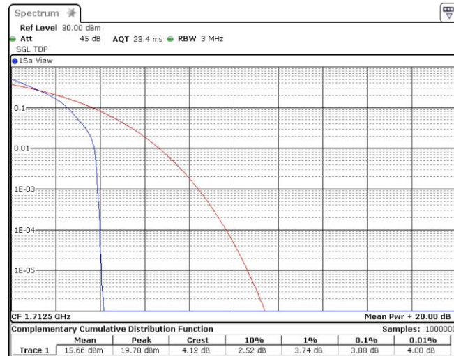
Band4-5MHz-QPSK-19975-25RB#0
