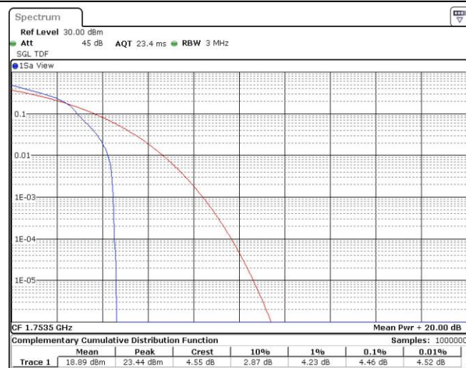
Band4-3MHz-16QAM-20385-15RB#0
