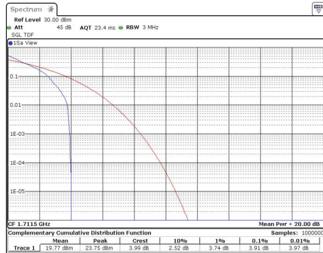
Band4-3MHz-QPSK-19965-15RB#0
