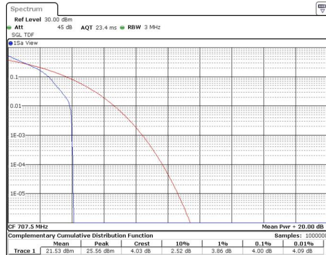
Band12-1.4MHz-QPSK-23095-6RB#0
