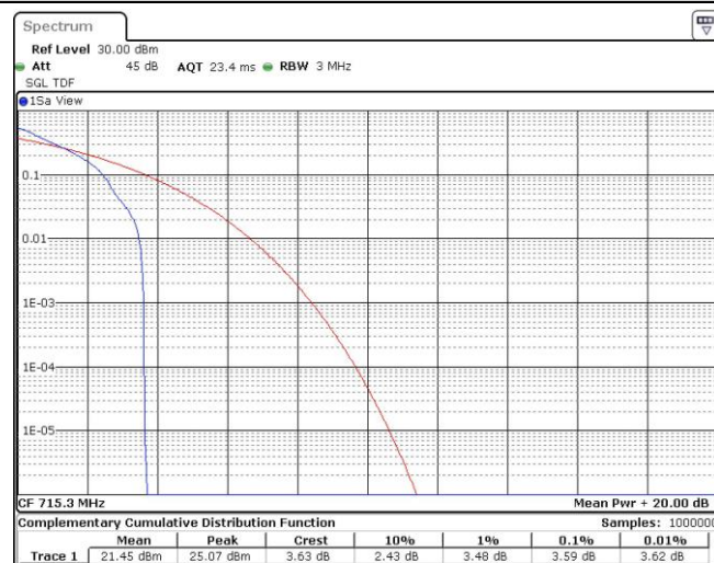
Band12-1.4MHz-QPSK-23173-1RB#0
