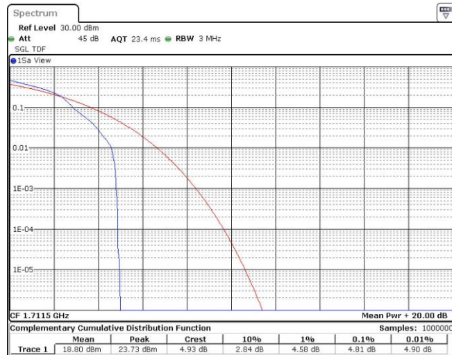
Band4-3MHz-16QAM-19965-15RB#0
