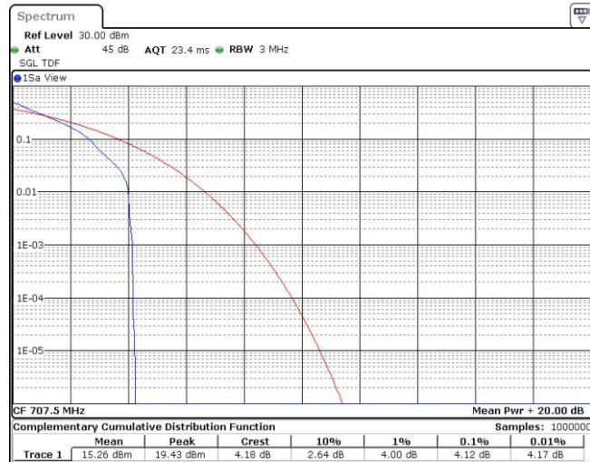
Band12-5MHz-QPSK-23095-25RB#0
