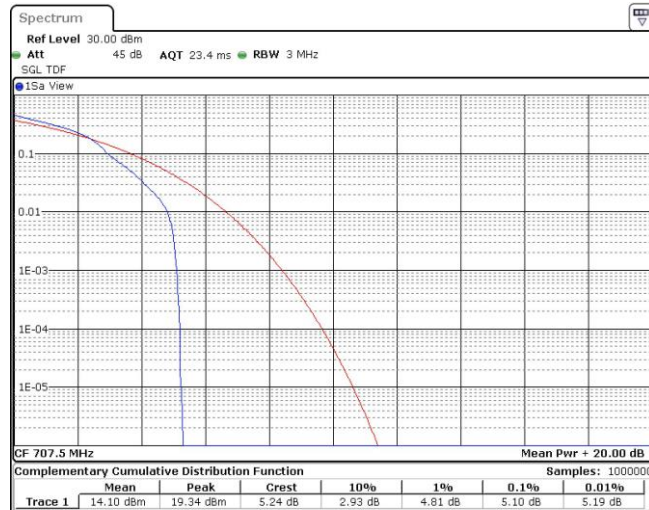
Band12-5MHz-16QAM-23095-25RB#0
