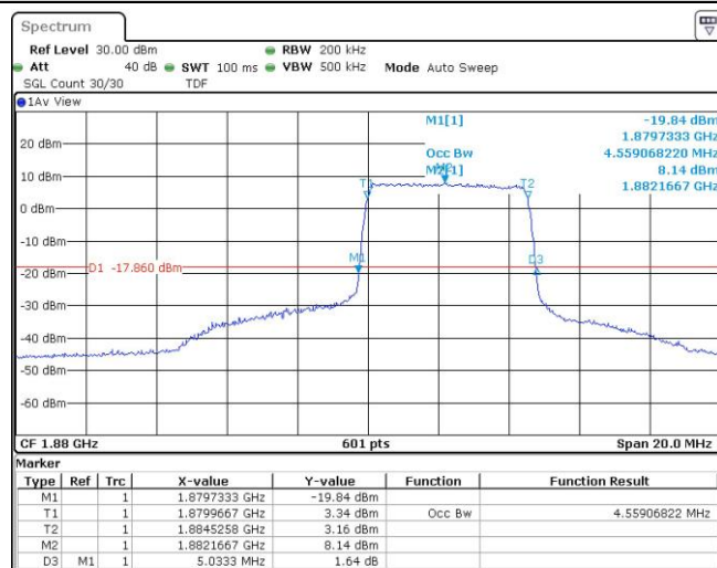
Band2-10MHz-16QAM-18900-25RB#25
