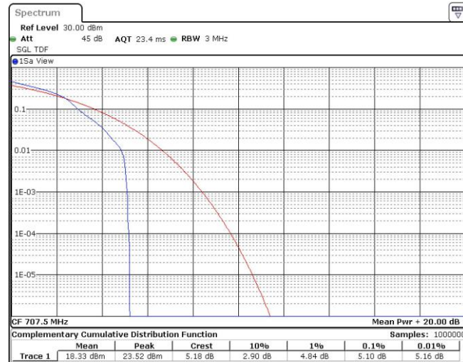
Band12-3MHz-16QAM-23095-15RB#0
