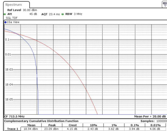
Band12-5MHz-16QAM-23035-1RB#0
