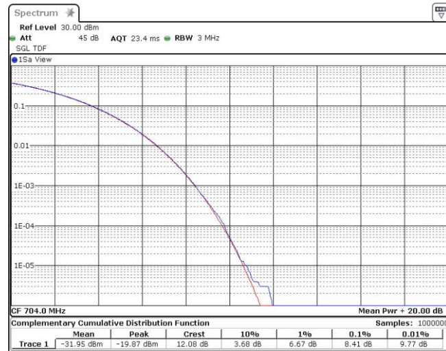
Band12-10MHz-QPSK-23060-50RB#0
