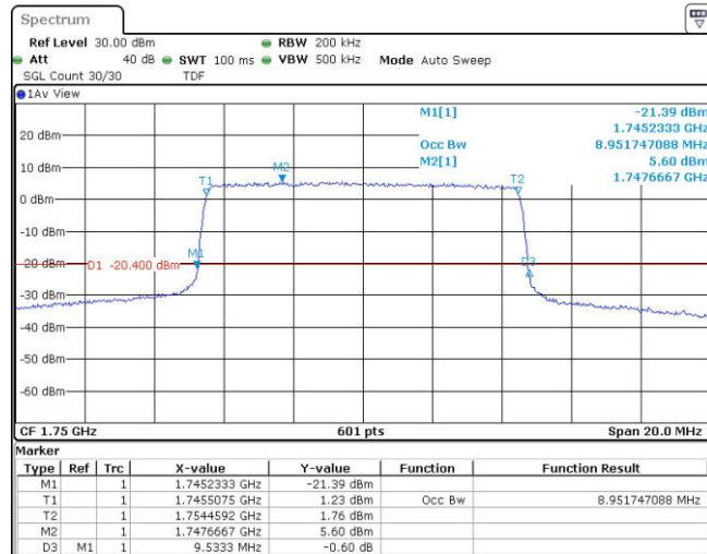
Band4-10MHz-16QAM-20000-1RB#0
