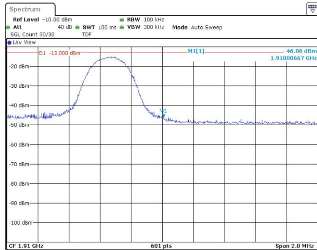
Band2-5MHz-16QAM-19175-1RB#24
