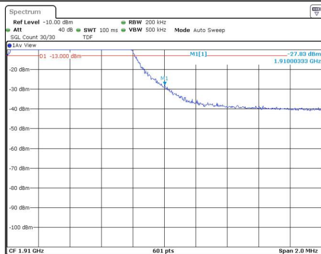
Band2-10MHz-16QAM-19150-25RB#0
