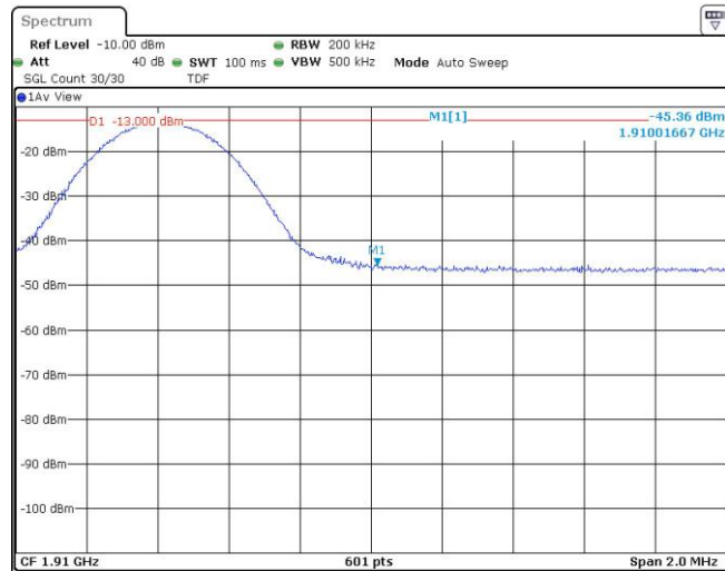
Band2-10MHz-16QAM-19150-1RB#49
