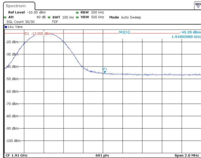
Band2-10MHz-QPSK-19150-1RB#49
