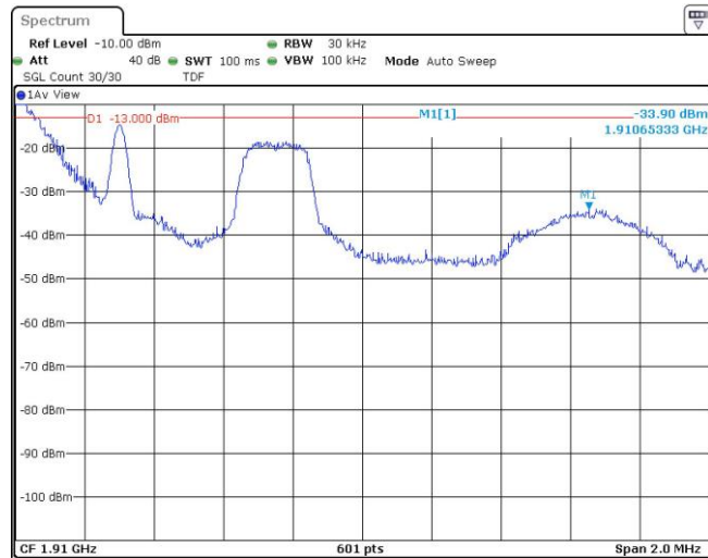
Band2-1.4MHz-QPSK-19193-1RB#5
