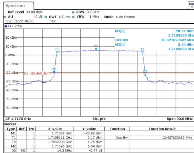
Band4-15MHz-16QAM-20175-38RB#0
