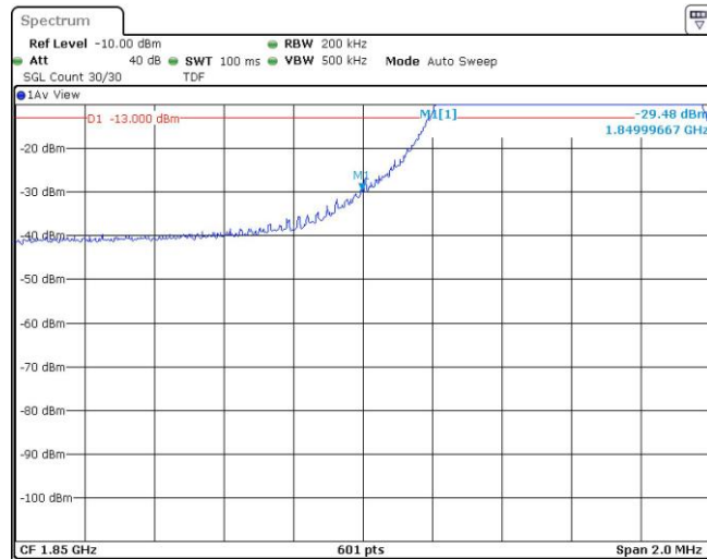
Band2-10MHz-16QAM-18650-1RB#49
