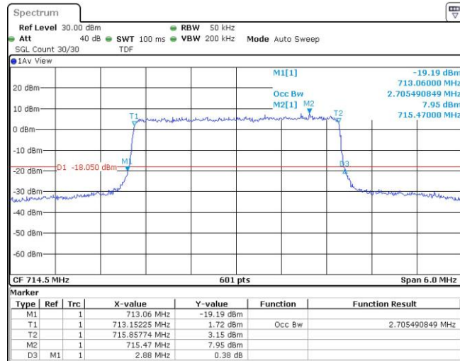
Band12-3MHz-16QAM-23025-15RB#0
