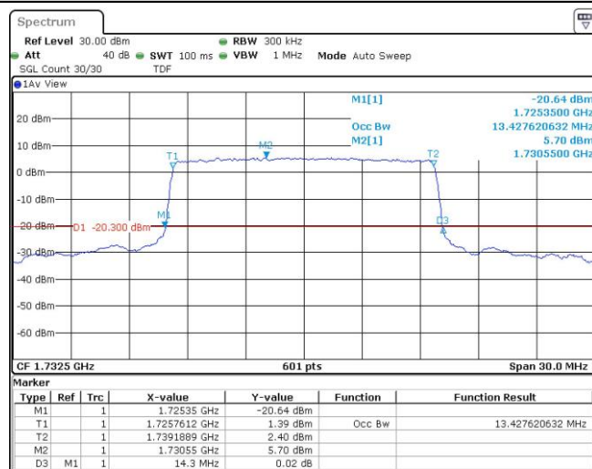
Band4-15MHz-16QAM-20175-38RB#0
