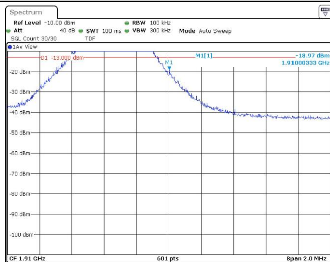
Band2-5MHz-16QAM-19175-25RB#0
