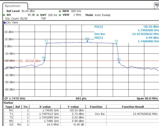
Band4-15MHz-QPSK-20325-38RB#0
