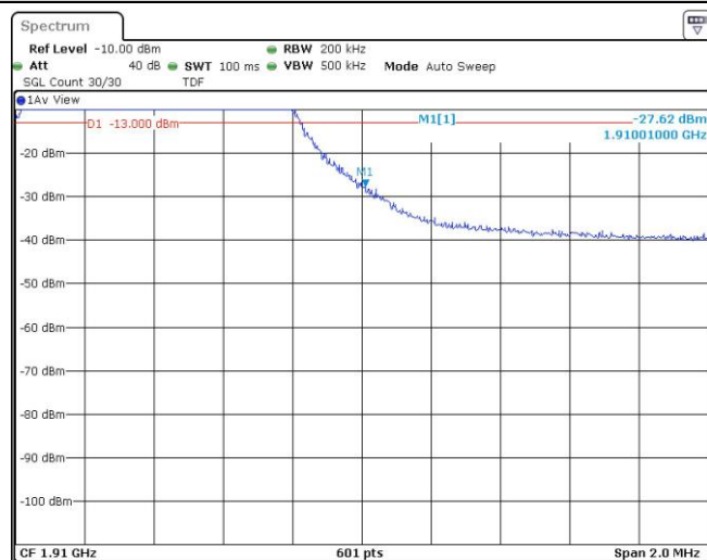
Band2-10MHz-QPSK-19150-25RB#0
