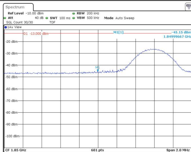
Band2-10MHz-16QAM-18650-25RB#0
