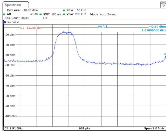
Band2-3MHz-16QAM-19185-1RB#14
