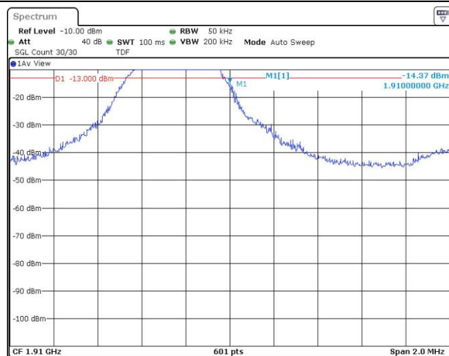
Band2-3MHz-16QAM-19185-15RB#0
