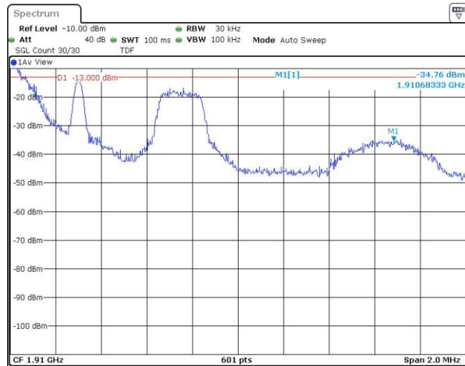
Band2-1.4MHz-16QAM-19193-1RB#5
