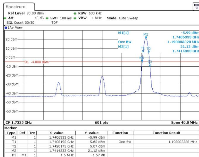
Band4-20MHz-16QAM-20175-1RB#99
