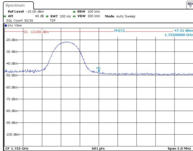
Band4-5MHz-16QAM-20375-1RB#24
