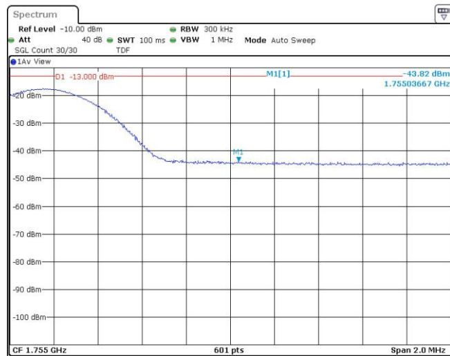
Band4-15MHz-QPSK-20325-1RB#74
