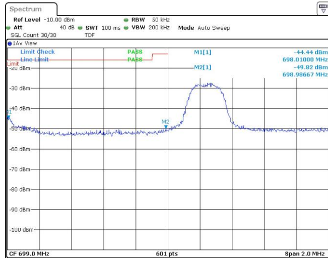
Band12-3MHz-16QAM-23025-15RB#0
