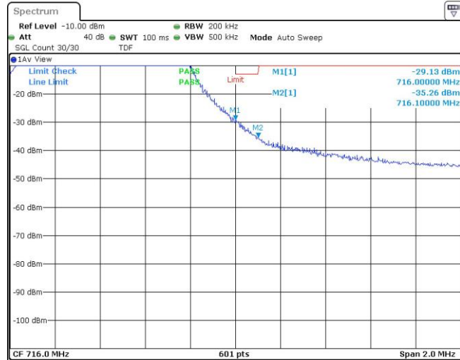
Band12-10MHz-QPSK-23130-50RB#0
