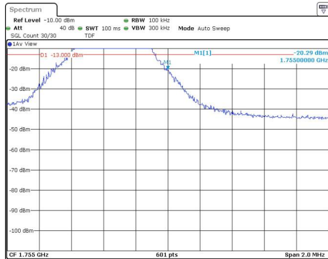
Band4-5MHz-16QAM-20375-25RB#0
