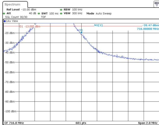
Band12-5MHz-16QAM-23155-25RB#0
