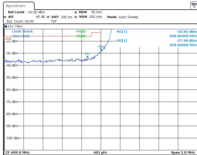
Band12-3MHz-16QAM-23165-1RB#0
