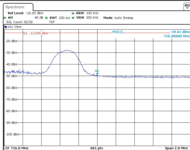
Band12-5MHz-QPSK-23155-1RB#24
