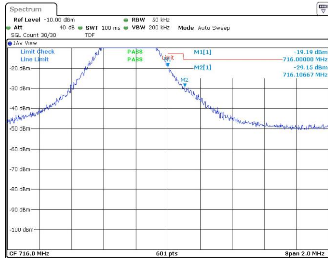
Band12-3MHz-16QAM-23165-15RB#0
