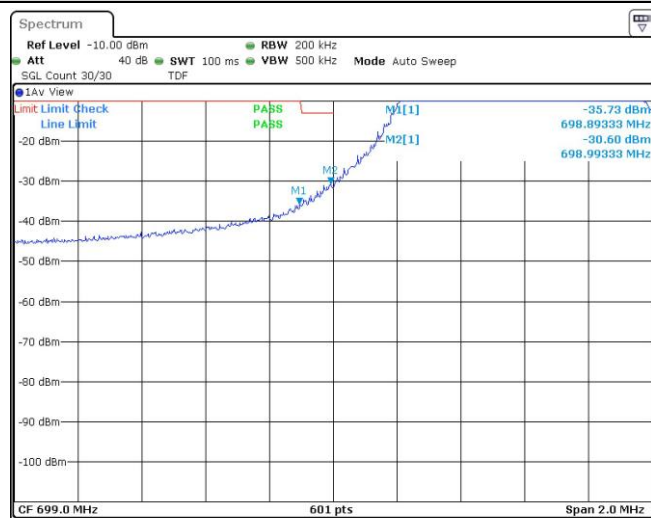
Band12-10MHz-QPSK-23060-1RB#49
