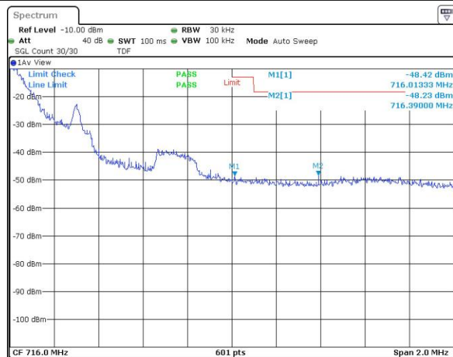
Band12-1.4MHz-QPSK-23173-1RB#5
