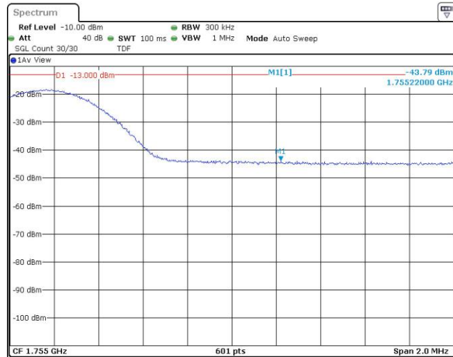
Band4-15MHz-16QAM-20325-1RB#74
