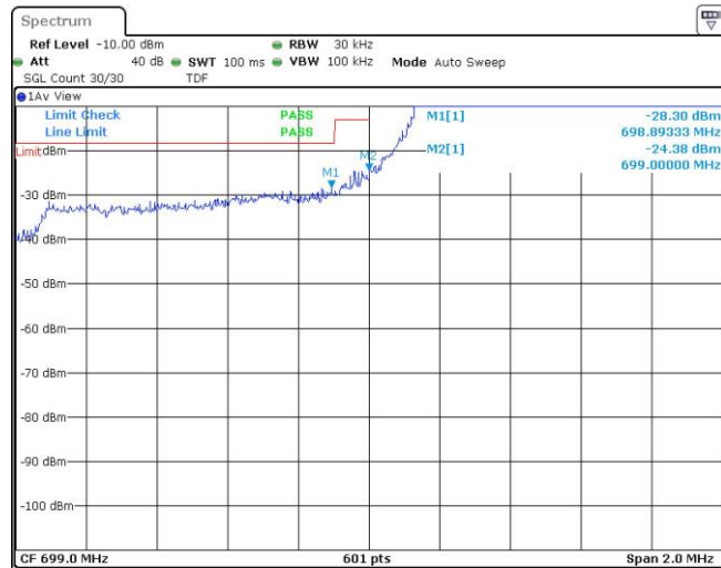
Band12-1.4MHz-QPSK-23173-1RB#0
