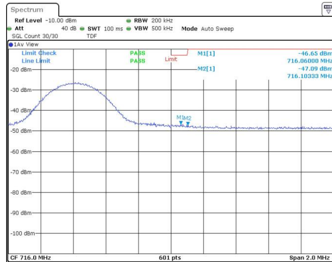
Band12-10MHz-16QAM-23130-1RB#49
