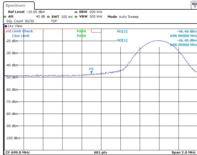
Band12-10MHz-QPSK-23060-50RB#0
