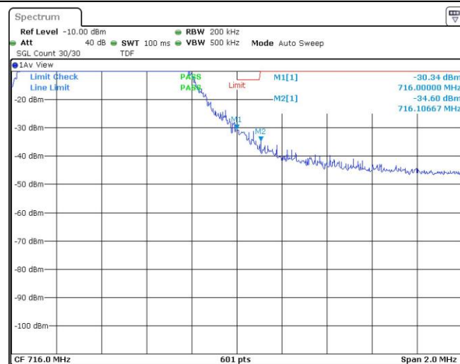
Band12-10MHz-16QAM-23130-1RB#49
