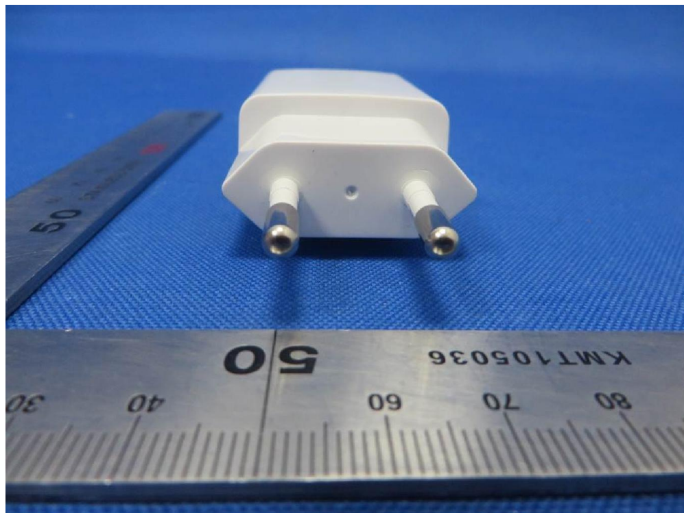
(14) EUT Photo (Adapter, M/N: UC13EU)
