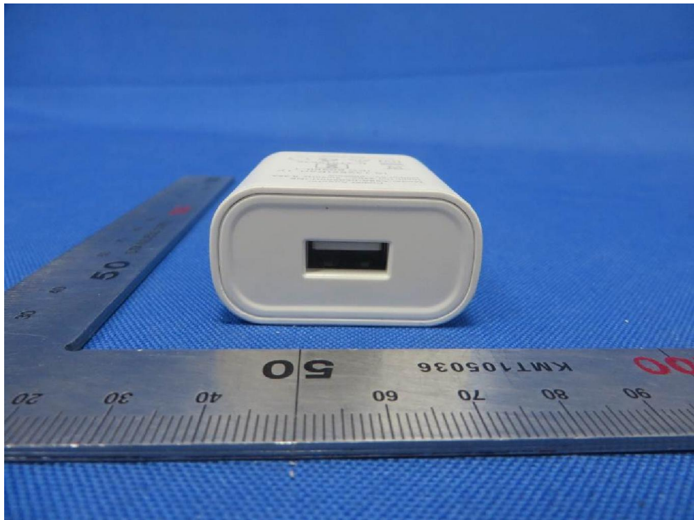
(18) EUT Photo (Adapter, M/N: A98A-050200U-IN2)
