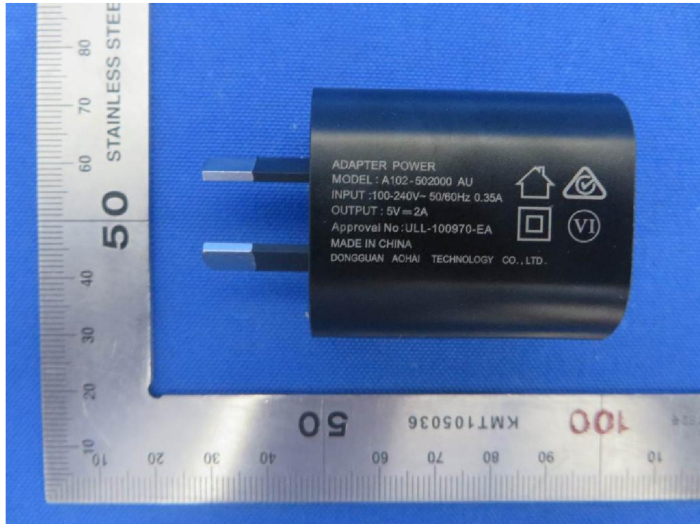
(19) EUT Photo (Adapter, M/N: A102-50200U AU)
