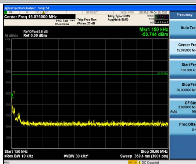
Band26_5MHz_16QAM_26765_1RB#0
