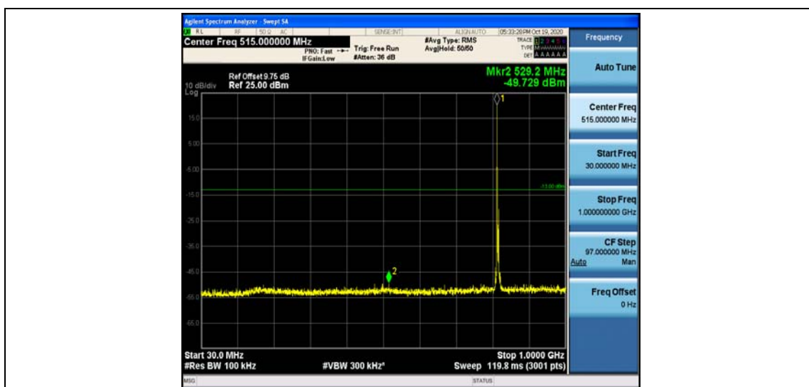
Band26_5MHz_QPSK_26740_1RB#0
