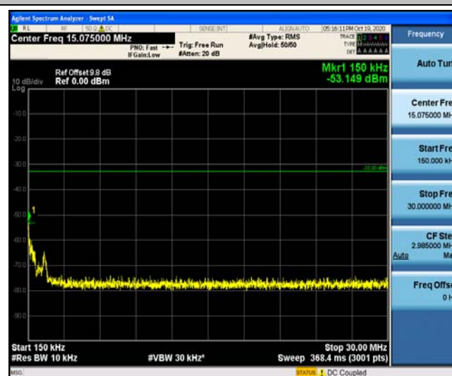
Band26_1.4MHz_16QAM_26697_1RB#0
