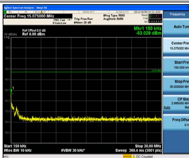
Band26_3MHz_QPSK_26705_1RB#0
