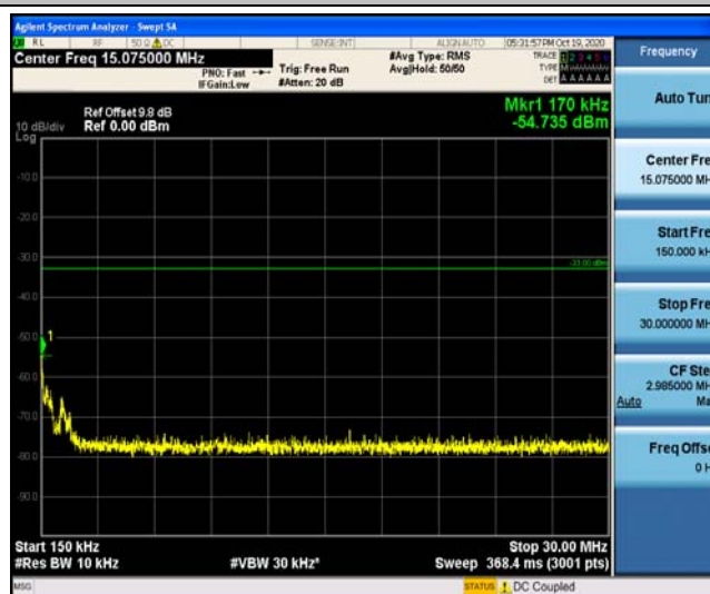
Band26_5MHz_16QAM_26715_1RB#0
