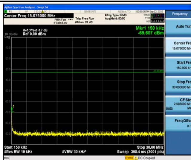
Band25_3MHz_16QAM_24055_1RB#0
