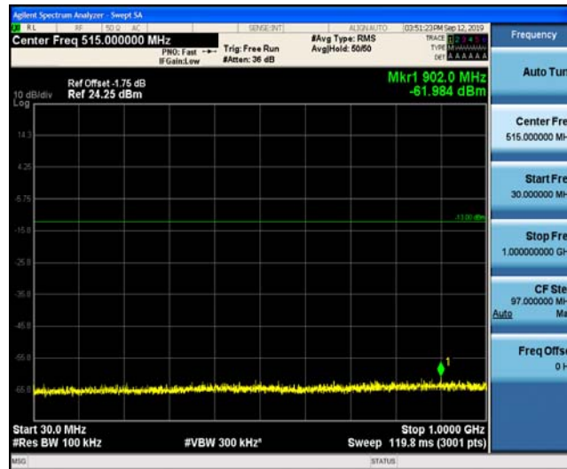
Band25_1.4MHz_QPSK_24047_1RB#0
