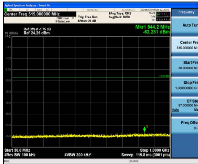
Band25_3MHz_QPSK_24055_1RB#0
