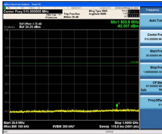
Band25_1.4MHz_16QAM_24047_1RB#0
