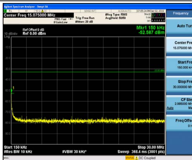
Band25_3MHz_16QAM_24055_1RB#0
