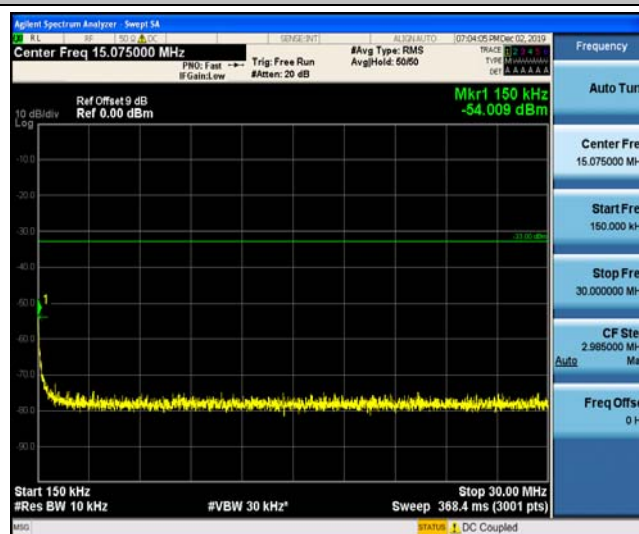
Band25_3MHz_QPSK_24055_1RB#0
