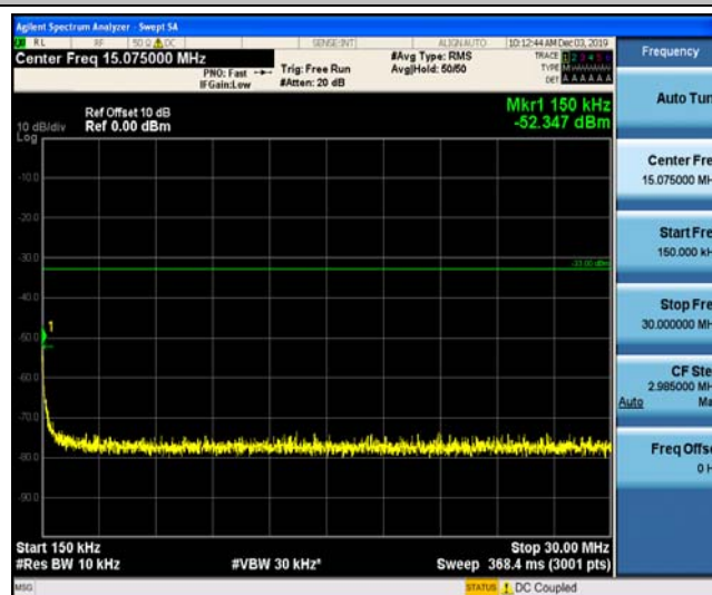
Band66_5MHz_16QAM_132647_1RB#0
