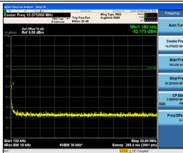
Band66_5MHz_16QAM_131997_1RB#0
