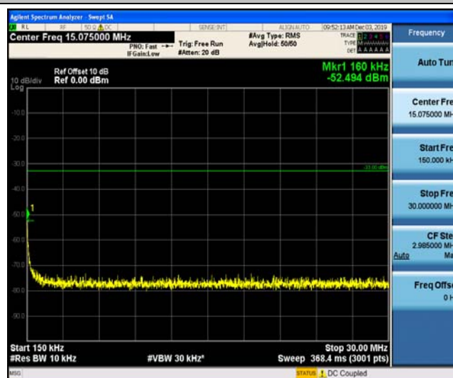
Band66_3MHz_16QAM_131987_1RB#0
