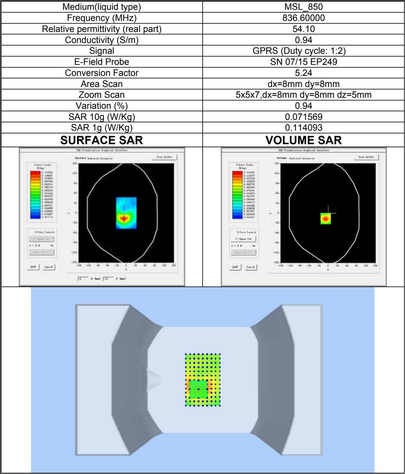
Plot 8: GPRS850MHz, Mid channel (Body-worn, Bottom edge) Product Description: Mobile Phone Test Date: 2018-05-30
