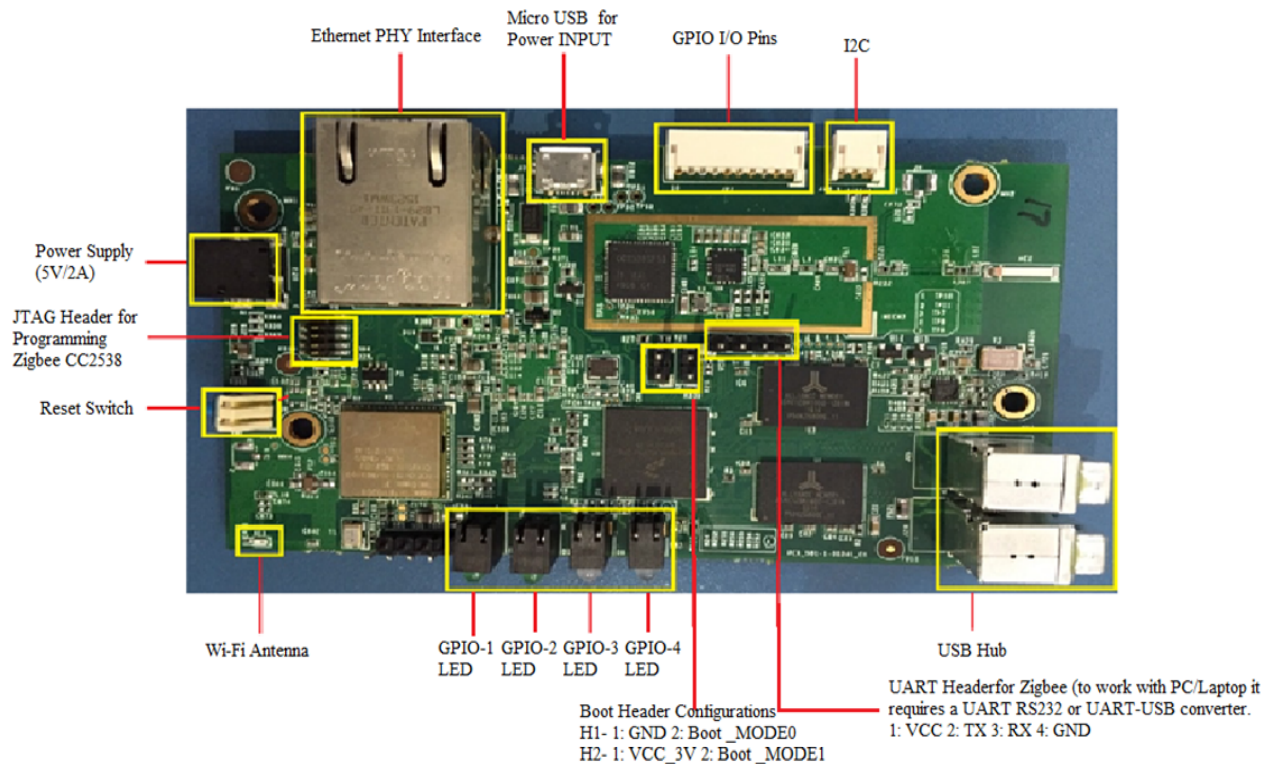
Fig 2: Board Details
