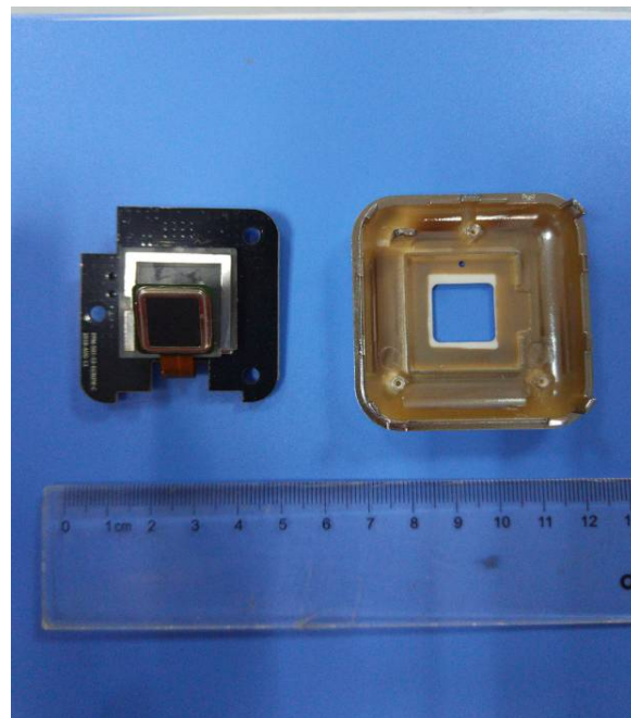
EUT – Cover off View 4
