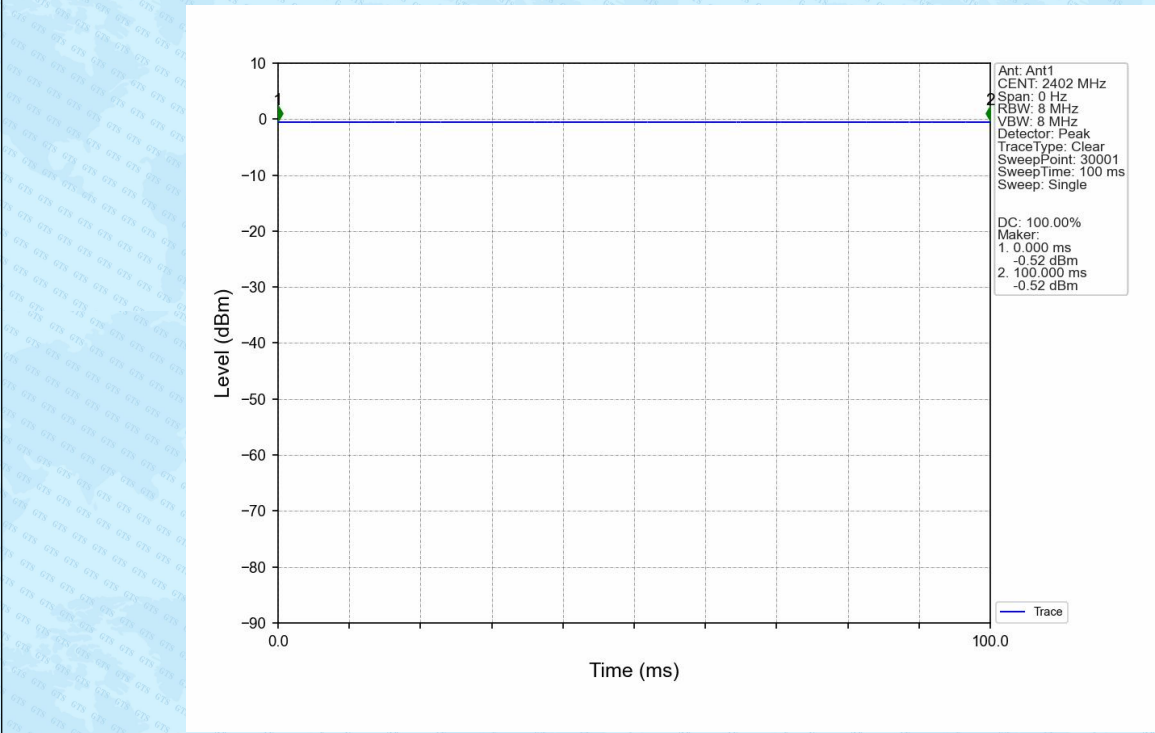
2M_LCH_2402MHz_Ant1_NTNV
