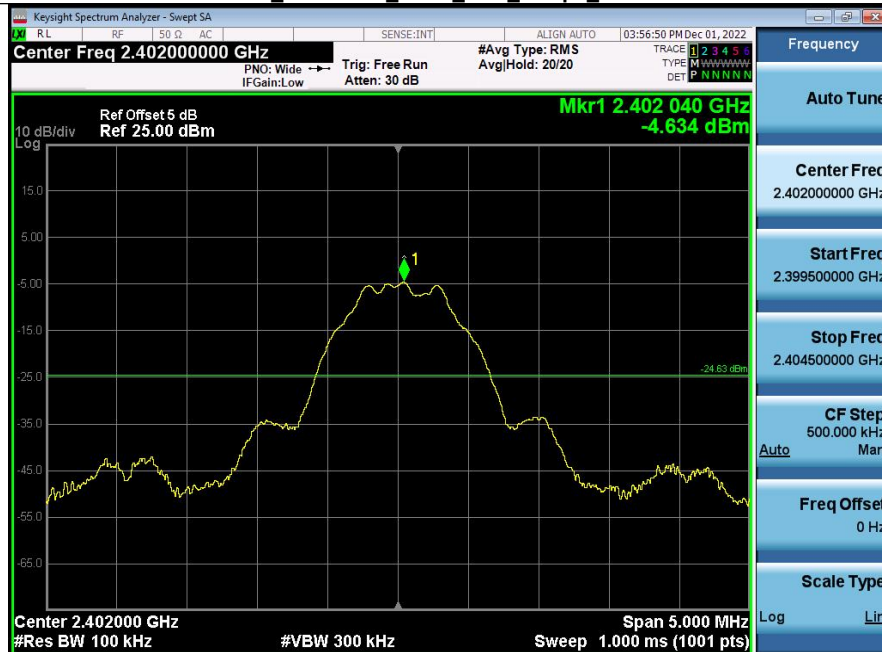
2 Spurious Emission_BLE_1Mbps_2402
