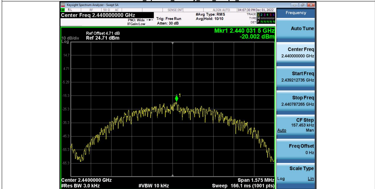
Power_Spectral_Density_BLE_1Mbps_2440
