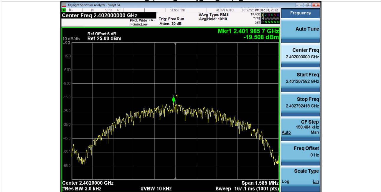
Power_Spectral_Density_BLE_1Mbps_2402
