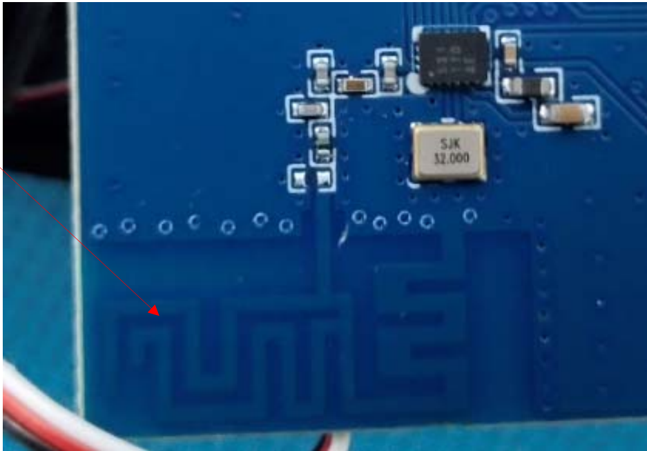
BT PCB Antenna
