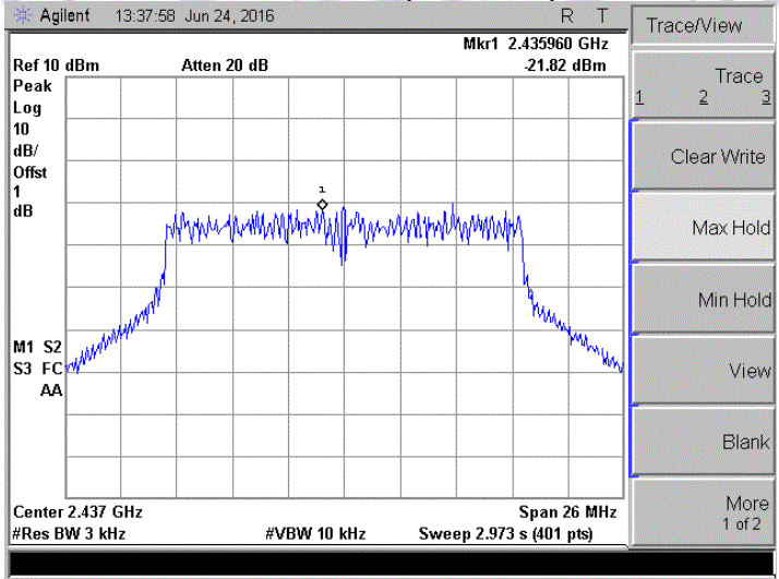
Channel 06 (2437MHz)
