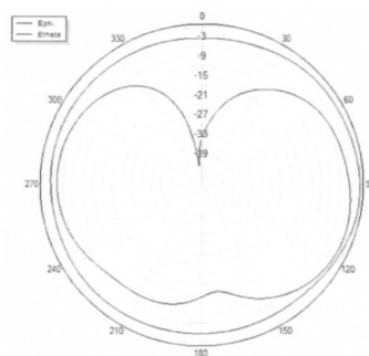
Theta=90 freq=2450MHz
