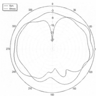
Phi=90 freq=2450MHz
