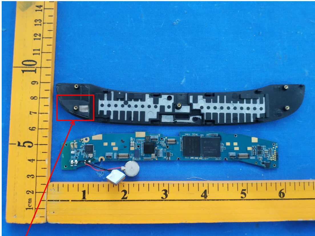
Internal Antenna
