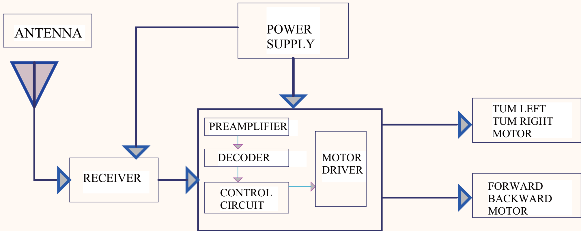
RX BLOCK DIAGRAM
