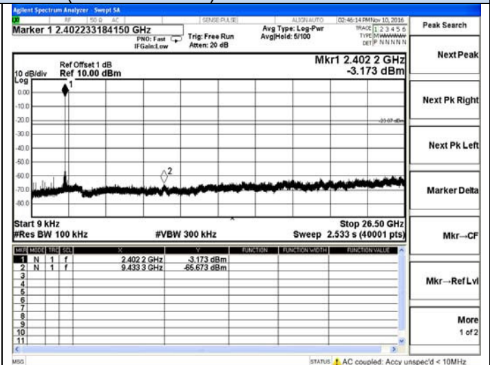
GFSK-Low channel
