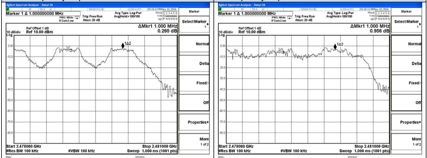
Frequency Separation GFSK-High channel
