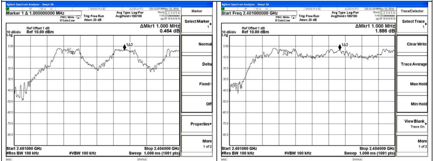
Frequency Separation GFSK-Low channel
