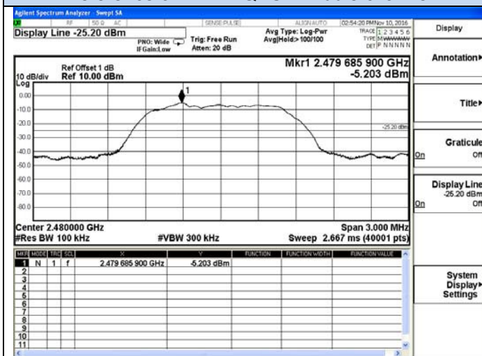
Reference of \pi/4 -DQPSK-High channel
