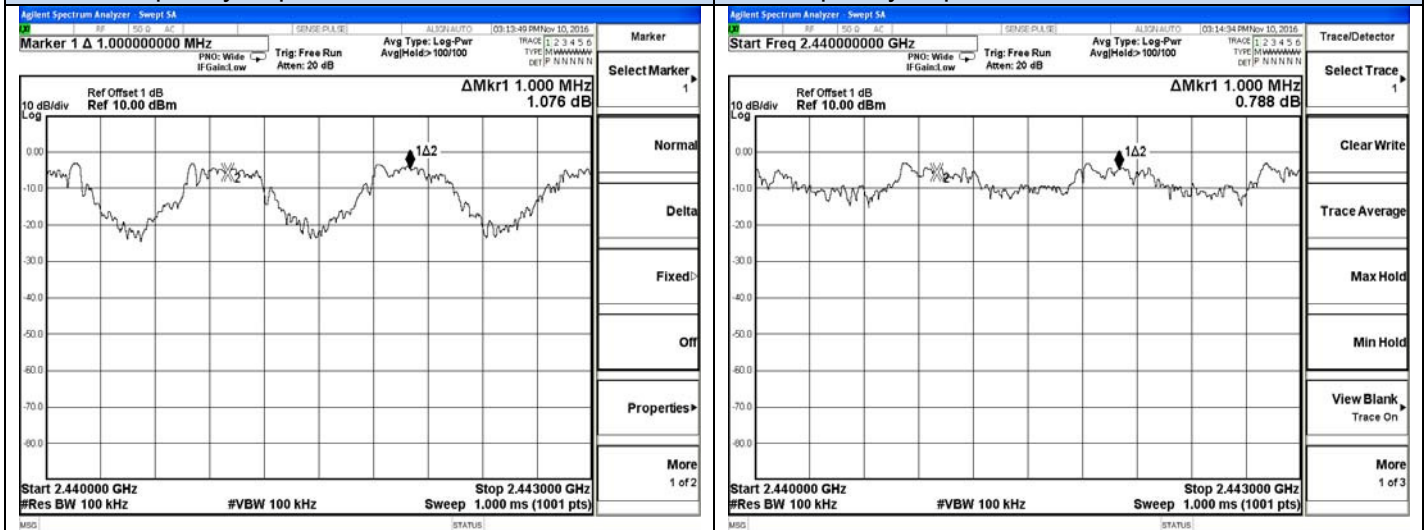
Frequency Separation GFSK-Middle channel
