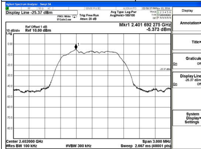
Reference of \pi/4 -DQPSK-Low channel
