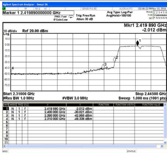
802.11n(HT40)-Low channel(Peak)
