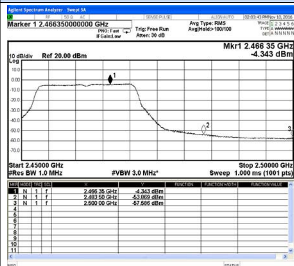
802.11n(HT20)-High channel(Average)
