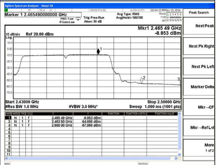
802.11n(HT40)-High channel(Average)
