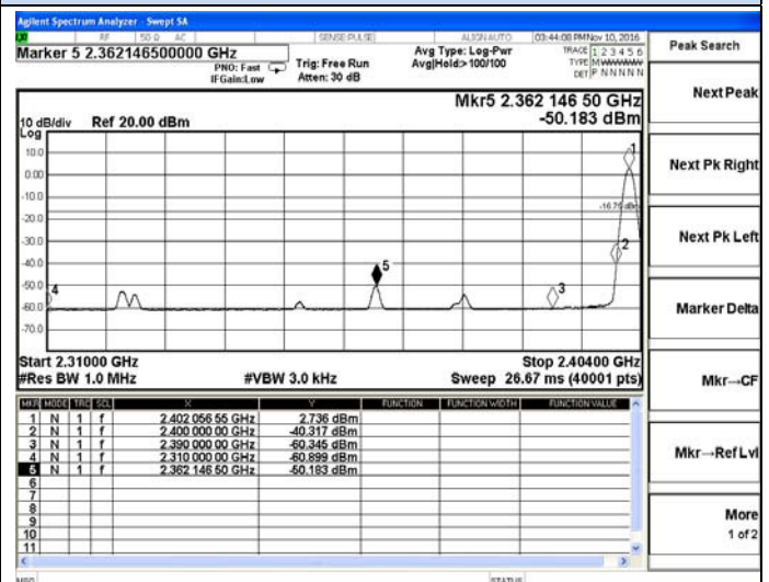
BT LE-Low channel(Average)
