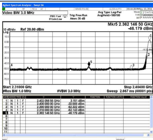
BT LE-Low channel(Peak)
