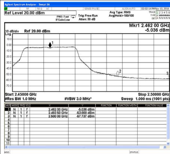
802.11g-High channel(Average)
