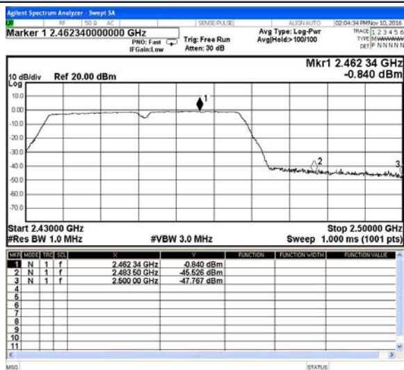
802.11n(HT40)-High channel(Peak)
