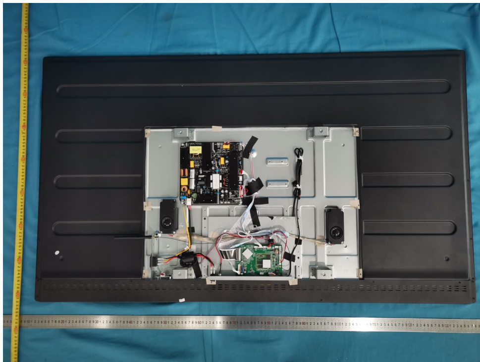
Internal Structure 2
