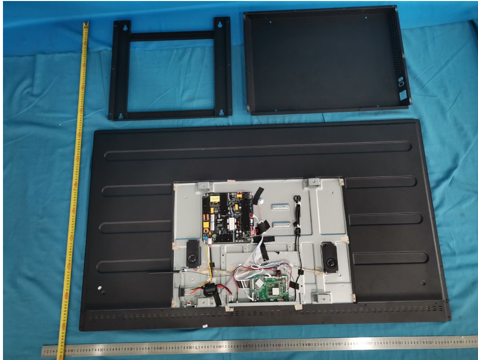
Internal Structure 1
