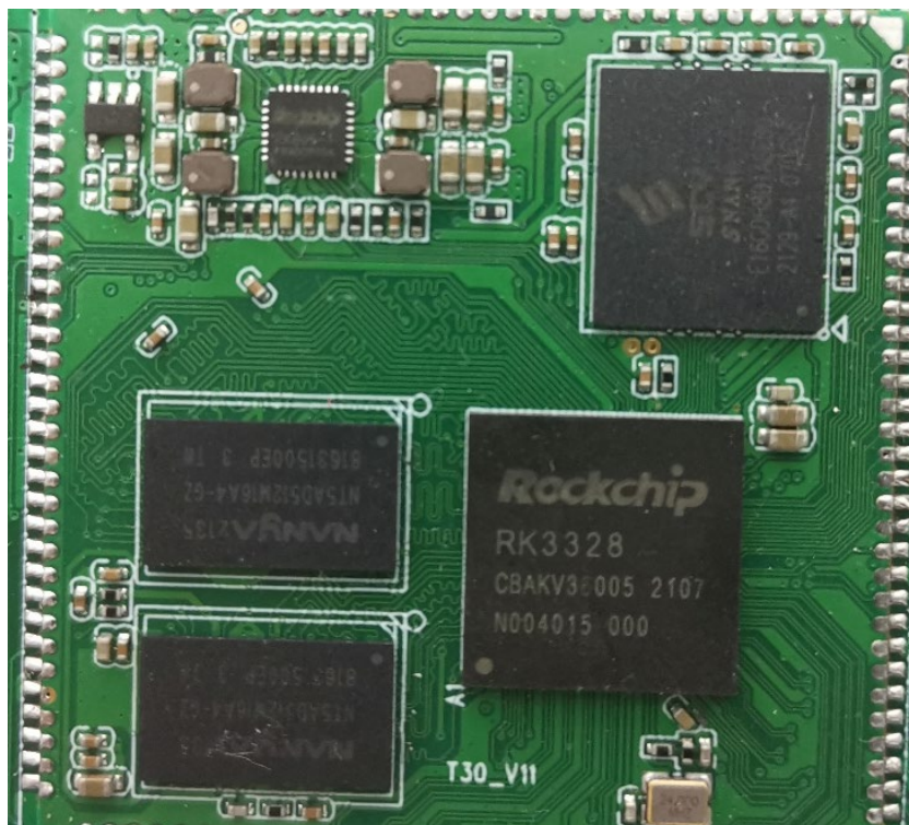
Mainboard Front 2
