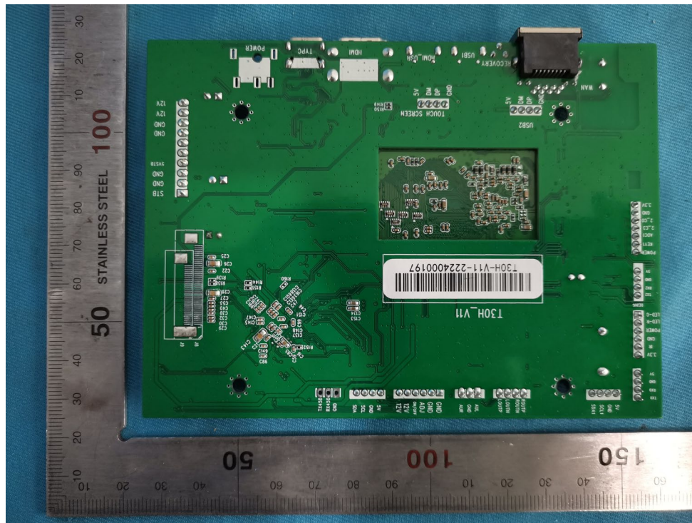
Mainboard Back
