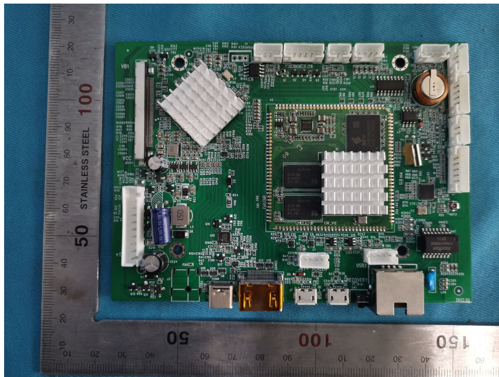
Mainboard Front 1
