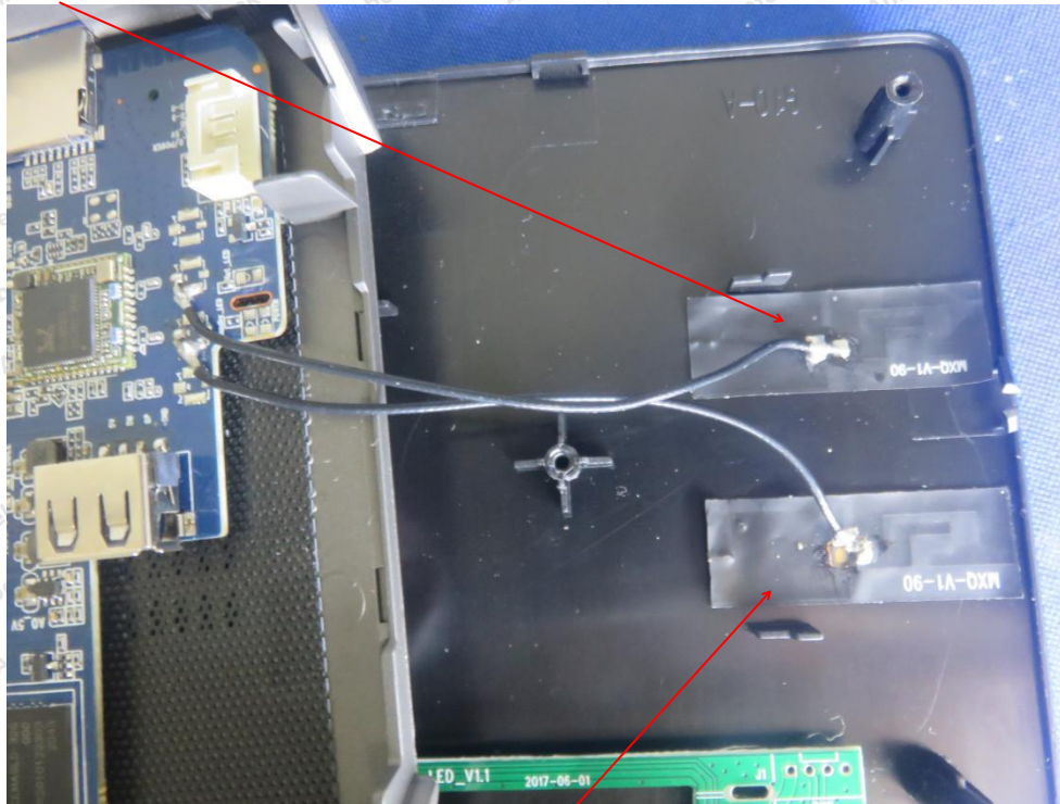
Wifi ANT A
