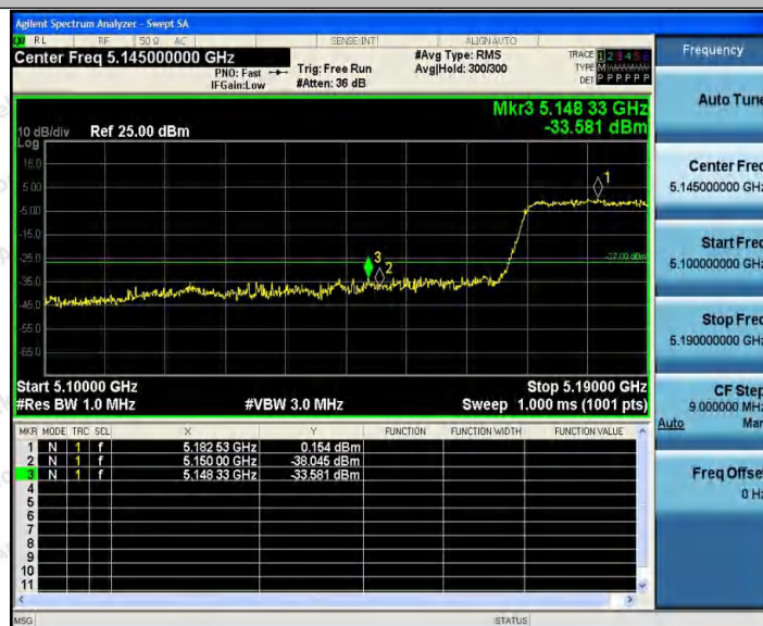
11AC80SISO_Ant1_High_5210
