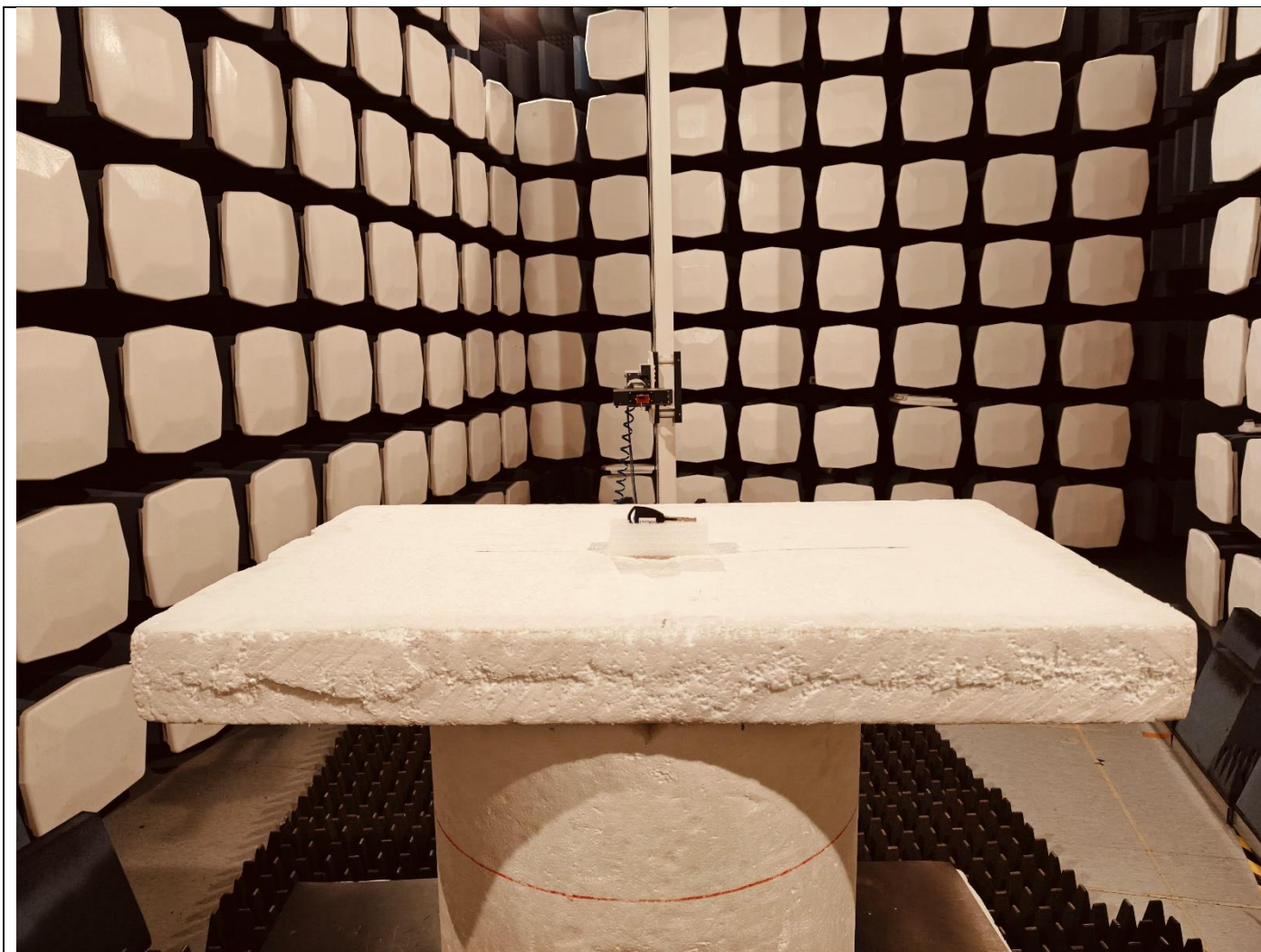
Picture 14, Radiated Spurious Emissions, EUT setup back, TX 18 – 26 GHz
