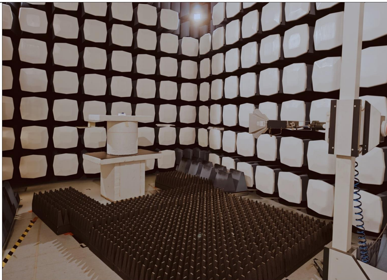
Picture 9, Radiated Spurious Emissions, common setup, TX 1 – 18 GHz and RX 1 – 12,75 GHz
