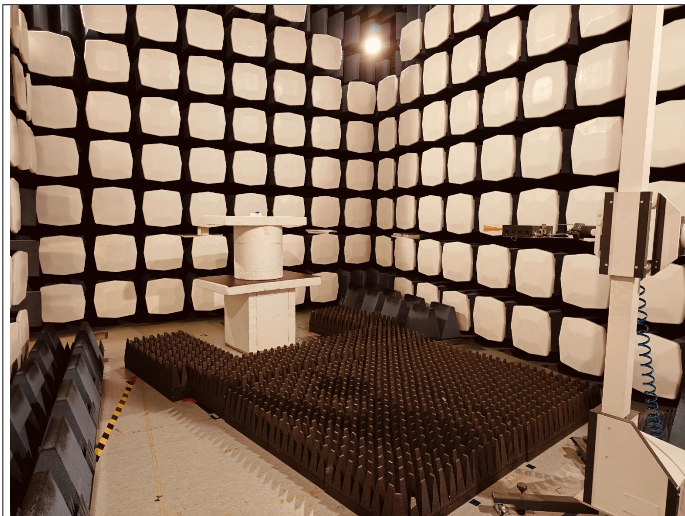
Picture 12, Radiated Spurious Emissions, common setup, TX 18 – 26 GHz
