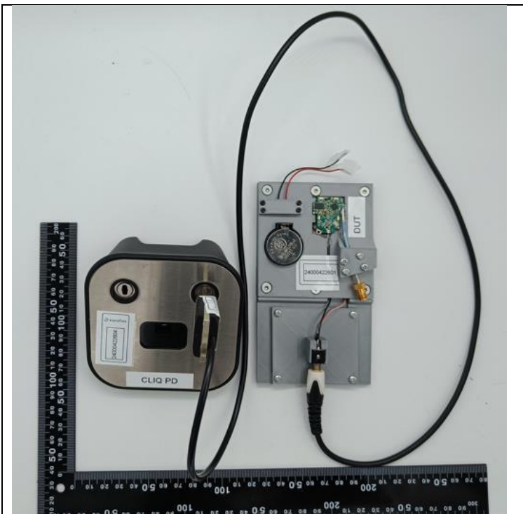
Picture 3, Conducted RF EUT with auxiliary equipment
