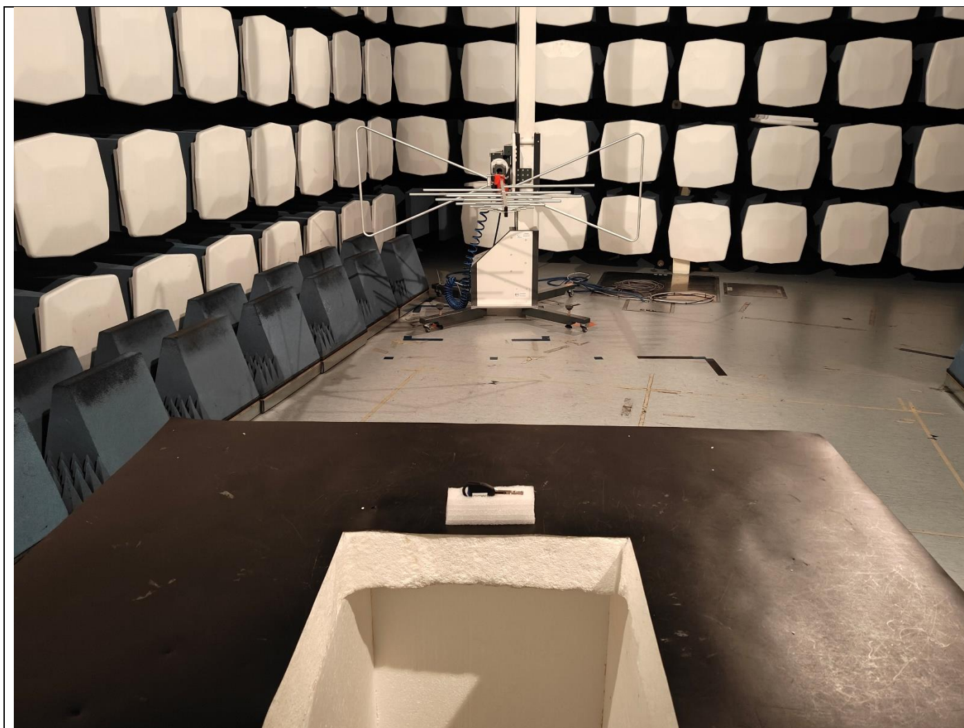
Picture 8, Radiated Spurious Emissions, EUT setup back, TX 30 – 1000 MHz and RX 30 – 1000 MHz
