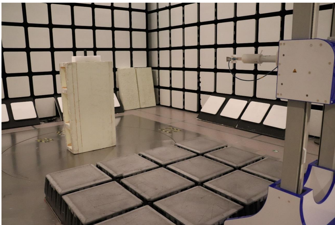
Photograph 6: Test setup for radiated tests (18 – 25 GHz)
