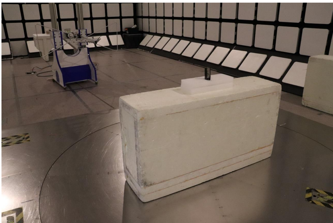
Photograph 4: Test setup for radiated tests (30 – 1000 MHz)
