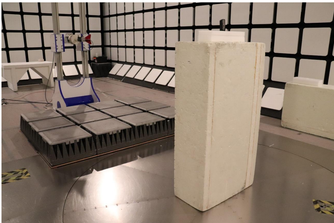
Photograph 5: Test setup for radiated tests (1 – 18 GHz)
