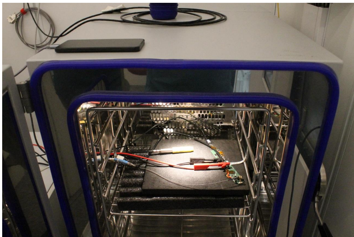
Photograph 2: Test setup for conducted tests
