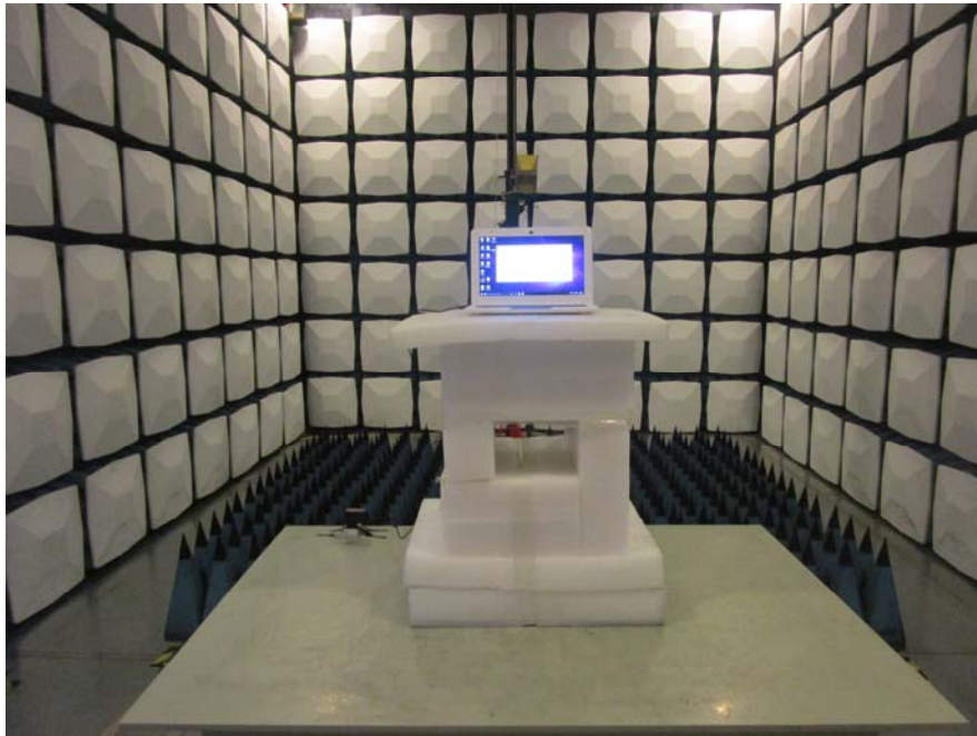
Radiated Emission View (Above 1GHz) (Adapter #2)
