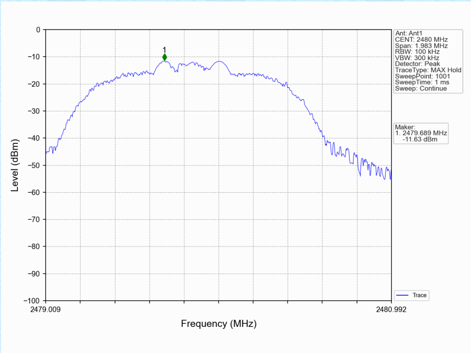
8DPSK_3DH5_HCH_2480MHz_Ant1_NTNV
