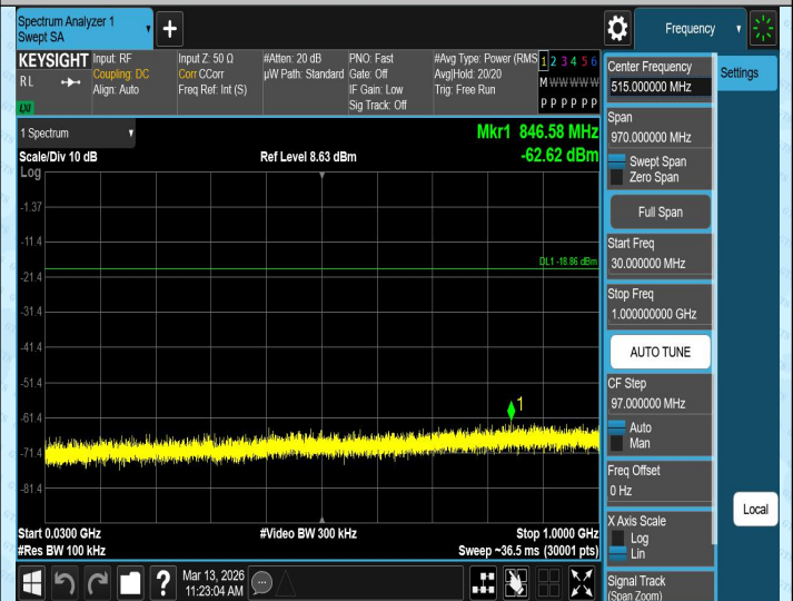
BLE_1M-Ant1-2480-30~1000-PASS
