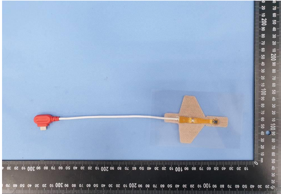
EUT Photo (16) _Adult/Pediatric Disposable Oximeter Sensor Cable
