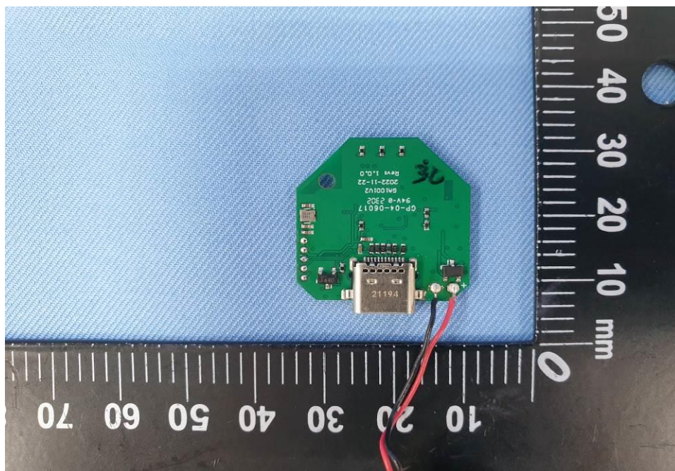
EUT Photo (11)
