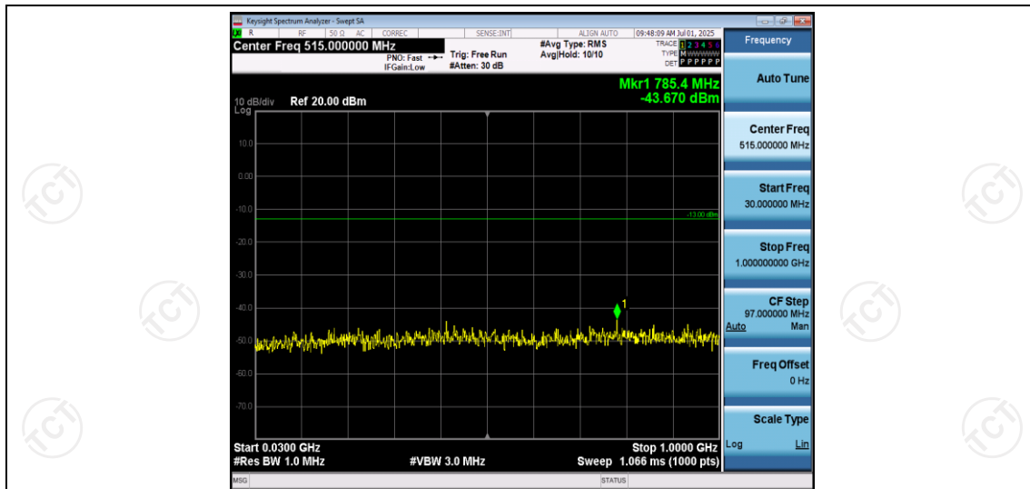
Band2-1.4MHz-QPSK-18607-1RB#0-Range1:30~1000MHz
