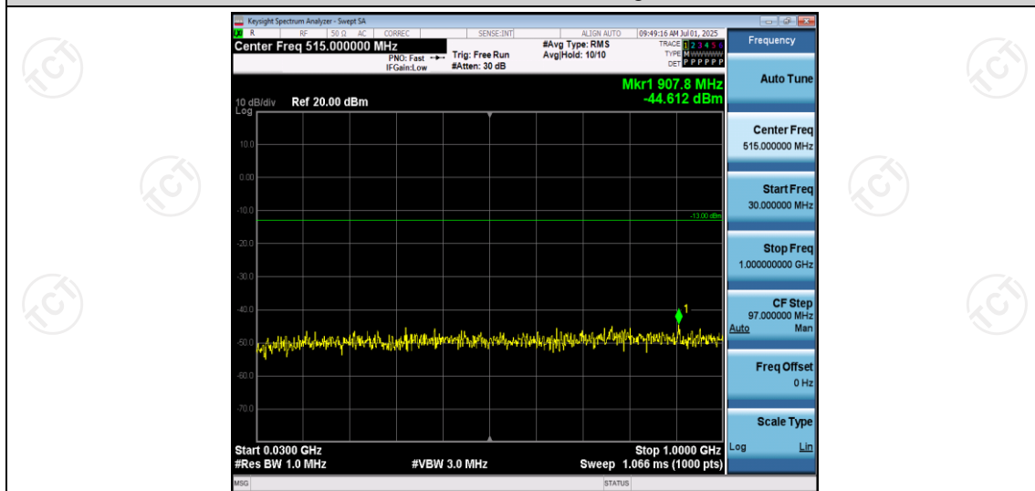
Band2-1.4MHz-QPSK-18900-1RB#0-Range1:30~1000MHz
