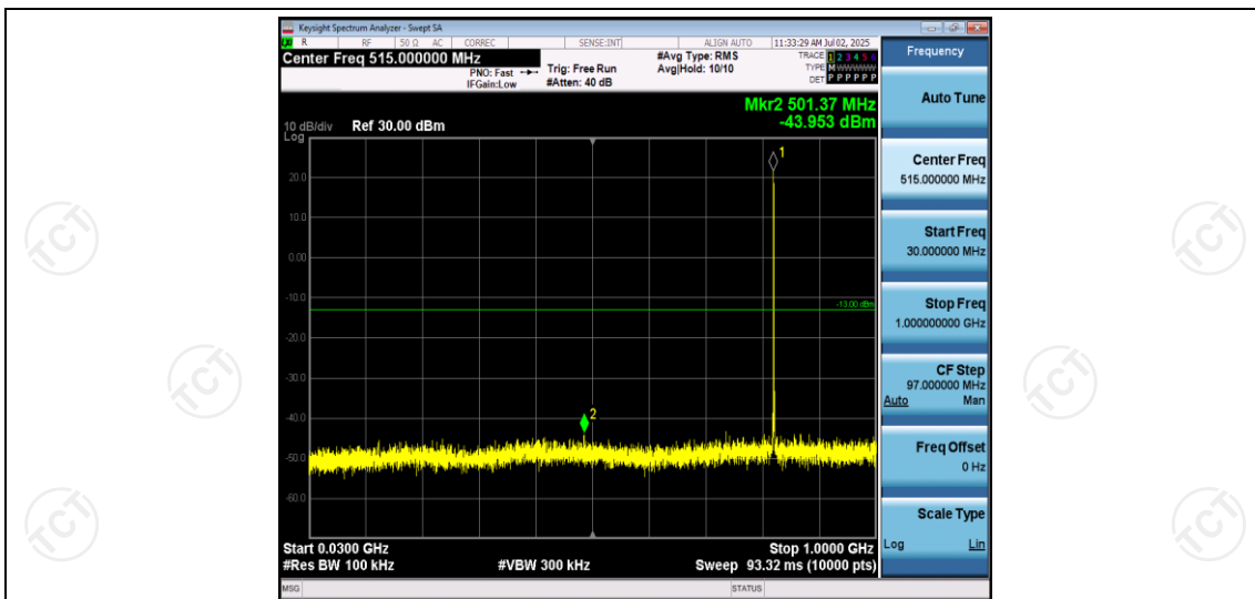
Band5-1.4MHz-QPSK-20407-1RB#0-Range1:30~1000MHz
