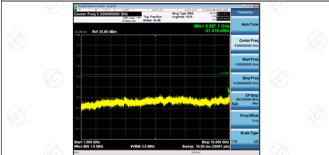
Band5-1.4MHz-QPSK-20407-1RB#0-Range2:1000~10000MHz
