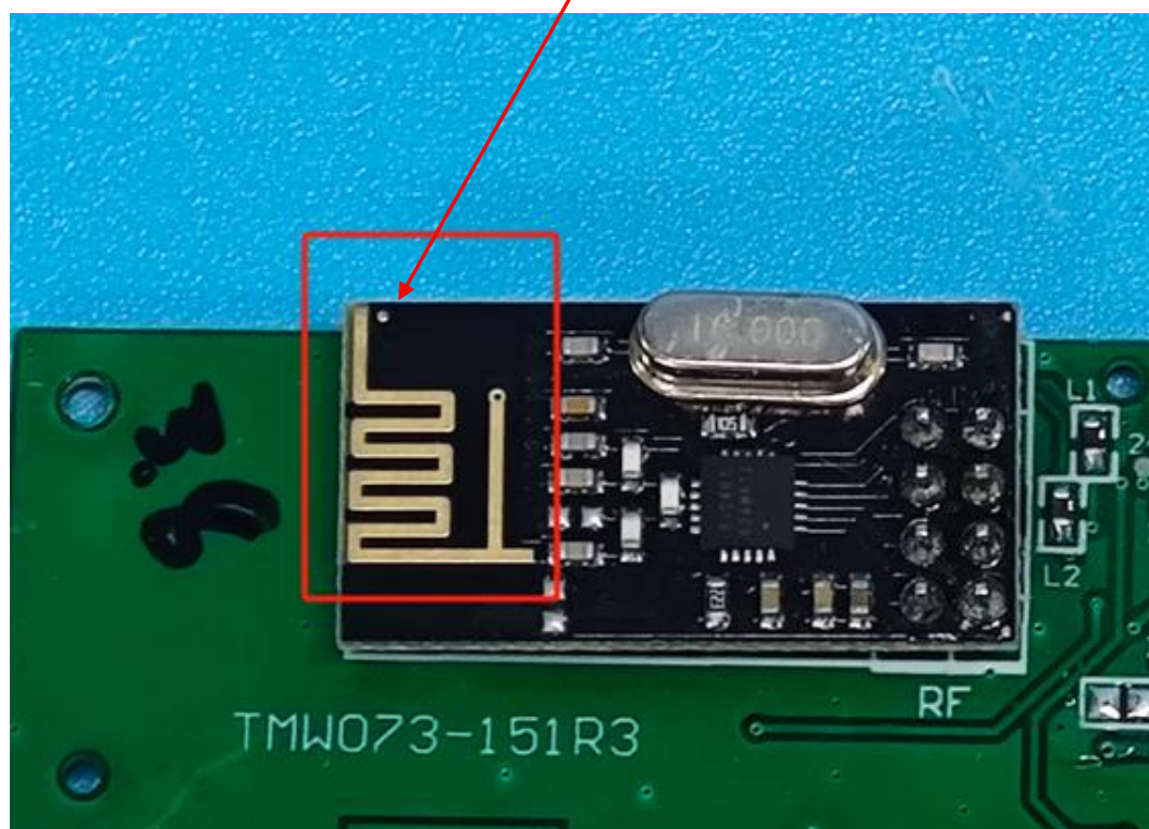
View of RF antenna
