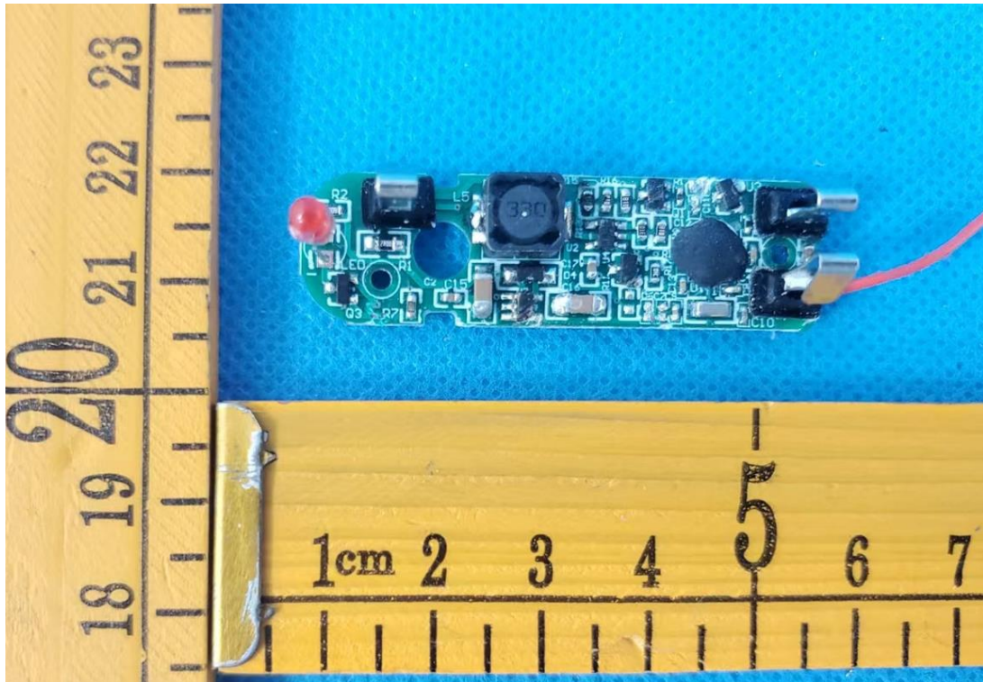
Inside View of the product
