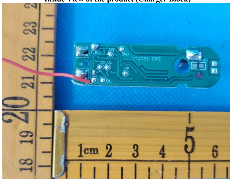
Inside View of the product (Charger Block)
