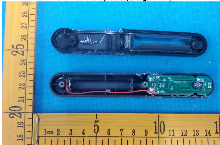
Inside View of the product (Charger Block)
