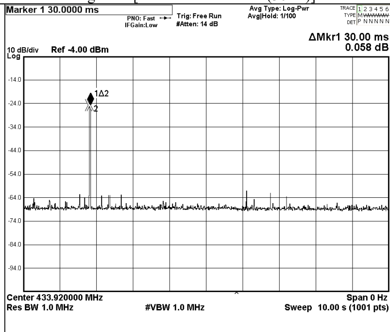
Figure B [Transmission Period(30ms)]
