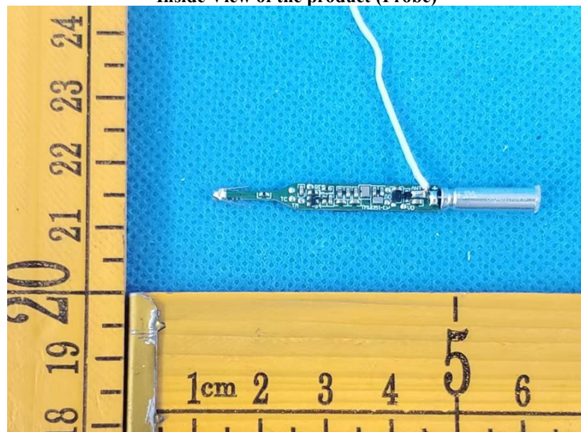
Inside View of the product (Probe)
