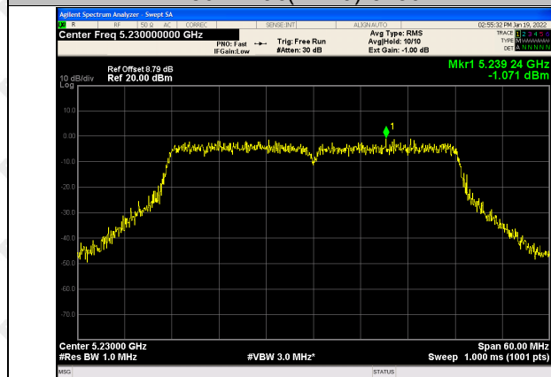
802.11ac(VH40)-5230
