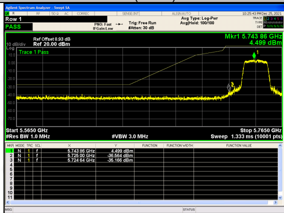
802.11ac(VH20)-5745
