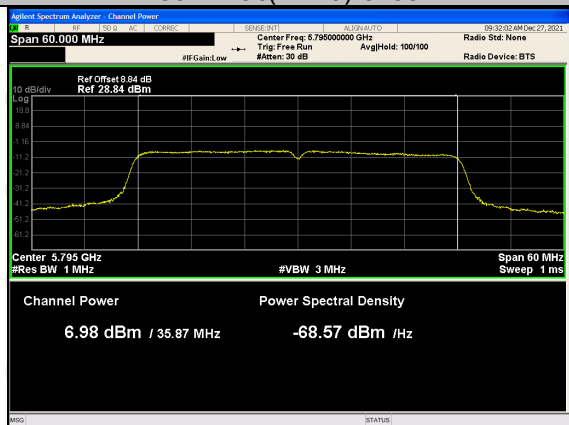
802.11ac(VH40)-5795
