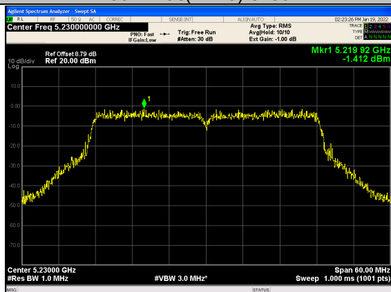
802.11ac(VH40)-5230
