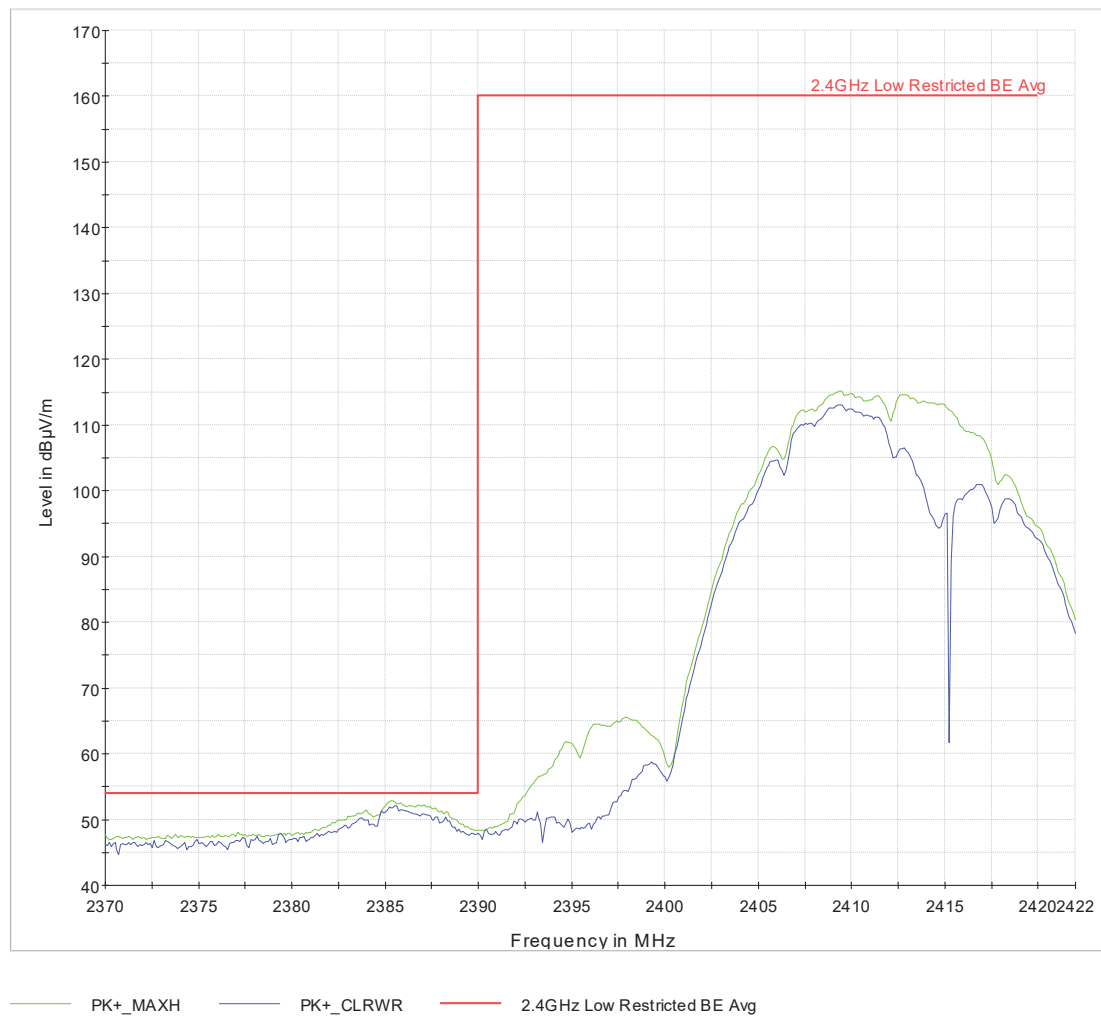
Figure 3 Low_Rest_BE_ch1_CCK_Tx=23.5_2x2_CDD_maximize
