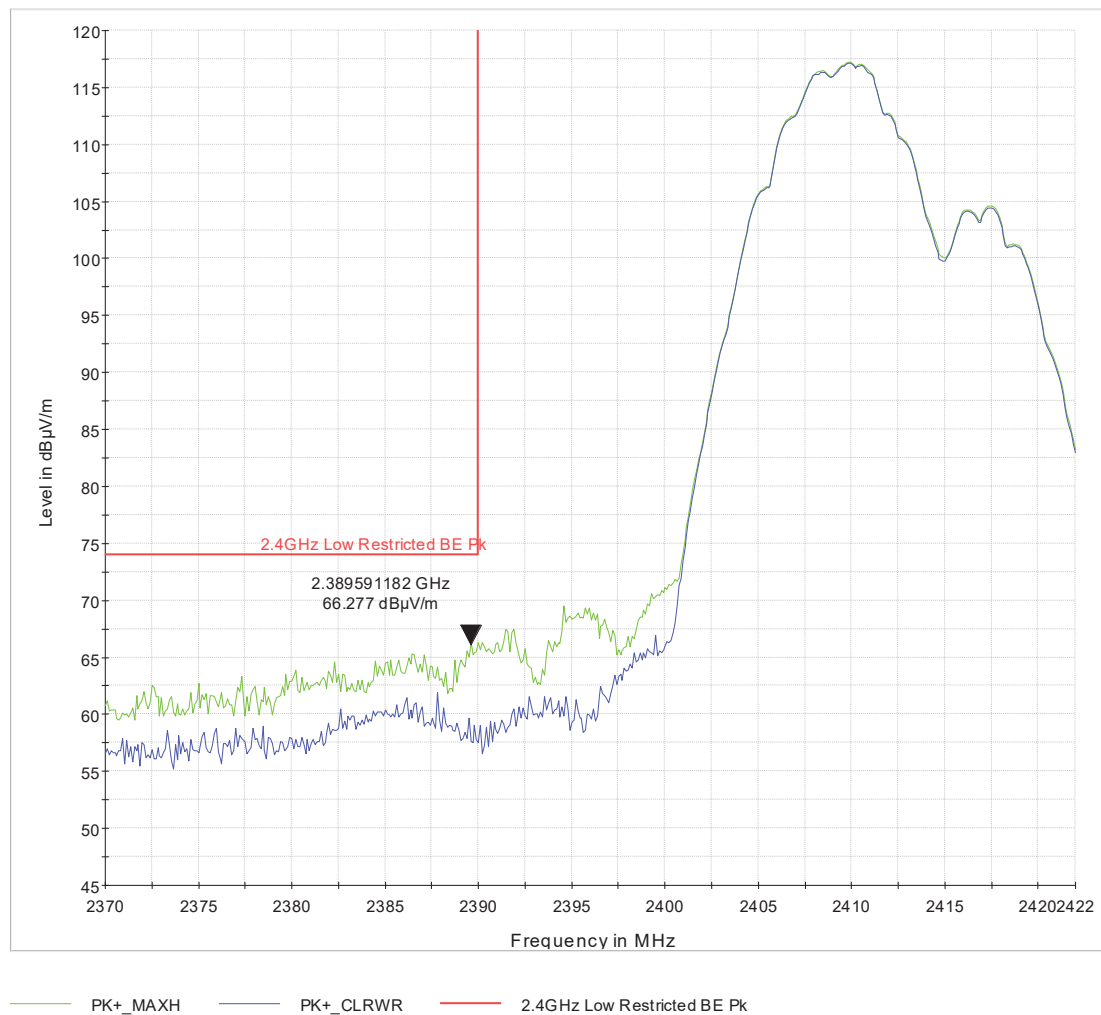
Figure 2 Low_Rest_BE_ch1_CCK_Tx=23.5_2x2_CDD_0deg_119cm_pk
