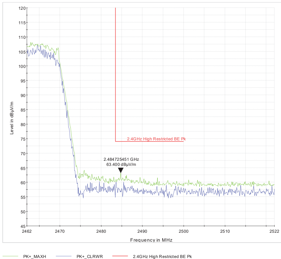
Figure 29 High_Rest_BE_ch9_HT40_Tx=14_2x2_BF_0deg_105cm_pk
