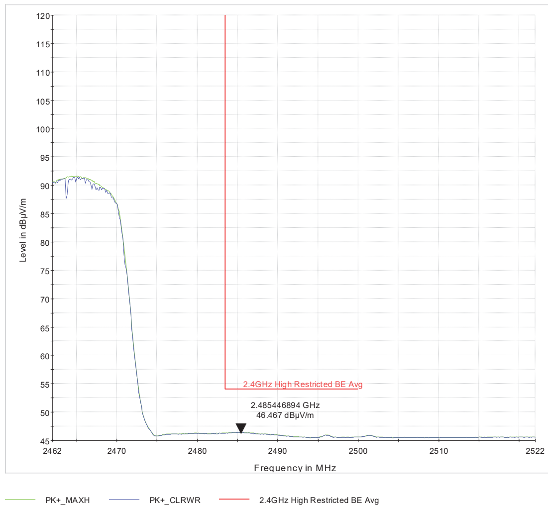
Figure 28 High_Rest_BE_ch9_HT40_Tx=14_2x2_BF_0deg_105cm_avg
