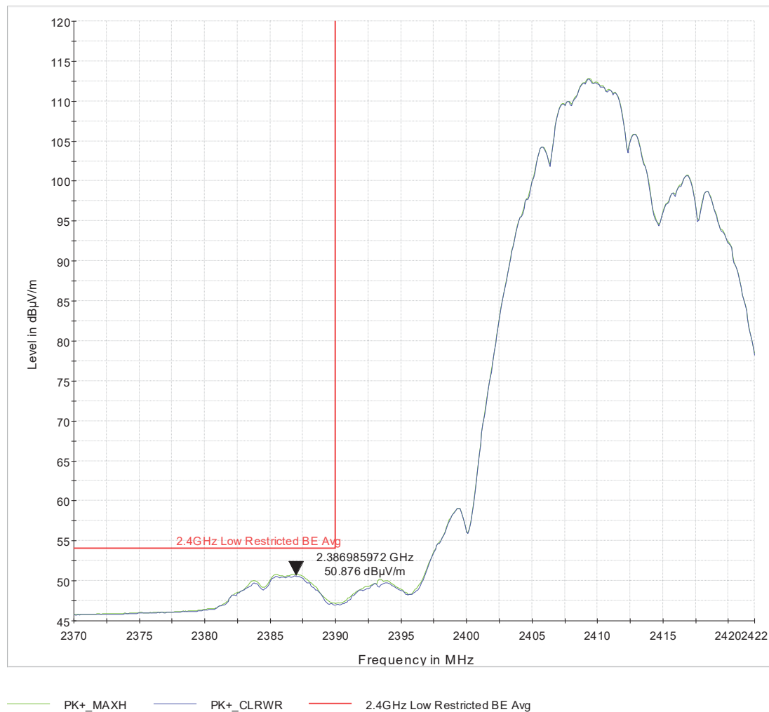
Figure 1 Low_Rest_BE_ch1_CCK_Tx=23.5_2x2_CDD_0deg_119cm_avg
