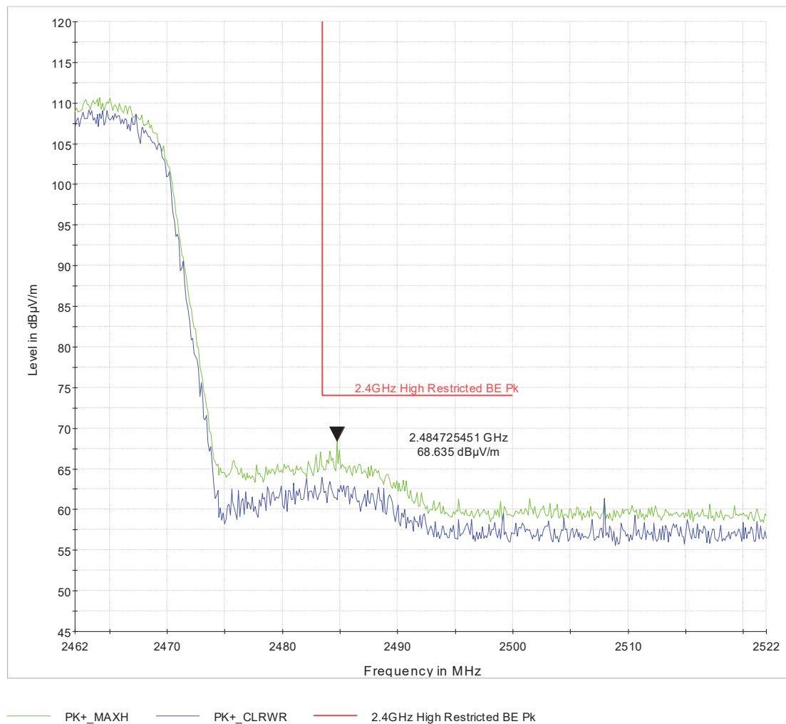
Figure 23 High_Rest_BE_ch9_HT40_Tx=14_2x2_CDD_360deg_124cm_pk
