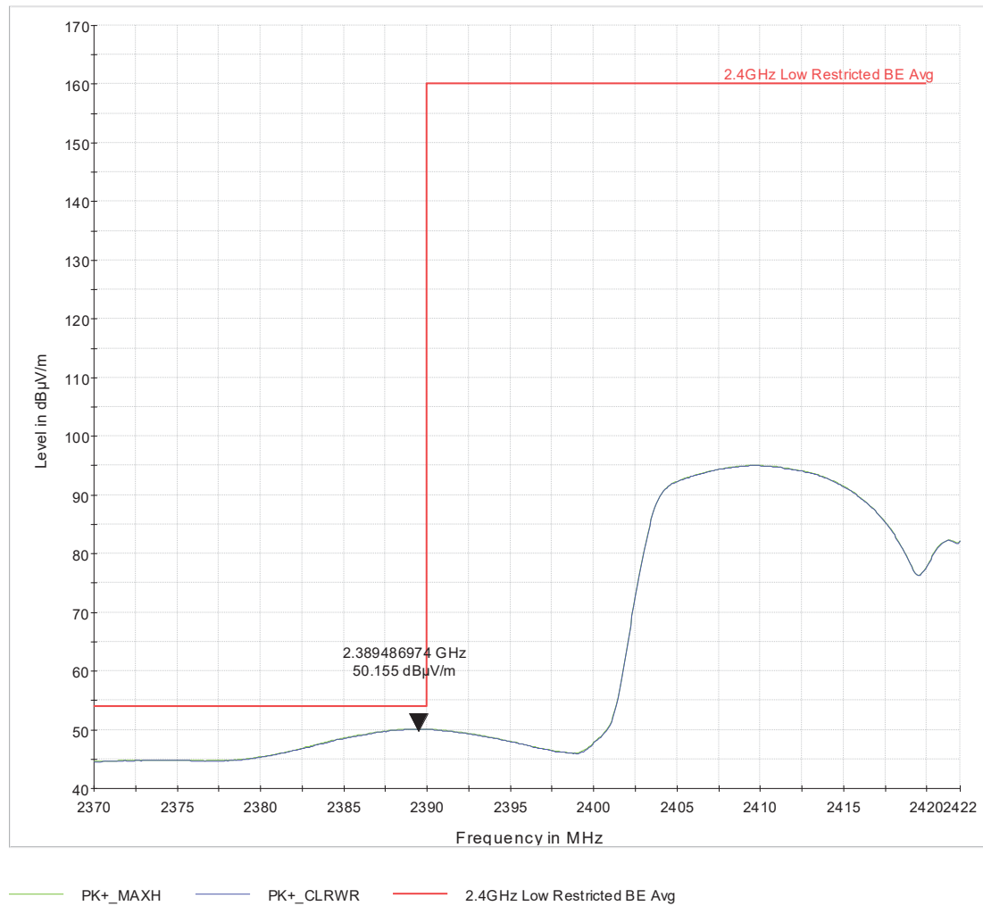
Figure 7 Low_Rest_BE_ch3_HT40_Tx=13.5_2x2_CDD_291deg_369cm_avg
