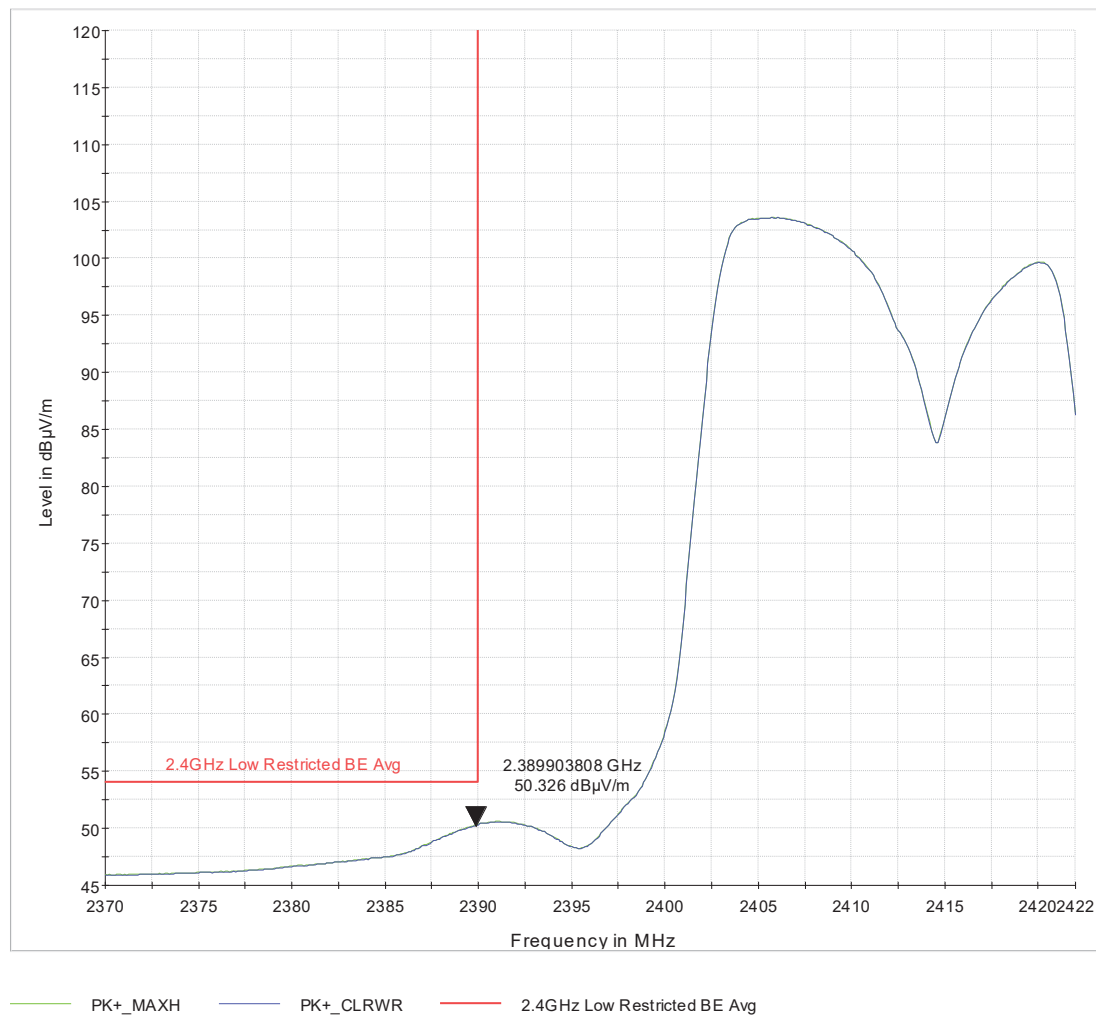
Figure 4 Low_Rest_BE_ch1_HT20_Tx=17_2x2_CDD_360deg_123cm_avg
