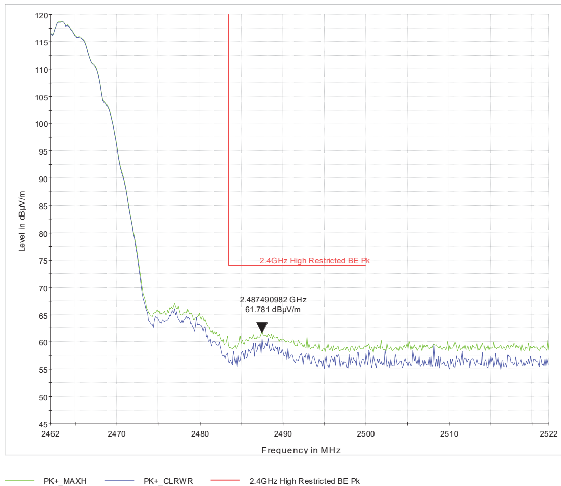
Figure 17 High_Rest_BE_ch11_CCK_Tx=24_2x2_CDD_278deg_189cm_V_pk
