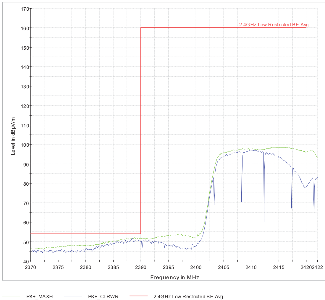
Figure 9 Low_Rest_BE_ch3_HT40_Tx=13.5_2x2_CDD_maximize
