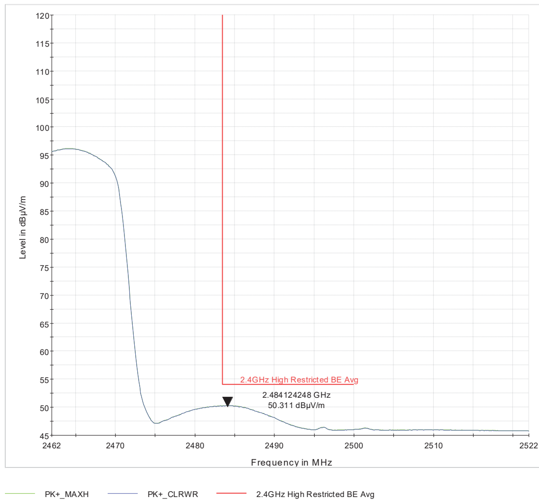
Figure 22 High_Rest_BE_ch9_HT40_Tx=14_2x2_CDD_360deg_124cm_avg
