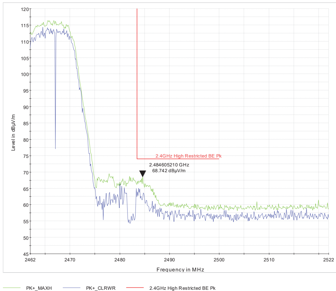
Figure 26 High_Rest_BE_ch11_VHT20_Tx=17_2x2_BF_284deg_192cm_V_pk
