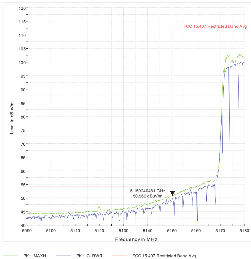
Figure 18 U-1_L-BE_ch38_VHT40_2x2_pwr=17_BF_maximize
