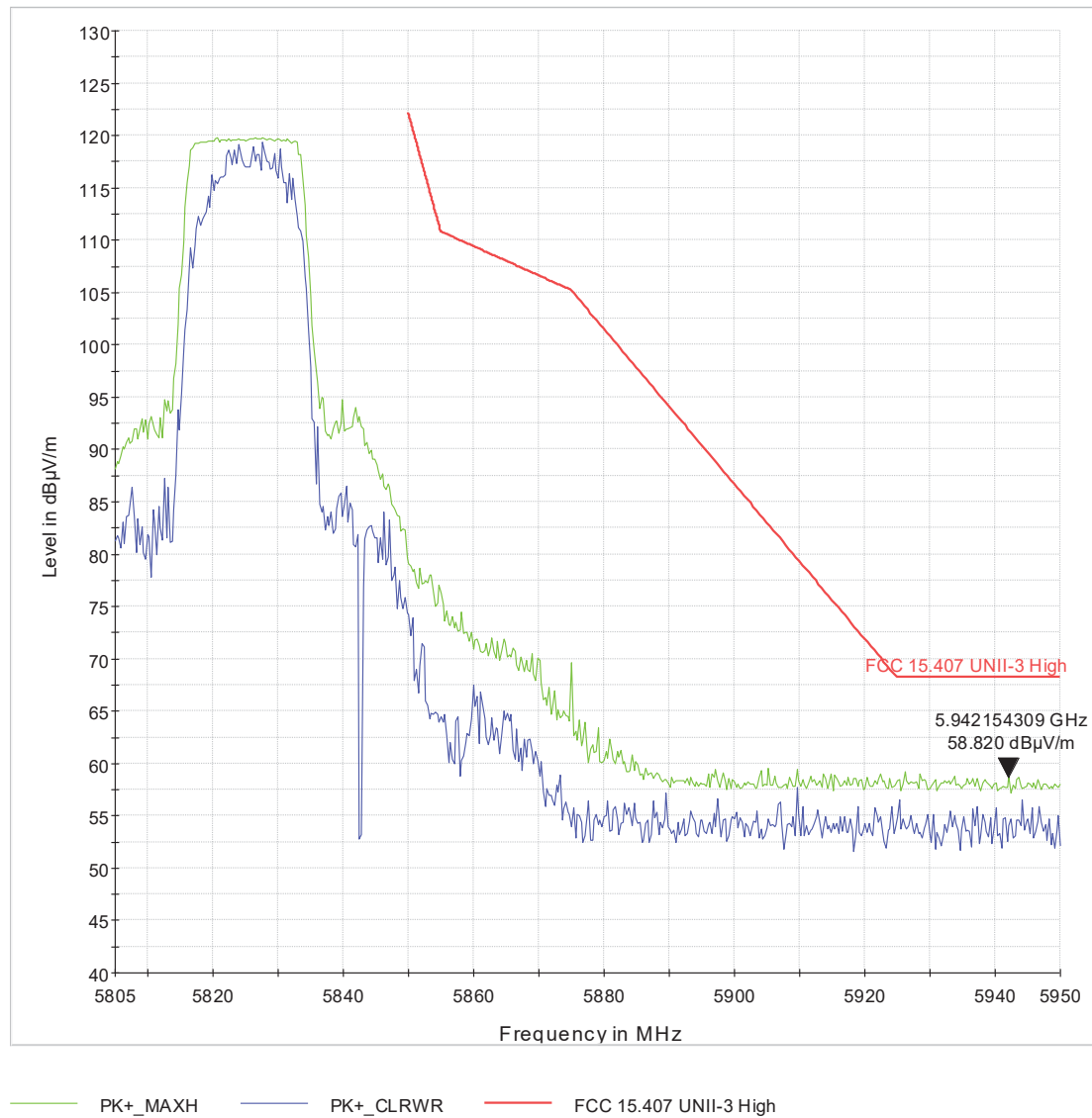
Figure 4 U-3_H-BE_ch165_HT20_2x2_pwr=25_125deg_150cm_V
