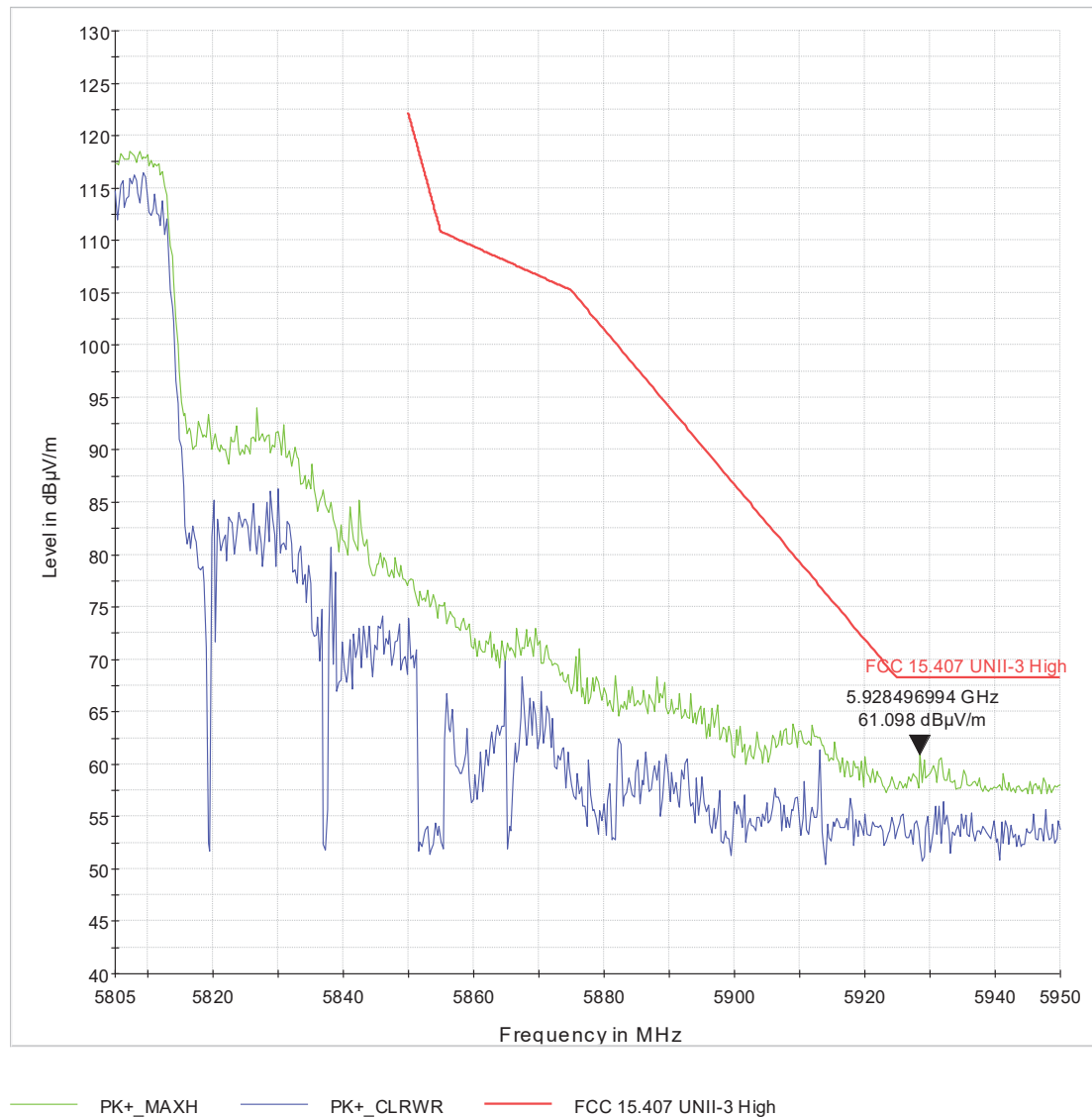
Figure 12 U-3_H-BE_ch159_VHT40_2x2_pwr=24_BF_137deg_250cm_V
