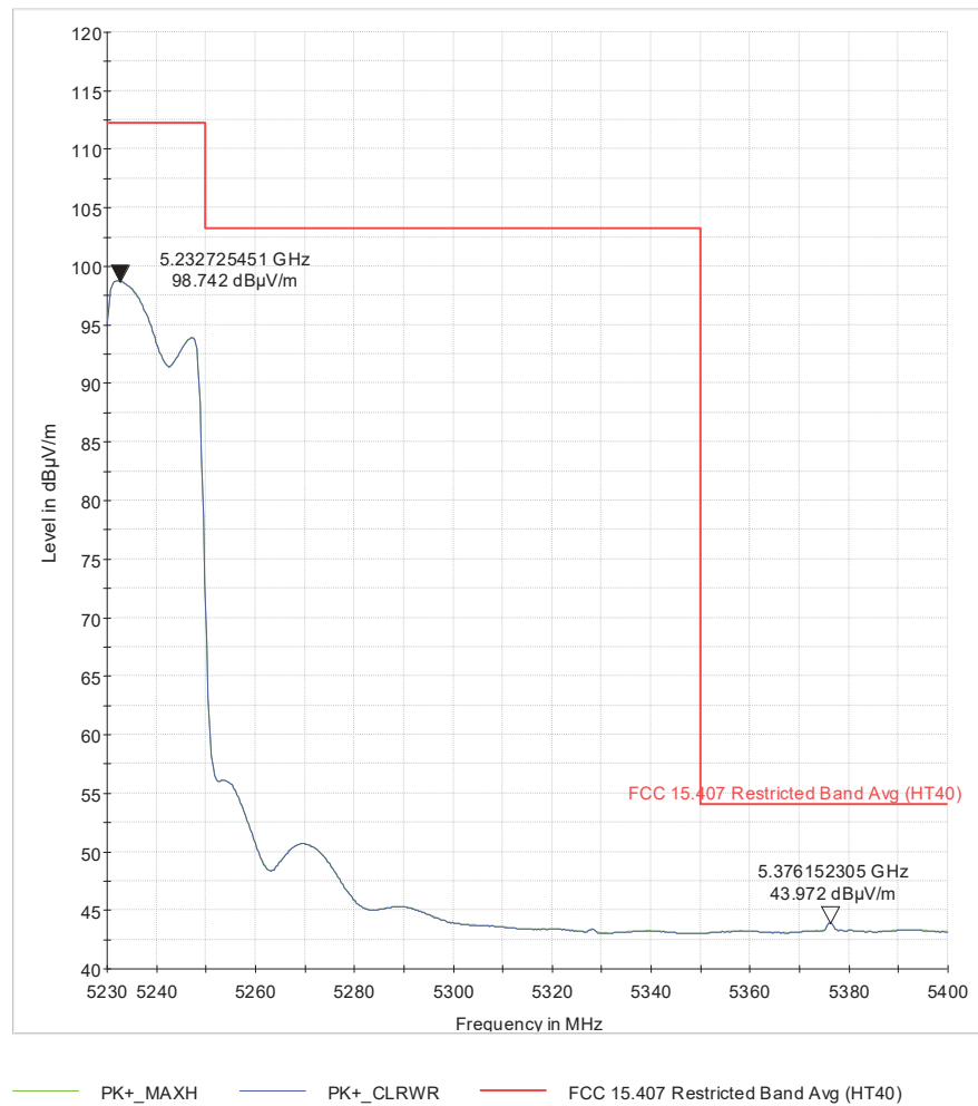
Figure 26 U-1_H_BE_HT40_ch46_pwr-17_2x2_CDD_234deg_150cm_V_avg
