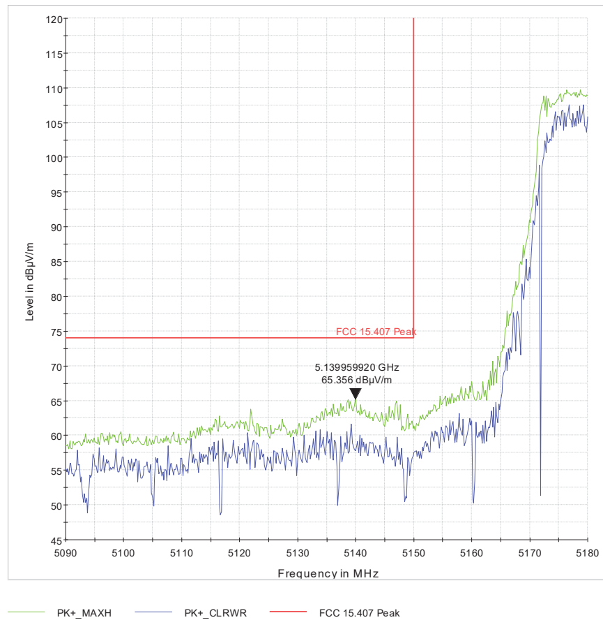
Figure 20 U-1_L-BE_ch42_VHT80_2x2_pwr=17_BF_228deg_178cm_H_pk
