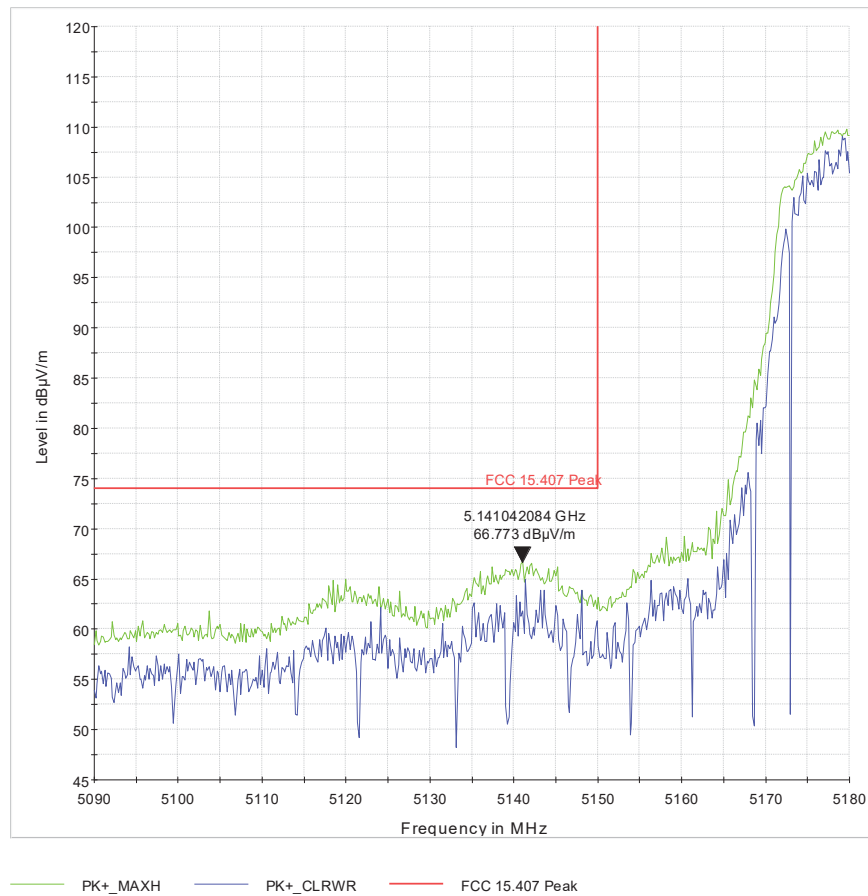
Figure 11 U-1_L-BE_ch42_VHT80_2x2_pwr=16.5_227deg_184cm_H_pk
