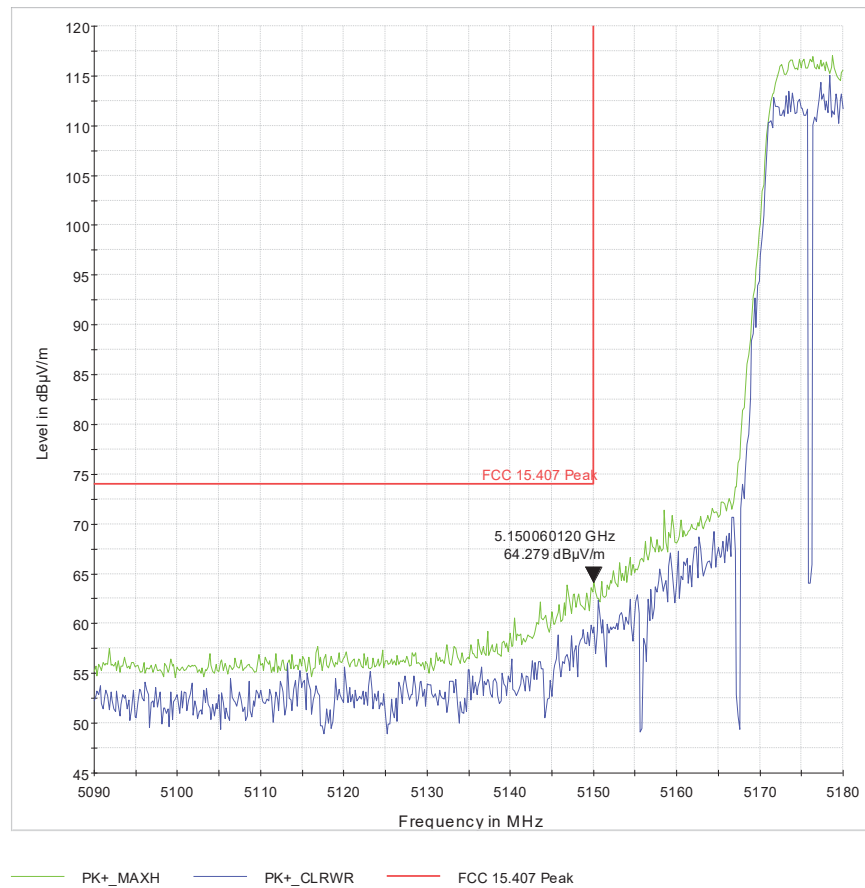
Figure 14 U-1_L-BE_ch36_VHT20_2x2_pwr=18_BF_218deg_209cm_H_pk
