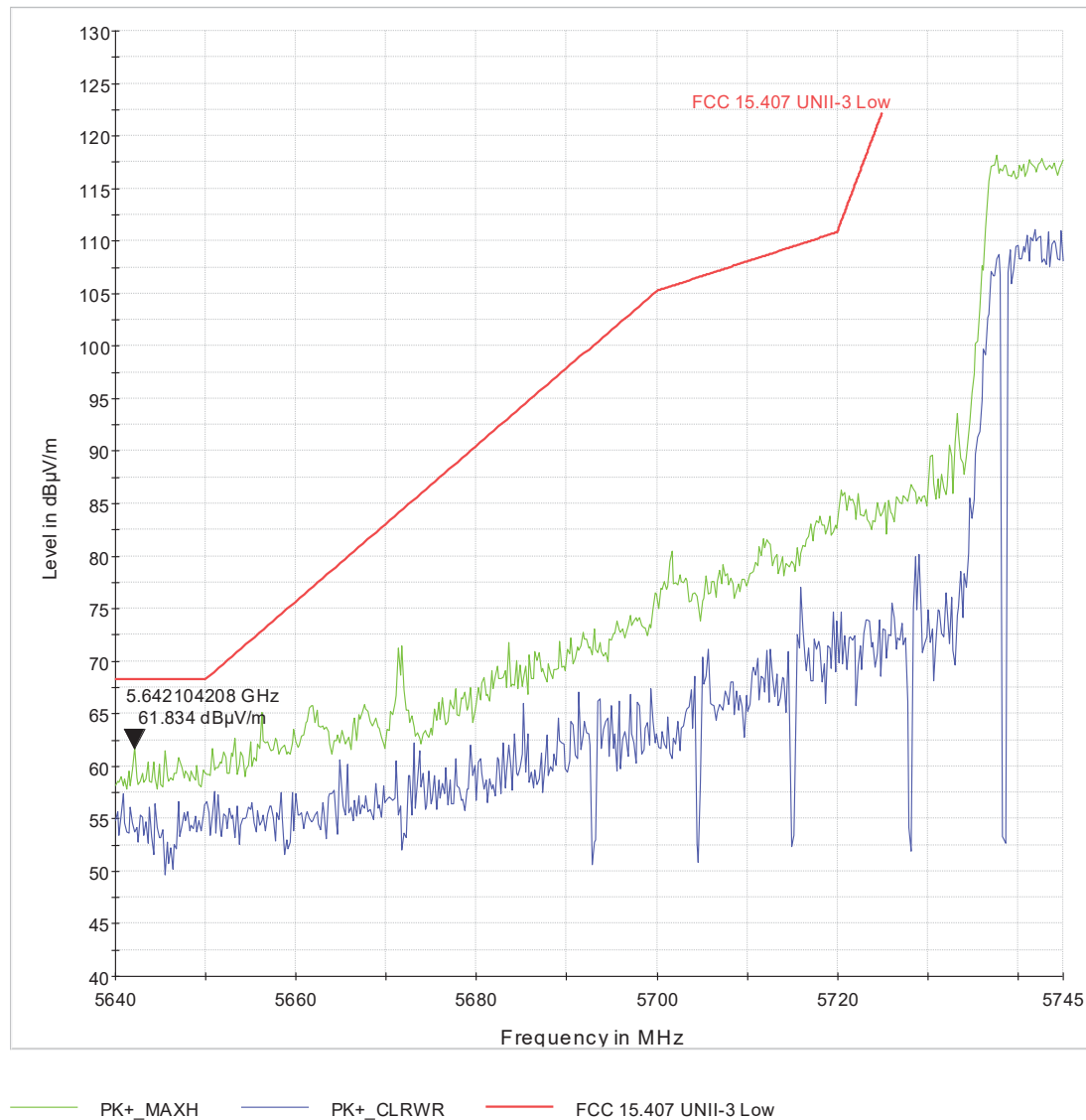
Figure 11 U-3_L-BE_ch151_VHT40_2x2_pwr=24_BF_230deg_134cm_H
