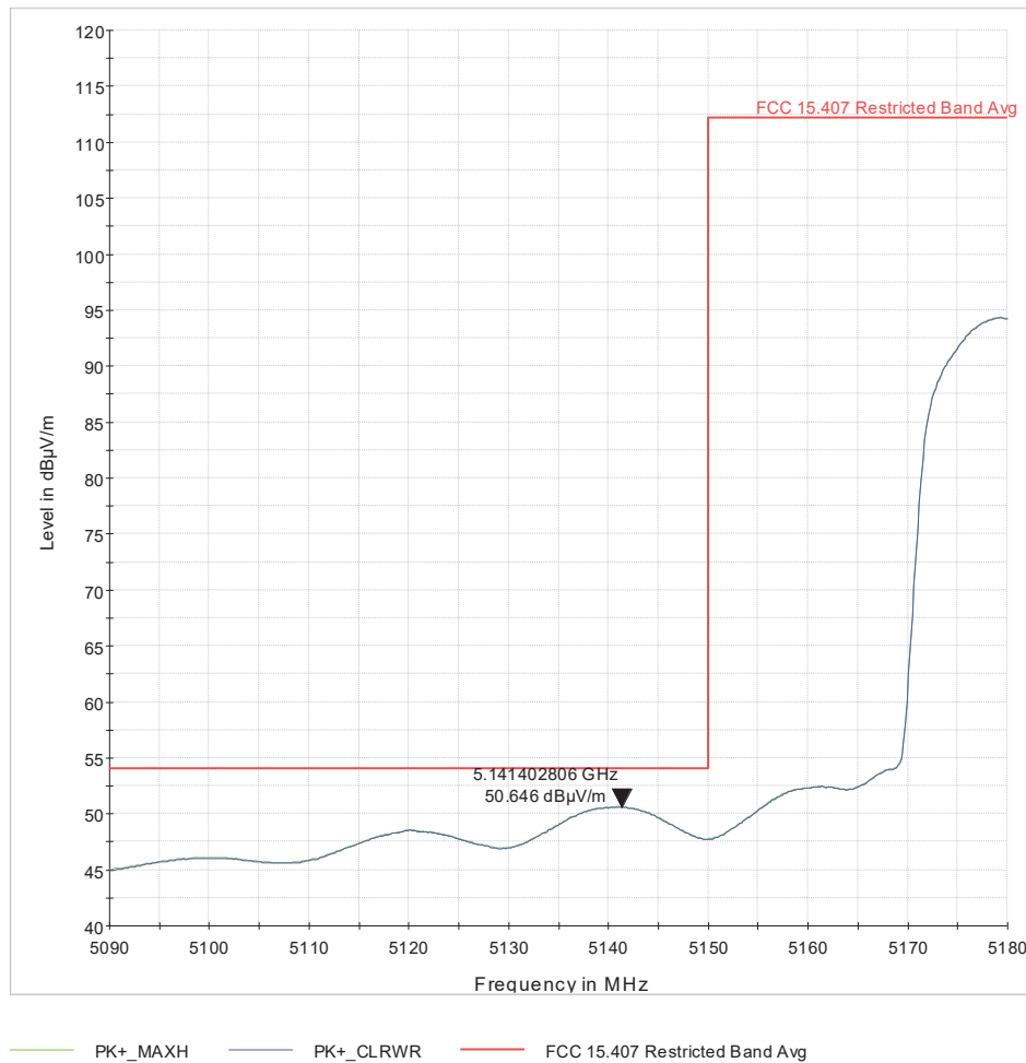
Figure 10 U- 1_L-BE_ch42_VHT80_2x2_pwr=16.5_227deg_184cm_H_avg
