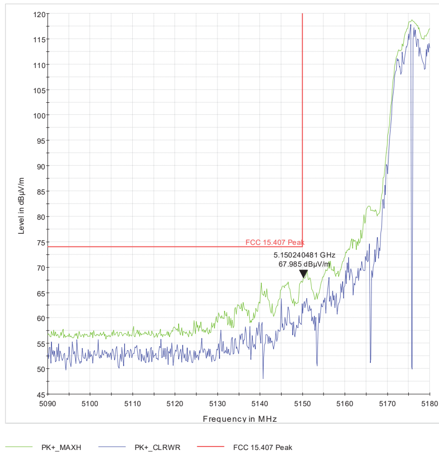
Figure 2 U-1_L-BE_ch36_NoHT_2x2_pwr=20.5_73deg_192cm_V_pk
