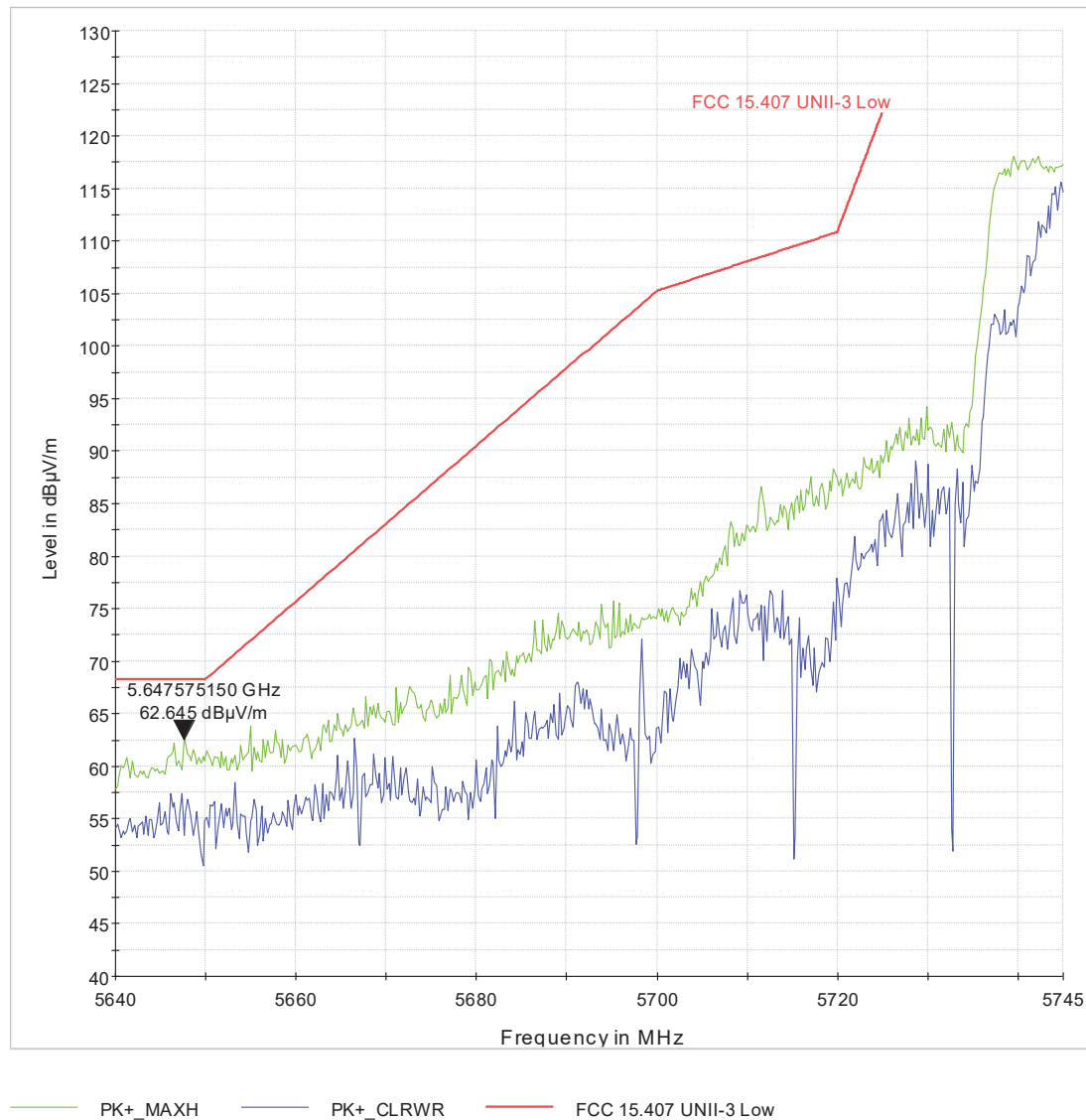
Figure 5 U-3_L-BE_ch151_HT40_2x2_pwr=24.5_132deg_250cm_V
