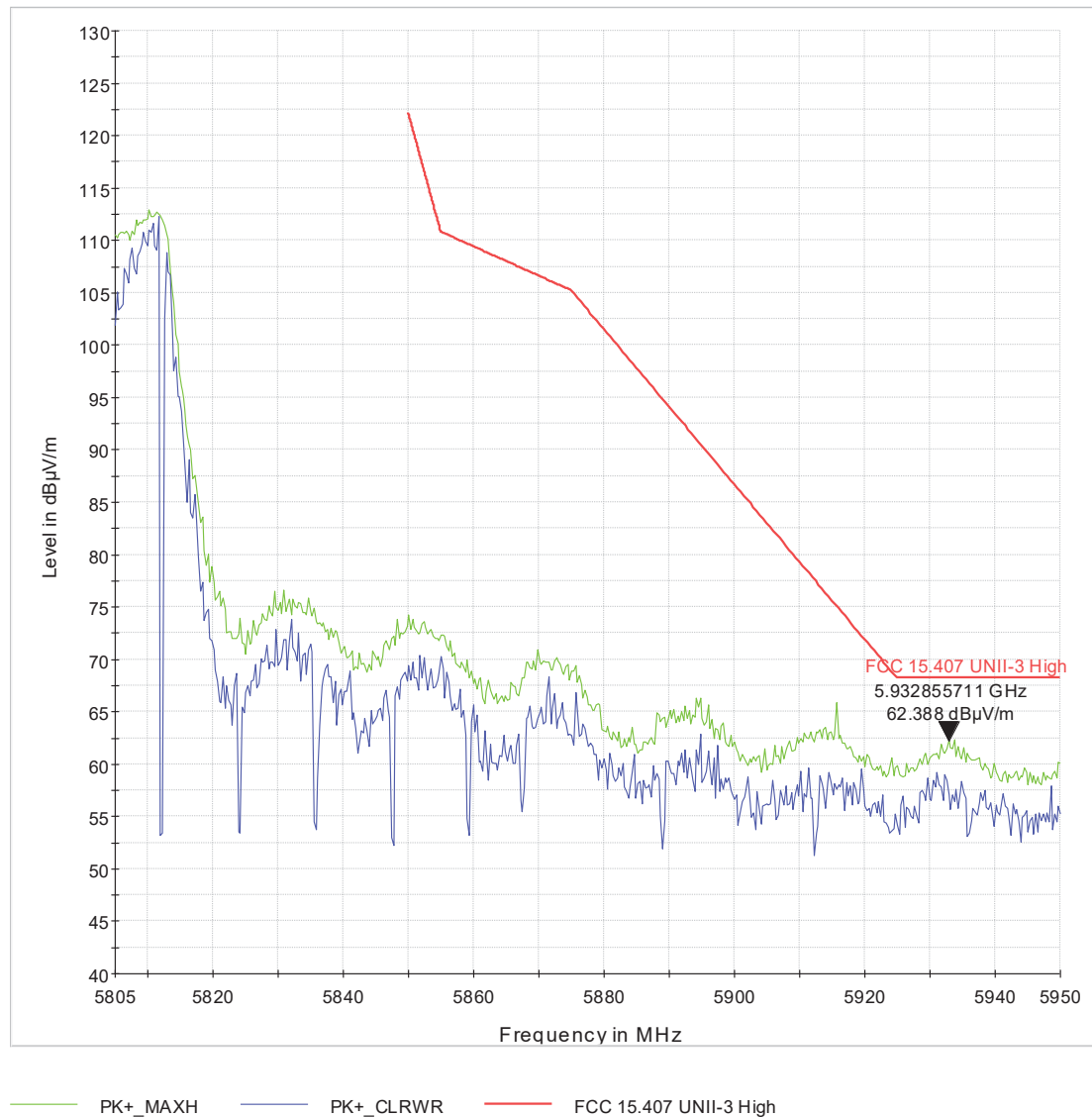
Figure 8 U-3_H-BE_ch155_VHT80_2x2_pwr=20.5_127deg_206cm_V
