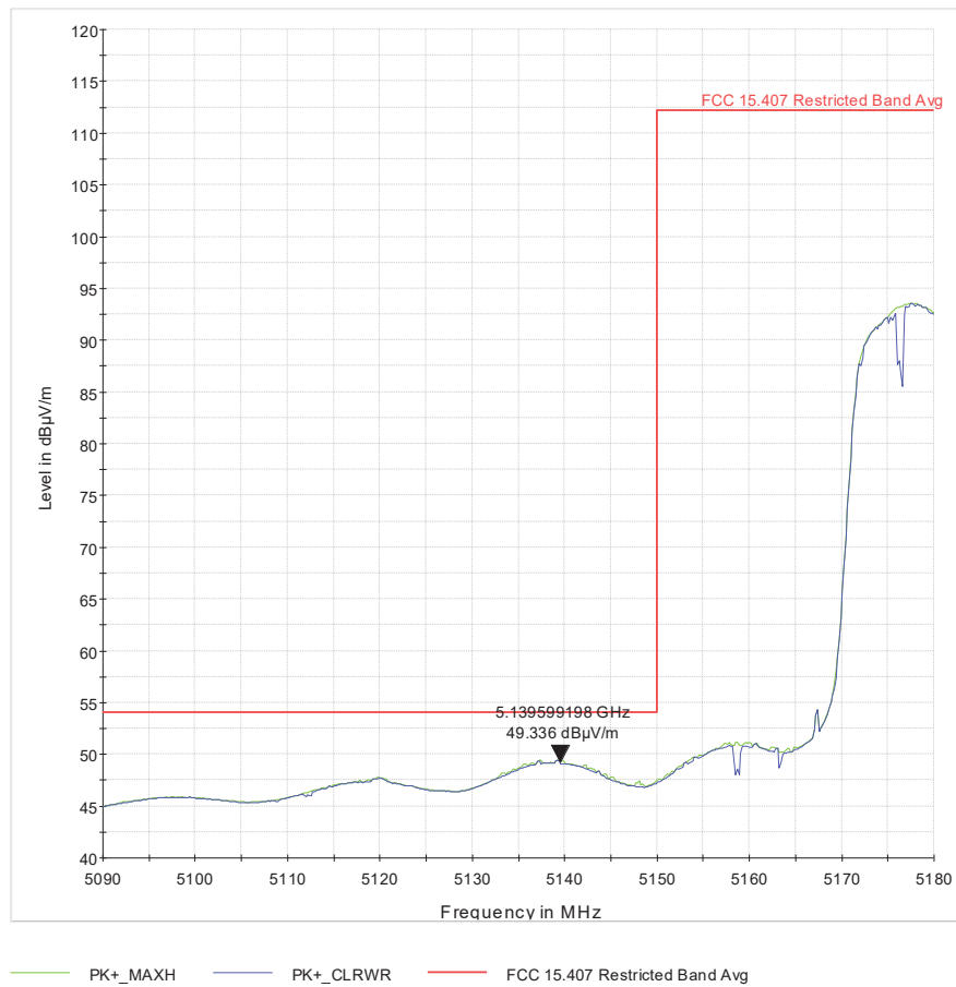
Figure 19 U-1_L-BE_ch42_VHT80_2x2_pwr=17_BF_228deg_178cm_H_avg
