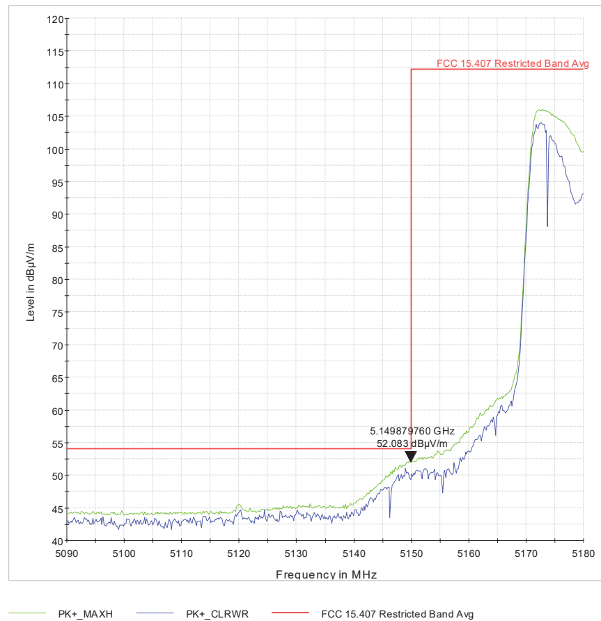
Figure 6 U-1_L-BE_ch36_HT20_2x2_pwr=20_maximize
