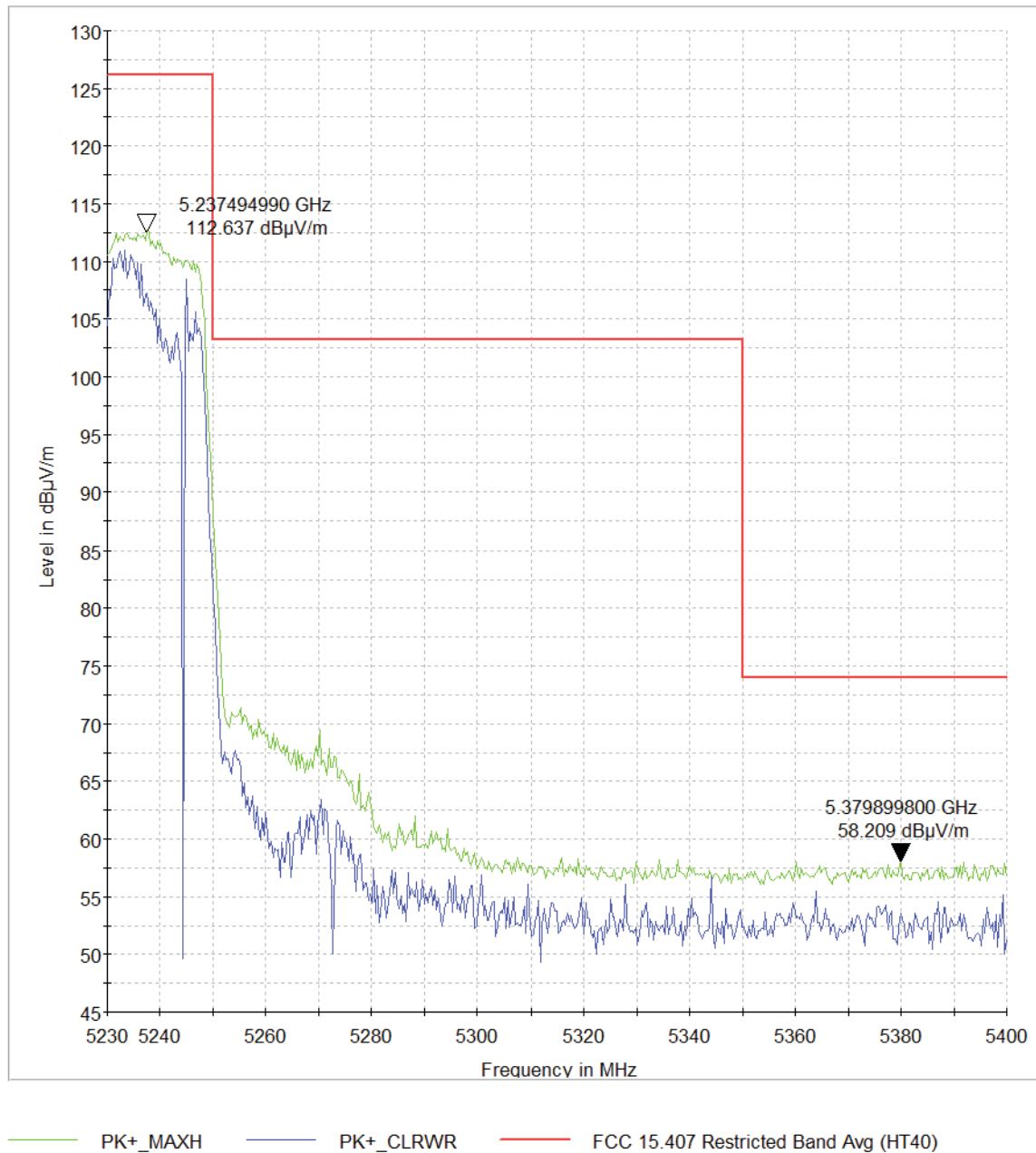
Figure 27 U-1_H_BE_HT40_ch46_pwr-17_2x2_CDD_234deg_150cm_V_pk
