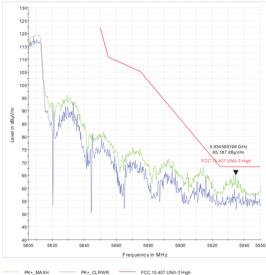
Figure 6 U-3_H-BE_ch159_HT40_2x2_pwr=24.5_130deg_208cm_V
