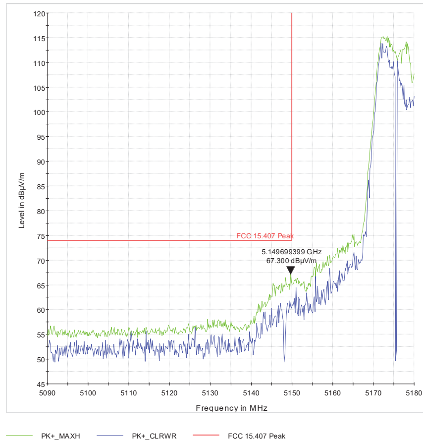
Figure 5 U-1_L-BE_ch36_HT20_2x2_pwr=20_241deg_168cm_H_pk
