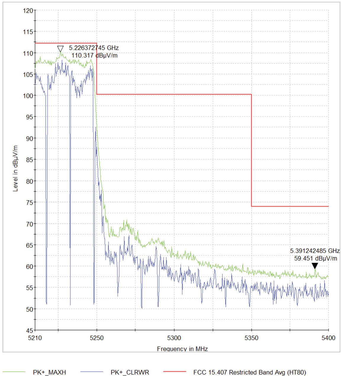
Figure 29 U-1_H_BE_VHT80_ch42_pwr-16.5_2x2_CDD_251deg_158cm_V_pk
