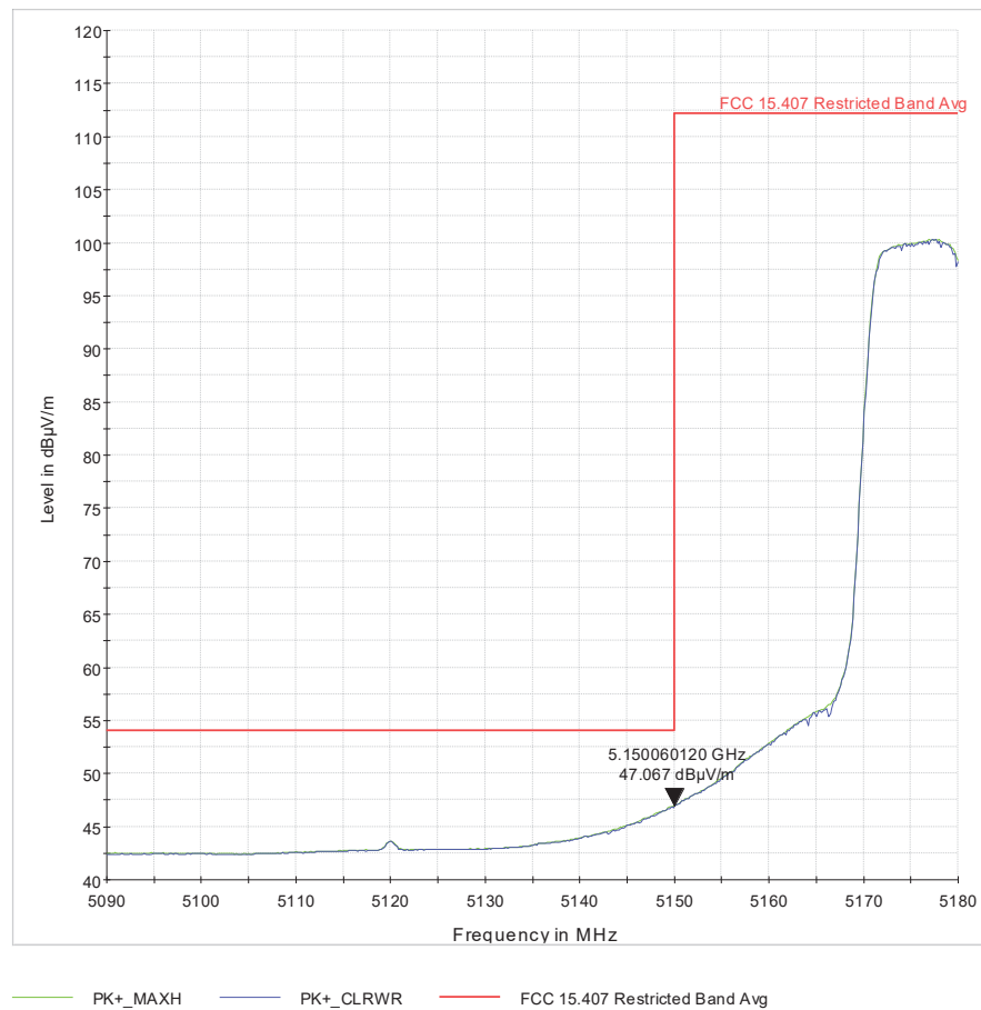
Figure 13 U-1_L-BE_ch36_VHT20_2x2_pwr=18_BF_218deg_209cm_H_avg
