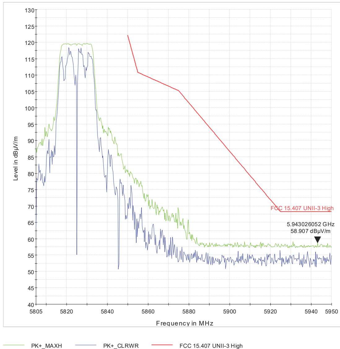
Figure 2 U-3_H-BE_ch165_NoHT_2x2_pwr=25_217deg_150cm_V
