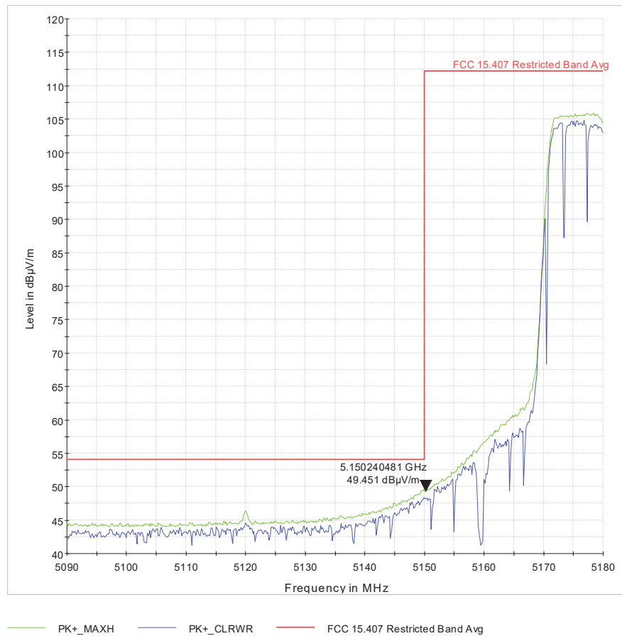
Figure 15 U-1_L-BE_ch36_VHT20_2x2_pwr=18_BF_maximize
