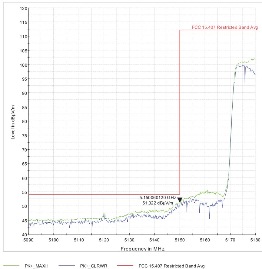
Figure 9 U-1_L-BE_ch38_HT40_2x2_pwr=17_maximize
