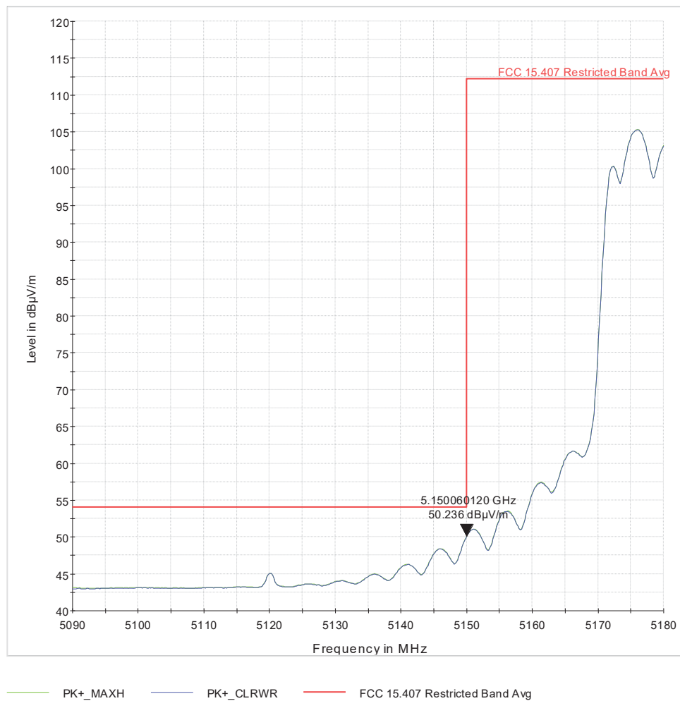
Figure 1 U-1_L-BE_ch36_NoHT_2x2_pwr=20.5_73deg_192cm_V_avg
