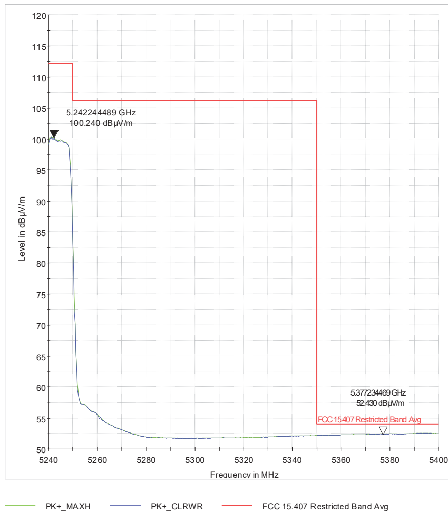
Figure 30 U-1_H_BE_VHT20_ch48_pwr-20_2x2_BF_262deg_123cm_V_avg
