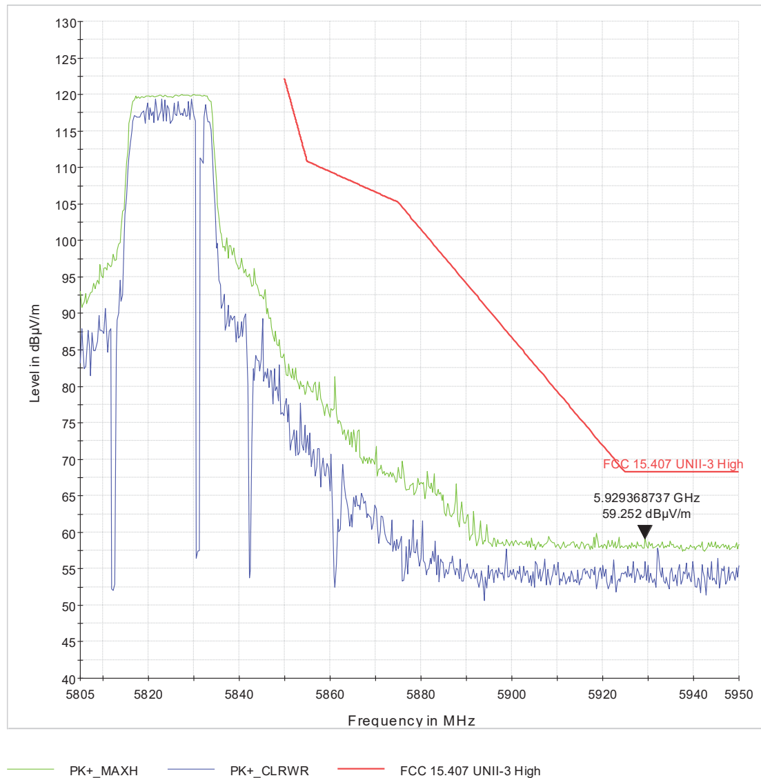
Figure 10 U-3_H-BE_ch165_VHT20_2x2_pwr=25_BF_135deg_159cm_V
