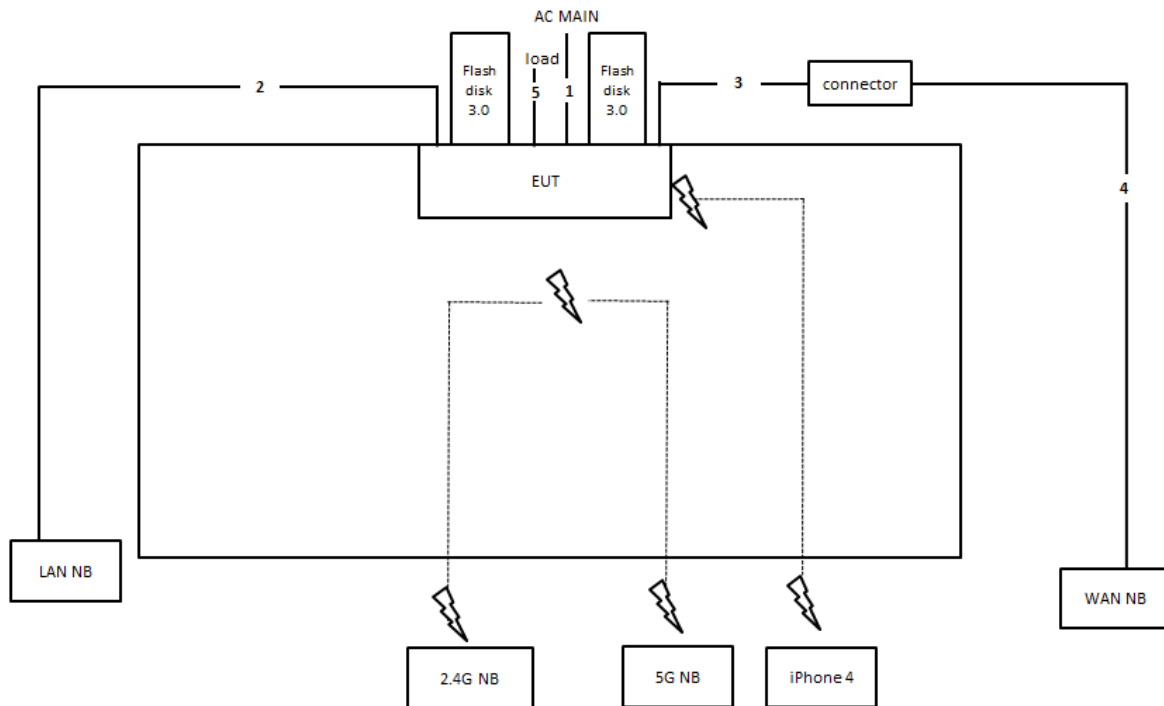
Test Setup Diagram - Radiated Test &lt; 1GHz
